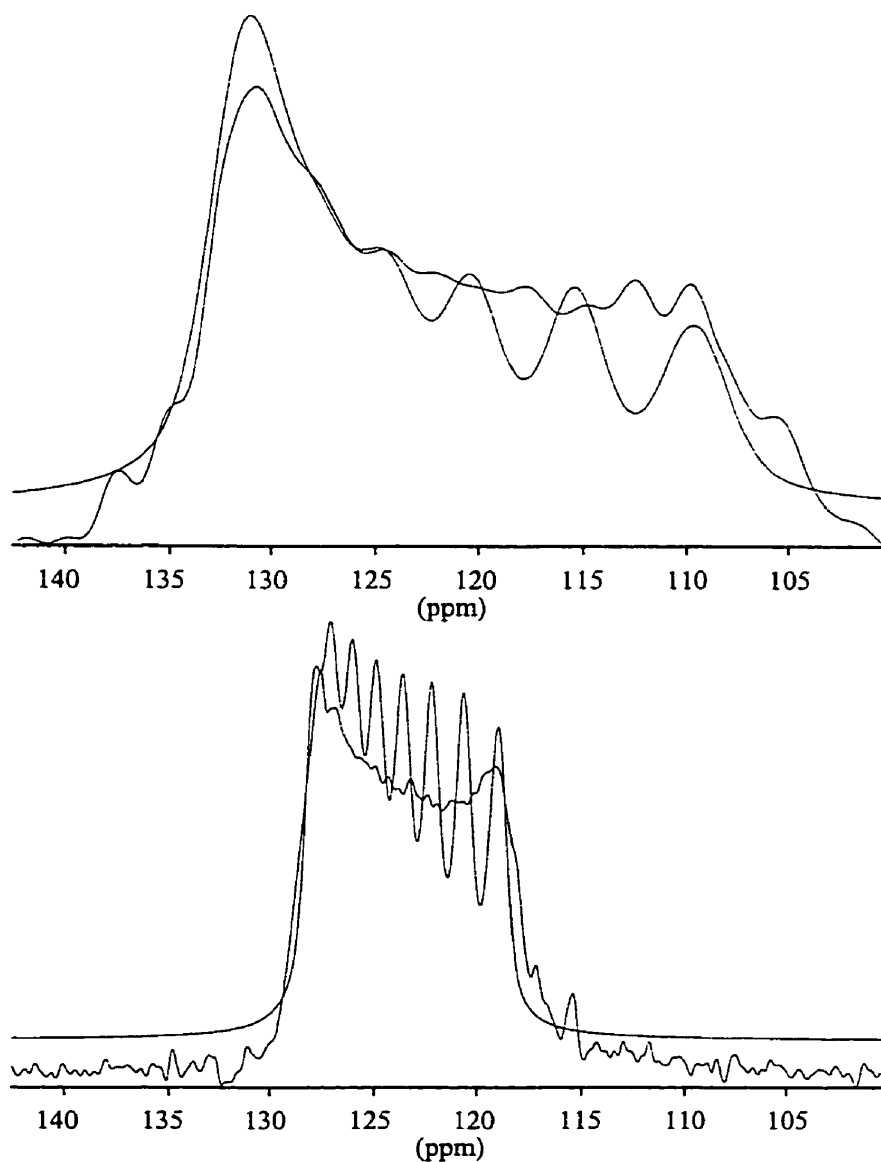
Figure 4.3: Solid-state ^{13}\text{C} NMR spectra of cyano- ^{13}\text{C}^{15}\text{N} -cobalamin at 4.7 T (upper) and 11.75 T (lower). Simulations using a \delta_{\text{iso}} = 123.5 ppm, R_{\text{eff}} = 600 Hz, J_{\text{CoC}} = 165 Hz, \alpha = 18^\circ , \beta = 165^\circ , \chi = 27.31 MHz, and \eta = 0.243 are offset slightly above experimental spectra.
