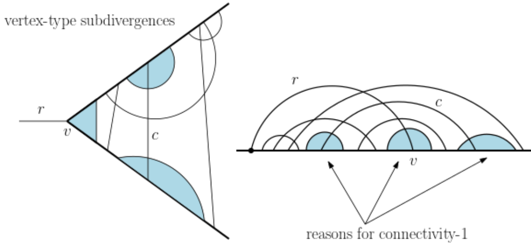
Figure 4.22: Connectivity-1 and vertex-type subdivergences.
