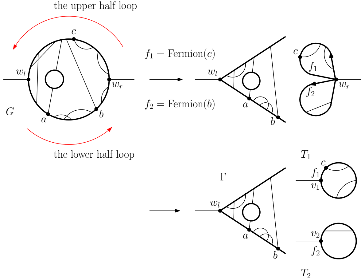
Figure 4.41: Calculating M^{-1}(G) .
