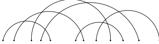
Figure 4.1: A diagram that is 3-connected but not 4-connected
