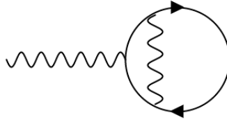
Figure 4.16: A tadpole diagram in QED
