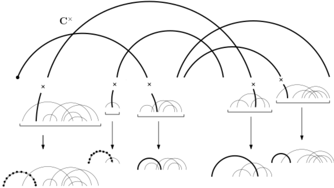
Figure 4.14: Maximal reasons obtained through the procedure (underlined), \mathbf{C}^\times (bold).
