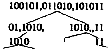
Figure 2.5: Tree Encoding
