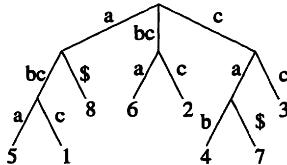
Figure 1.5: Suffix Tree
