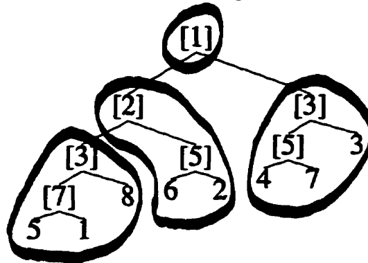
Figure 4.1: Tree Partition
