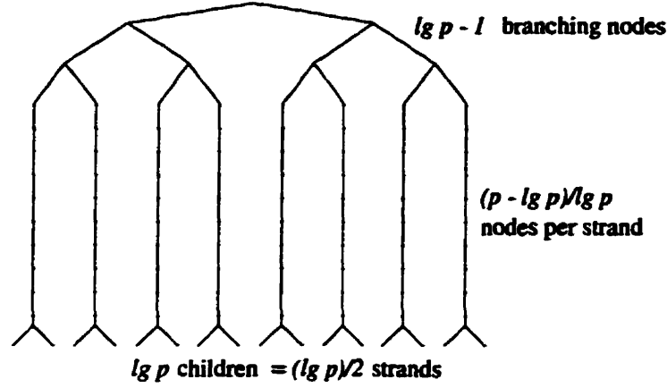
Figure 4.5: Node Cluster
