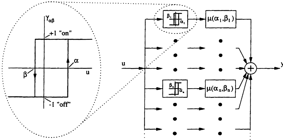
Figure 3.1: Schematic of the Preisach Model
