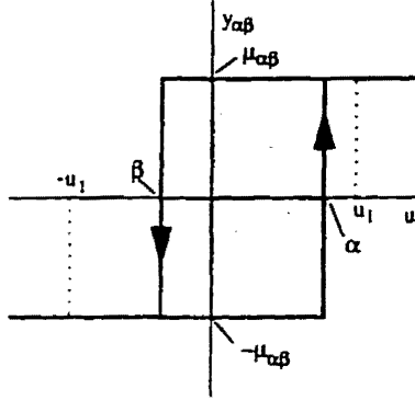
Figure 7.1: Weighted Relay
