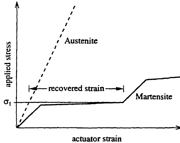
Figure 2.4: Stress-Strain Curves of Austenite and Martensite for SMA
