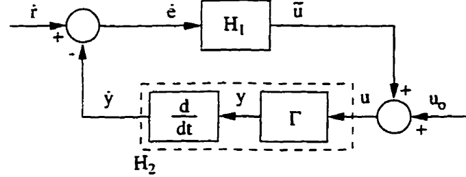
Figure 8.2: Velocity Feedback Configuration
