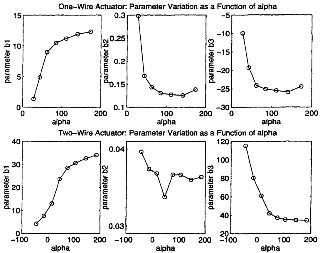
Figure 5.16: Parameter Variation
