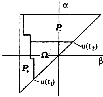
Figure 7.4: Proof of Theorem 7.2
