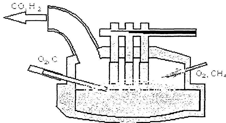
Figure 7.1: Schematic representation of a three phase EAF.
