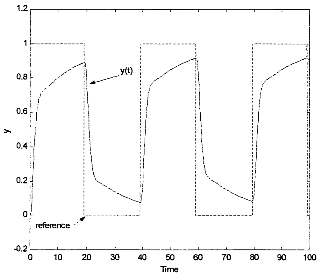
Figure 6.15: Predictive controller tracking for D_a=0.0576 .
