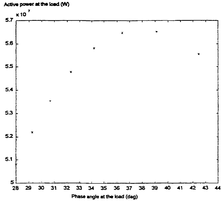
Figure 8.11: Active power at the load for THD = 1.
