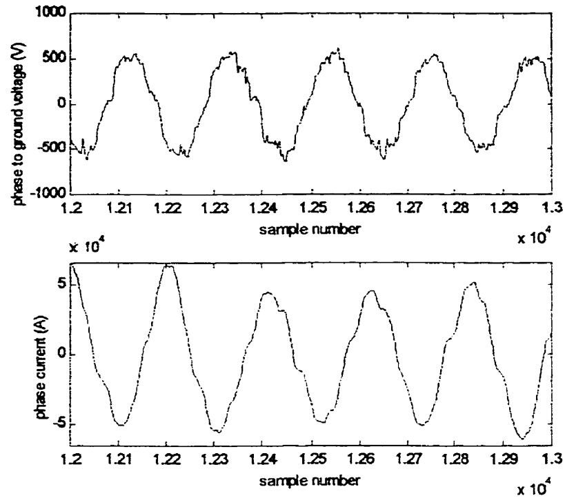
Figure 7.6: Voltage and current waves taken from a 58 MW, 3 phase EAF.
