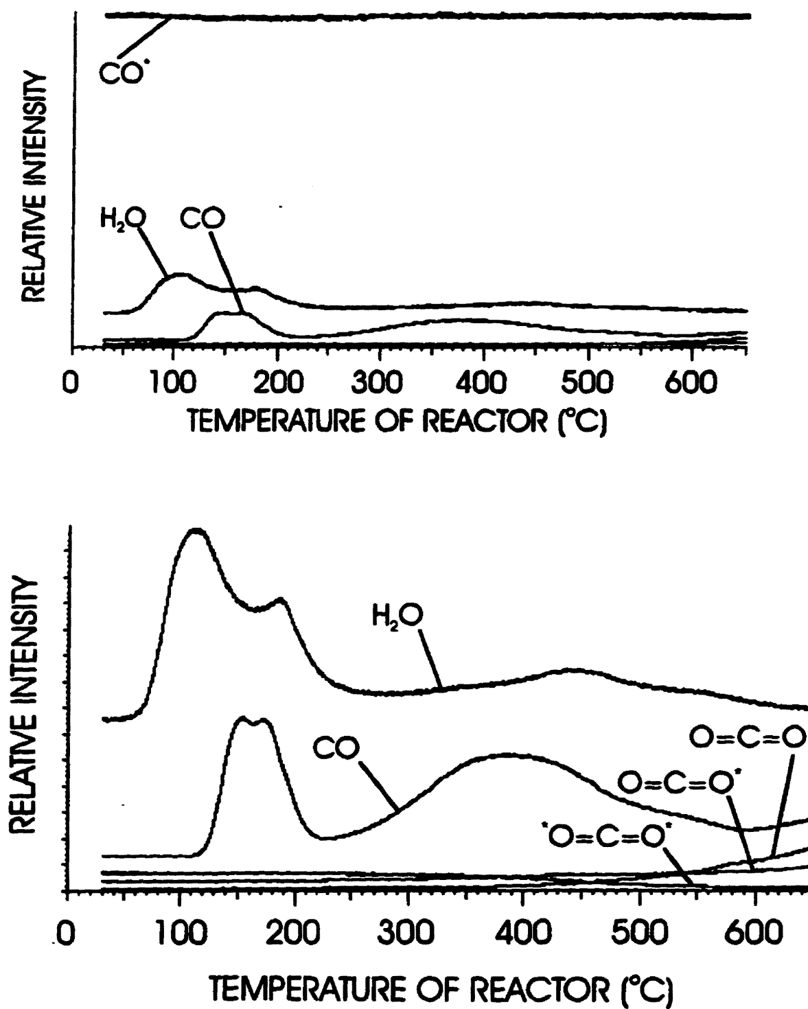
Fig.9.13A TPR of C^{18}O (8% C^{18}O/He and 15 mL/min) on 50 mg of 23.1%HPW/ SiO_2 . * = isotope 18.
