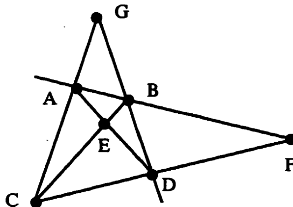
Figure 2.3: The Anti-Fano Configuration
