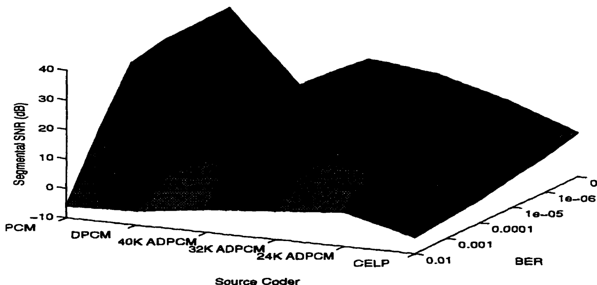
Figure 7.4: Objective Quality Measures under Stream Encryption
