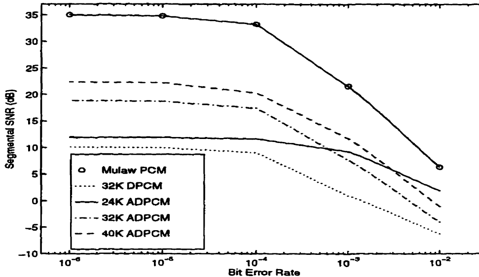
Figure 5.6: SegSNR Measures Under Gaussian Noise Conditions, \sigma_x^2 = \text{BER}
