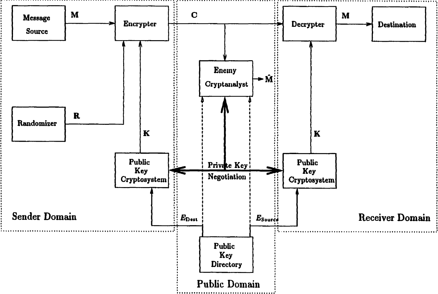
Figure 4.3: Use of Public Key to Exchange a Session Key
