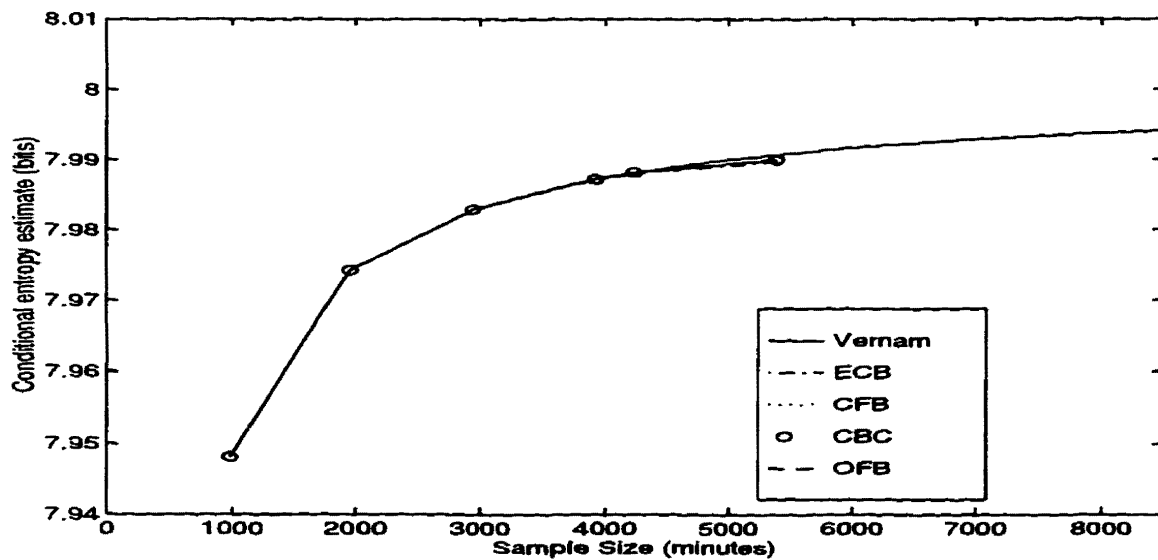
Figure N.2: Convergence Rate Comparison for Encrypted 32 kbps DPCM speech
