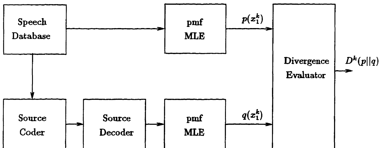
Figure 5.12: Block Diagram of Divergence Testing Methodology
