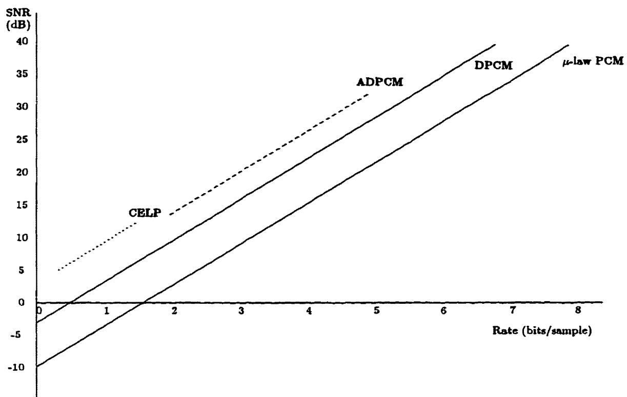
Figure H.1: SNR-Rate Performance of Representative Coders
