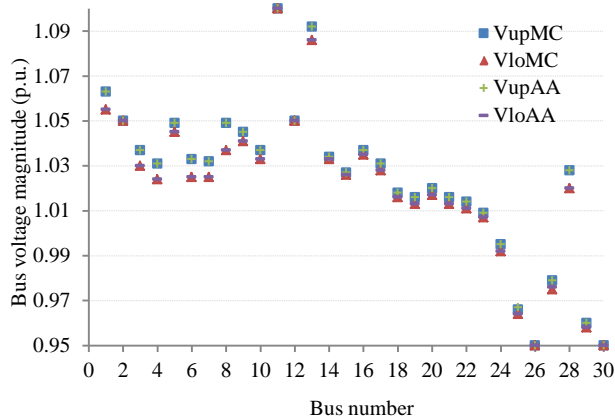
Fig. 2. Bus voltage magnitude intervals.
