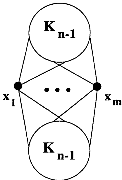
Figure 4.5: S_{m,m} .
