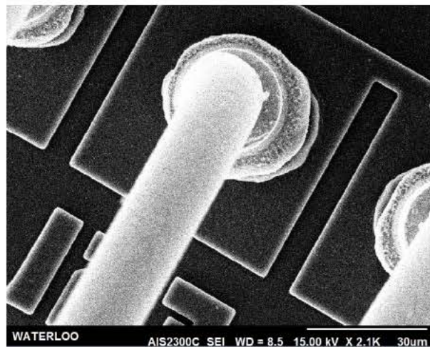
Figure 4. SEM image of a bonded ball using 18 \mu\text{m} PCS wire on Al metallization.
