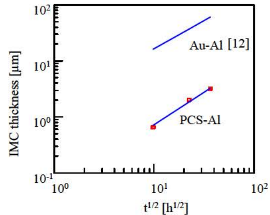
Figure 10. IMC thickness vs. square root of aging time t at 170 °C for Au-Al [12] and PCS-Al, respectively.
