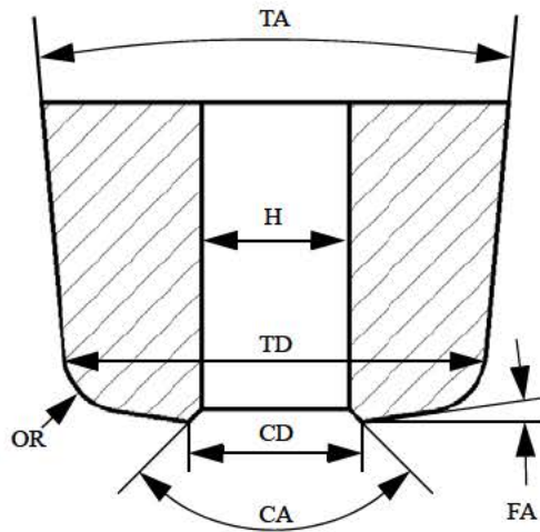
Figure 3. The illustration of a cross-section of the capillary used in this study, where TA = 10^\circ , H = 23 \mu\text{m} , TD = 66 \mu\text{m} , CD = 27 \mu\text{m} , CA = 90^\circ , OR = 10 \mu\text{m} , and FA = 8^\circ .
