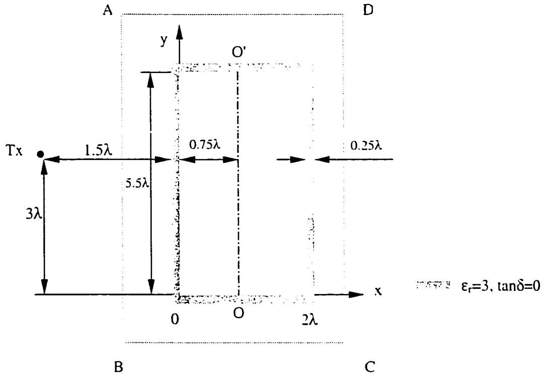
Fig. 3.6 2D lay out of a house with wooden walls and a transmitter located outside for studying penetration of wave from outdoor to indoor. The area of interest is enclosed by the virtual box ABCD.
