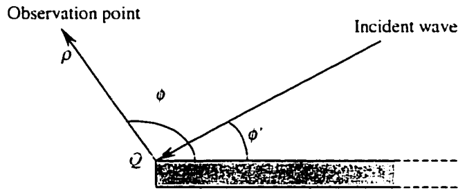
Fig. 2.4 Diffraction by thick lossy dielectric half plan (top view).
