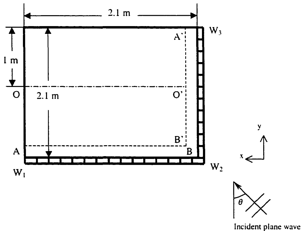
Fig. 4.12 Plane wave incidence on a building at 45°.
