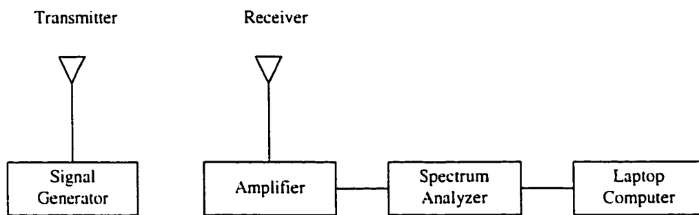
Fig. 2.12 Measurement system configuration.
