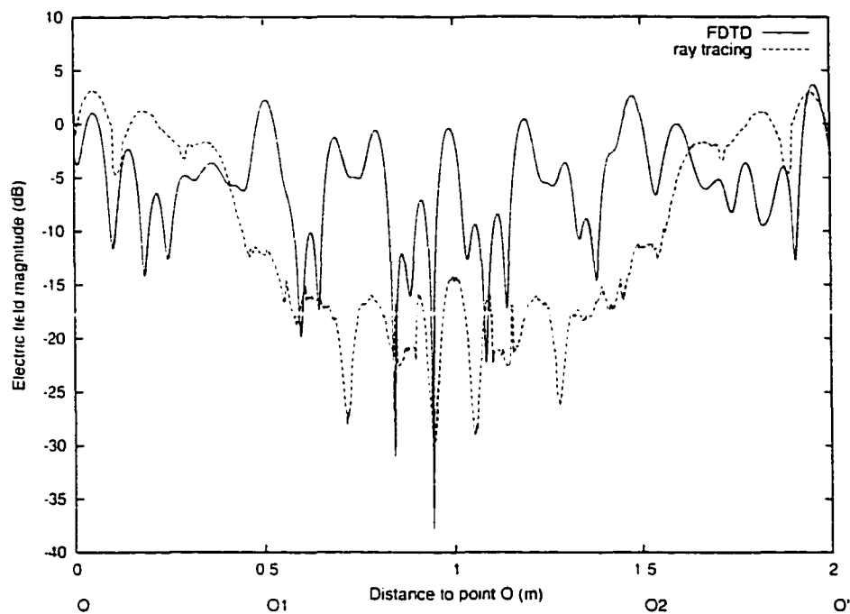
Fig. 4.8 Electric field distributions along OO' of Fig. 4.7 obtained by ray tracing and FDTD methods.
