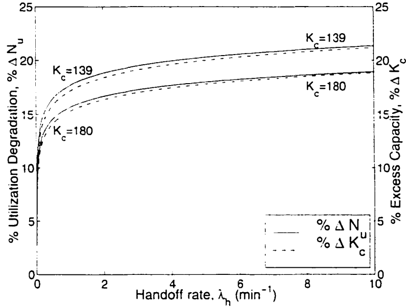
Figure 3.9: Percentage utilization degradation and excess capacity requirement as a function of mobility ( \mu^{-1} = 2 mins, P_f^* = 10^{-6} , P_n^* = 10^{-3} )
