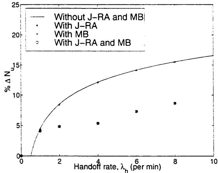
Figure 6.3: % utilization degradation as a function of mobility for RT service ( c = 1.5 Mbps, \mu^{-1} = 2 mins, P_n^* = P_f^* = 10^{-3} , \text{PLR}^* = 10^{-6} )
