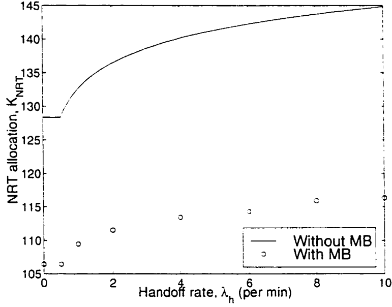
Figure 5.10: NRT capacity requirement as a function of mobility ( N_{uNRT} = 80 , r = 3 , P_n^* = P_f^* = 10^{-3} )
