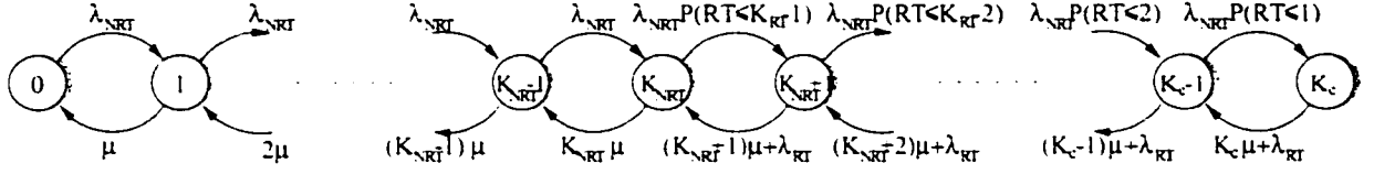
Figure 5.2: NRT Birth-Death Process
