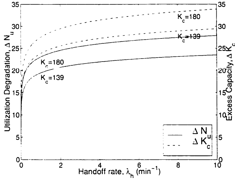
Figure 3.8: Utilization degradation and excess capacity requirement as a function of mobility ( \mu^{-1} = 2 mins, P_f^* = 10^{-6} , P_n^* = 10^{-3} )
