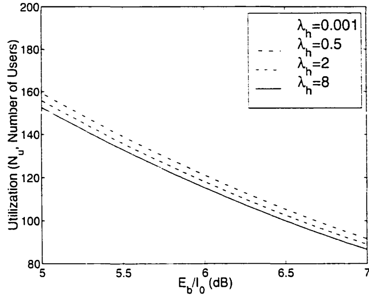
Figure 3.12: E_b/I_0 and capacity tradeoff ( K_c = 139 , \mu^{-1} = 2 mins, P_f^* = 10^{-6} , P_n^* = 10^{-3} )
