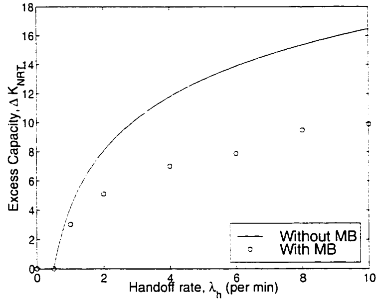
Figure 5.11: NRT excess capacity requirement as a function of mobility ( N_{u_{NRT}} = 80 , r = 3 , P_n^* = P_f^* = 10^{-3} )
