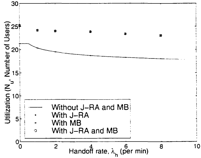
Figure 6.1: Utilization as a function of mobility for RT service ( c = 1.5 Mbps, \mu^{-1} = 2 mins, P_n^* = P_f^* = 10^{-3} , PLR^* = 10^{-6} )
