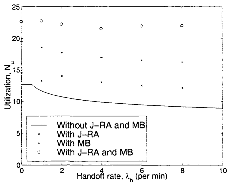
Figure 6.4: Utilization as a function of mobility for NRT service ( c = 1.5 Mbps, \mu^{-1} = 2 mins, P_n^* = P_f^* = 10^{-3} , \text{PLR}^* = 10^{-6} )
