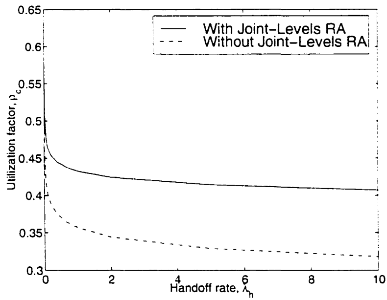
Figure 4.7: Call-level utilization factor in CDMA environment P_C^{(3)} ( \text{PLR}^* = 10^{-6} , P_n^* = 10^{-3} and P_f^* = 10^{-6} )
