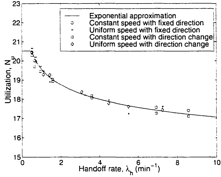
Figure 3.1: Accuracy of the exponential inter-handoff time assumption with K_c = 35
