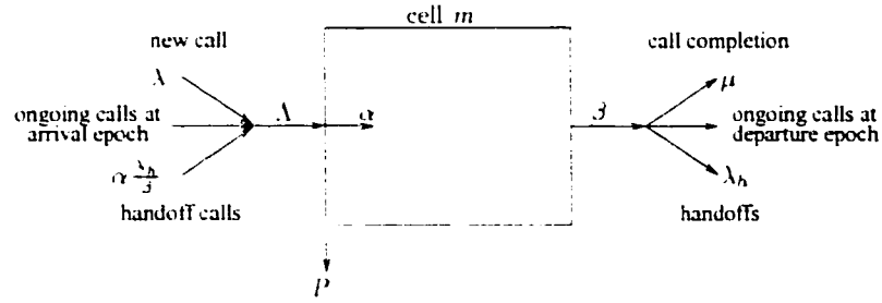
Figure 3.3: Queueing Model for Homogeneous Traffic
