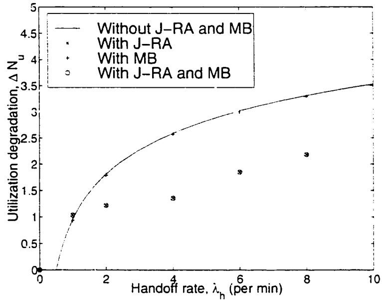
Figure 6.2: Utilization degradation as a function of mobility for RT service ( c = 1.5 Mbps, \mu^{-1} = 2 mins, P_n^* = P_f^* = 10^{-3} , \text{PLR}^* = 10^{-6} )
