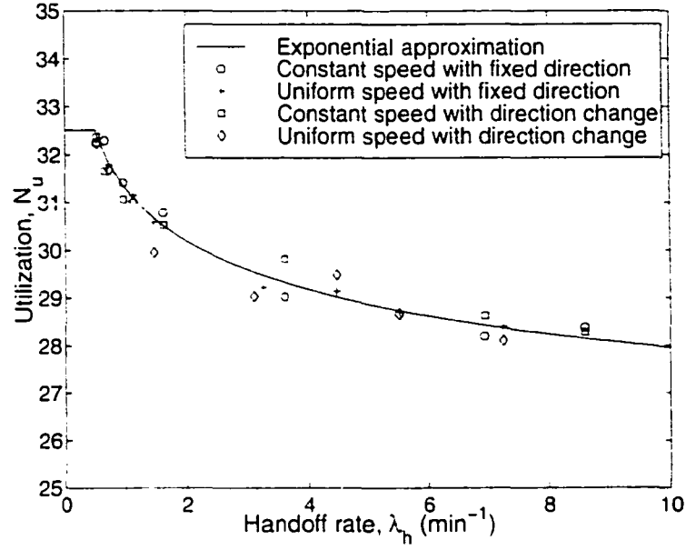
Figure 3.2: Accuracy of the exponential inter-handoff time assumption with K_c = 50
