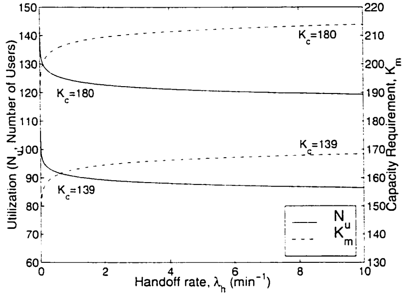
Figure 3.7: Utilization and capacity requirement as a function of mobility ( \mu^{-1} = 2 mins, P_f^* = 10^{-6} , P_a^* = 10^{-3} )
