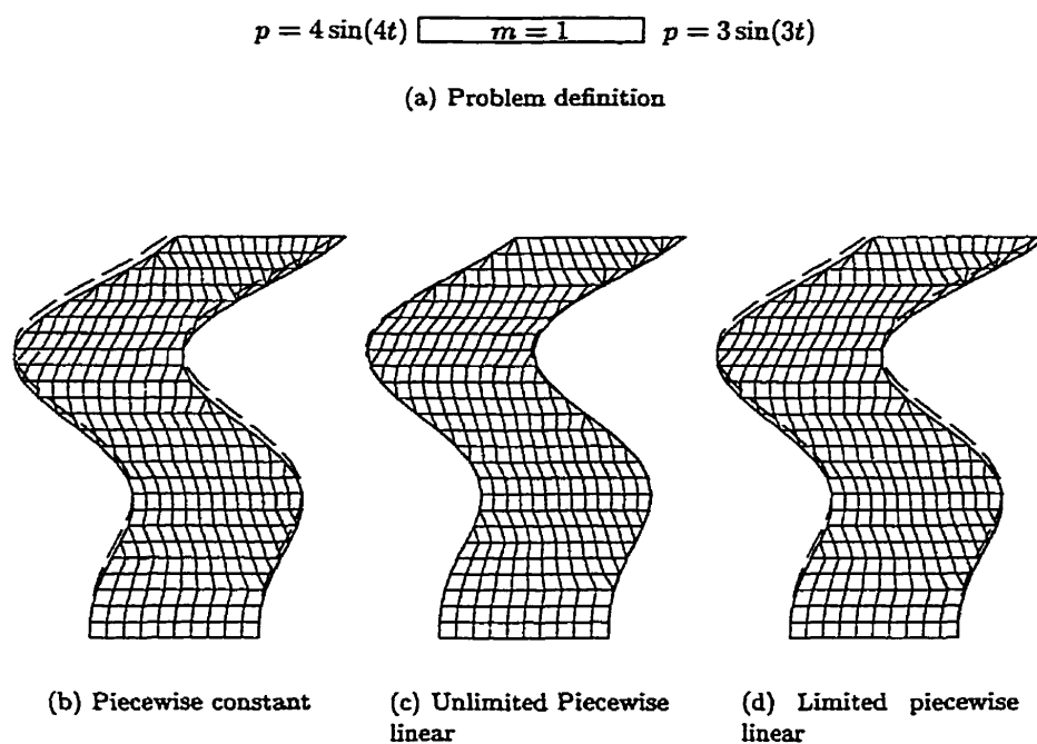
Figure 6.4: One-dimensional free boundary test case. The dashed line indicates the analytical boundary position.
