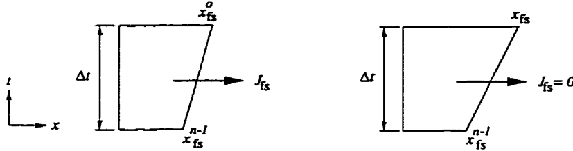
Figure 6.1: Application of kinematic condition for one-dimensional problems. Left: before; right: after.
