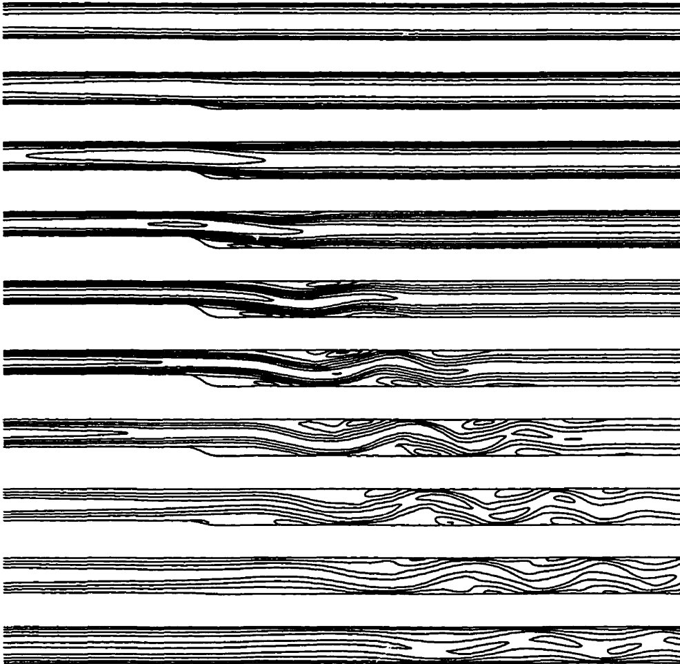
Figure 5.8: Contours of u -velocity for moving indentation test case on time planes t^* = 0.1, 0.2, \dots, 1.0 .
