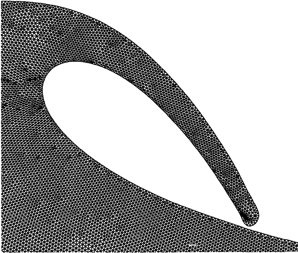
Figure 6.12: Close-up of the overturning wave at t = 51.75 .
