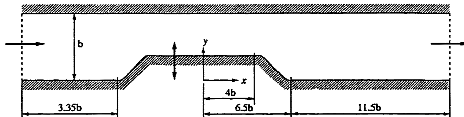
Figure 5.6: Geometry of moving indentation test case, with b = 1 .
