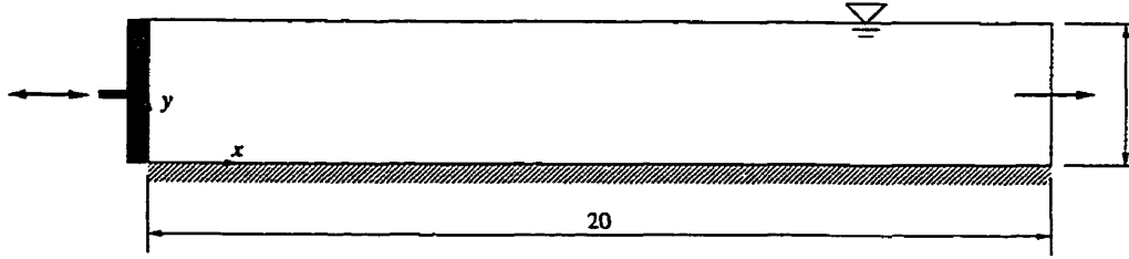
Figure 6.8: Wave channel geometry used in overturning wave test case.
