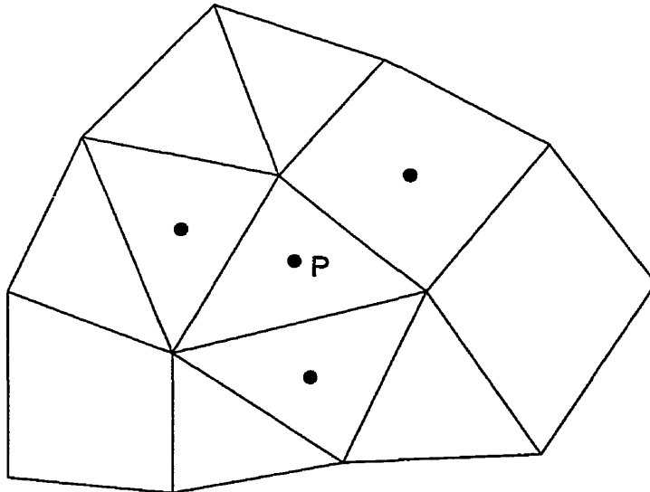
Figure 3.2: Least-squares stencil used in calculating cell gradient vectors.
