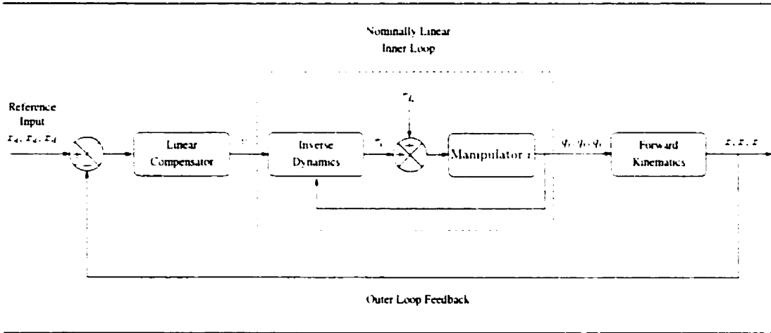
Figure 4.1: Decentralized Feedback Linearization Control of Manipulator i .
