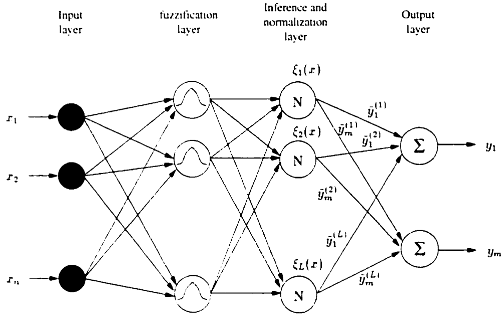
Figure 5.1: The Structure of an Adaptive MIMO FLC.
