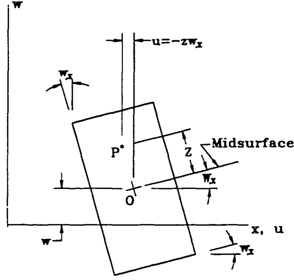
Figure 3.1: Kirchhoff plate element after loading.
