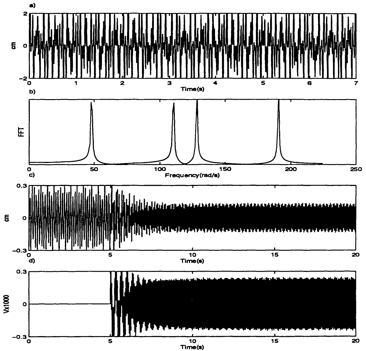
Figure 4.3: Oscillatory response of a simply supported plate to four harmonic inputs a)Disturbance b)FFT of the disturbance c)Plant response at (\frac{L_g}{2}, \frac{7L_g}{12}) using LQ d)Controller Input using LQ
