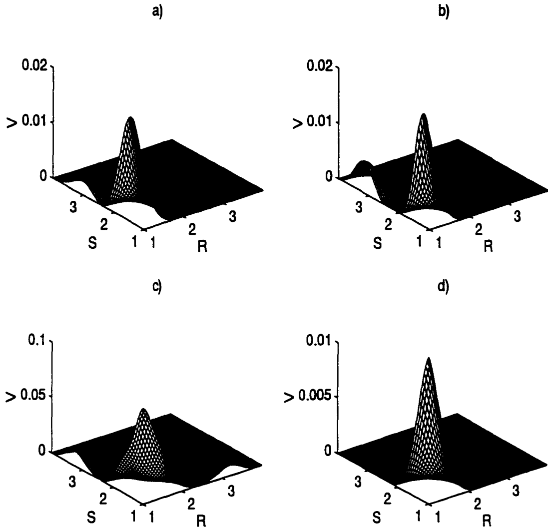
Figure 3.4: Contribution of inputs to the cost function at observation point (\frac{5L_x}{12}, \frac{5L_y}{12}) (a) Effect of piezo located at (\frac{L_x}{2}, \frac{L_y}{4}) (b) Effect of piezo located at (\frac{L_x}{2}, \frac{L_y}{2}) . (c) Effect of all piezos (d) Effect of external point load
