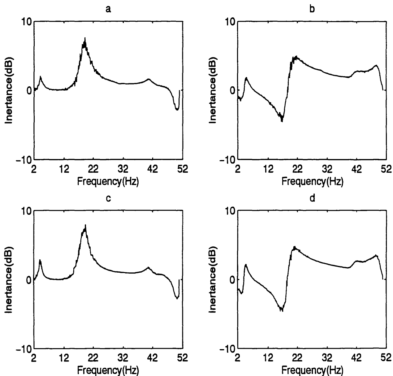
Figure 5.7: Frequency Response Function of Point (\frac{5L_a}{12}, \frac{5L_a}{12}) a)Magnitude b)Real, Frequency Response Function of Point (\frac{7L_a}{12}, \frac{5L_a}{12}) c)Magnitude d)Real.
