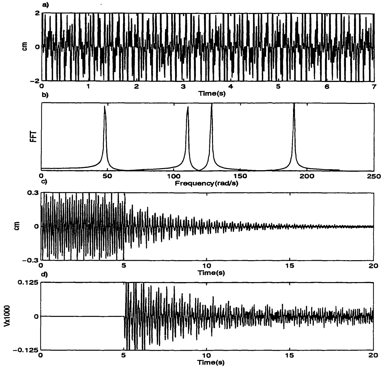
Figure 4.9: Oscillatory response of a simply supported plate to four harmonic inputs a)Disturbance b)FFT of the disturbance c)Plant response at (\frac{5L_n}{12}, \frac{7L_n}{12}) for \alpha_p = -1000, \alpha_c = 500 and optimal \xi_c d)Controller Input
