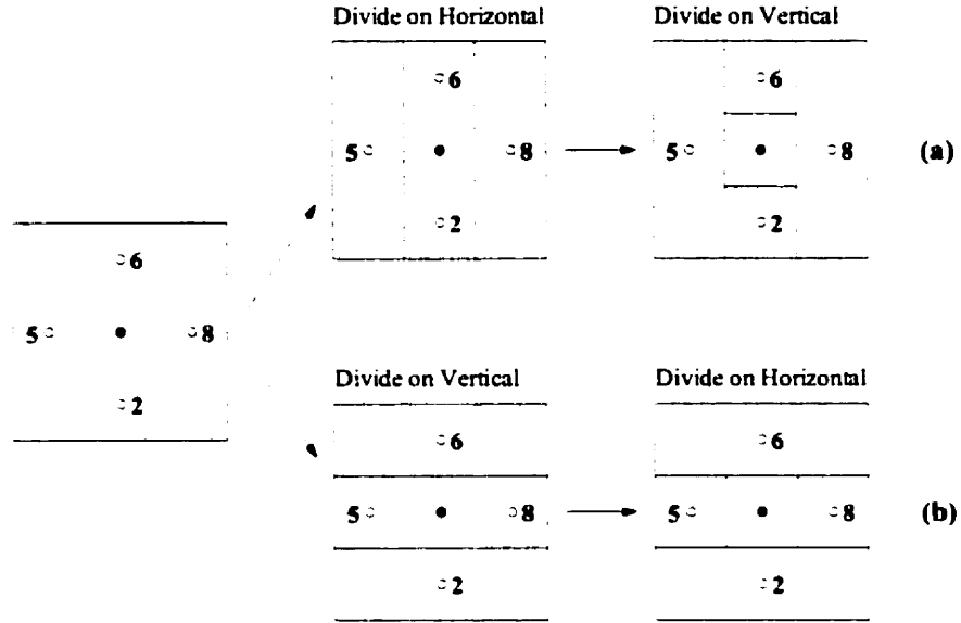
Figure 4.7: Dividing rectangles in the DIRECT algorithm.
