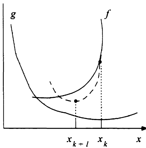
Figure 4.8: Newton's method for minimization.
