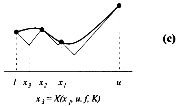
Figure 4.4: Shubert's algorithm
