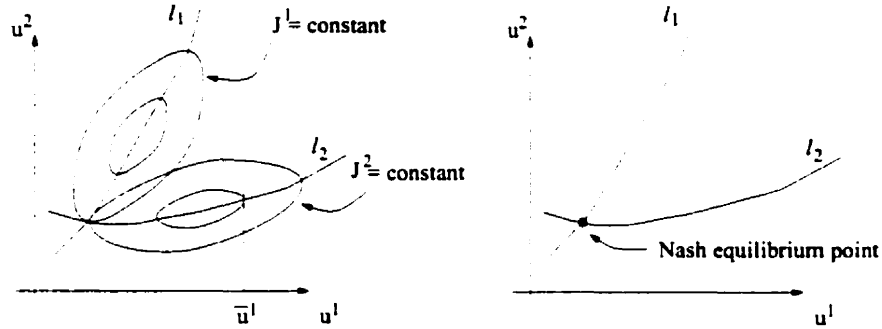
Figure 2.1: Iso-cost curves and the corresponding reaction curves for a two-player infinite game.
