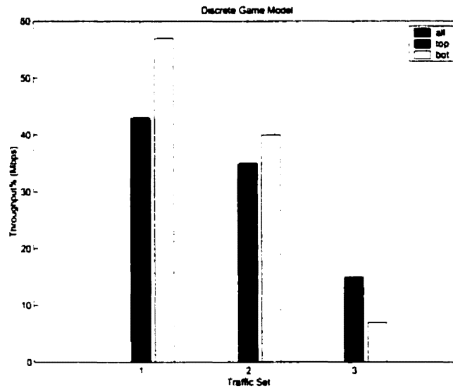
Figure 5.14: Throughput values for Net (3) (Equation 5.2)
