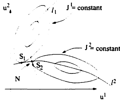
Figure 2.2: Nash and Stackelberg equilibria
