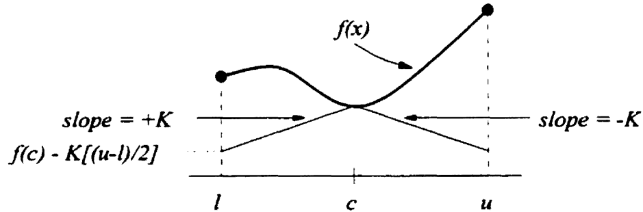
Figure 4.5: Computing a lower-bound with centerpoint sampling.
