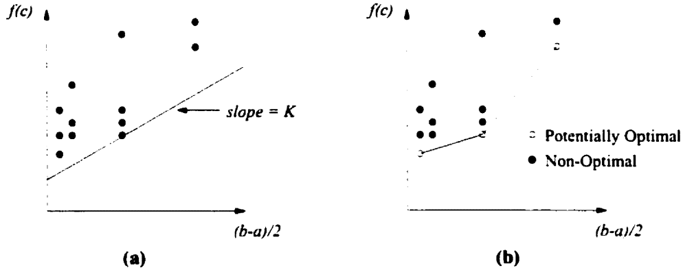
Figure 4.6: Set of potentially optimal intervals.
