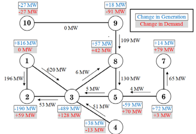
Fig. 8. Transmission line flows, generation and demand changes 2010-2018.
