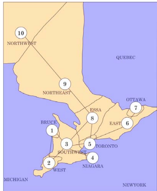
Fig. 3. Ontario 10-zone power system model.
