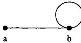
Figure 5.1: Underlying graph of Murskii's groupoid
