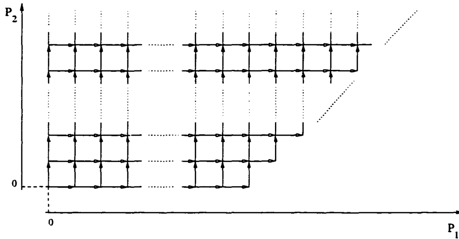
Figure 4.1: Computation structure
