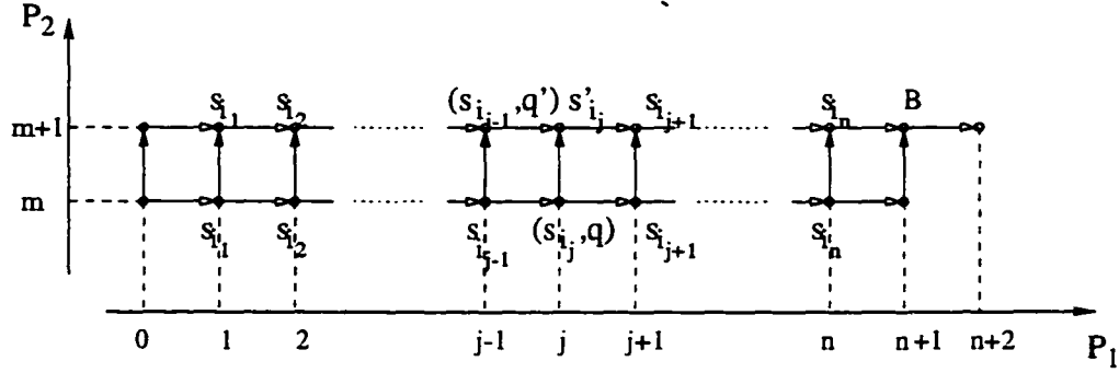
Figure 4.2: Two consecutive lines of a computation structure
