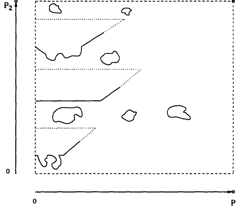
Figure 4.4: Finitely generated structure in \mathcal{K}
