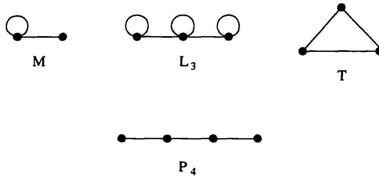
Figure 6.1: Prohibited subgraphs
