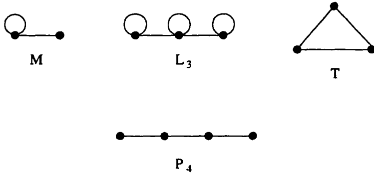
Figure 5.2: Prohibited subgraphs
