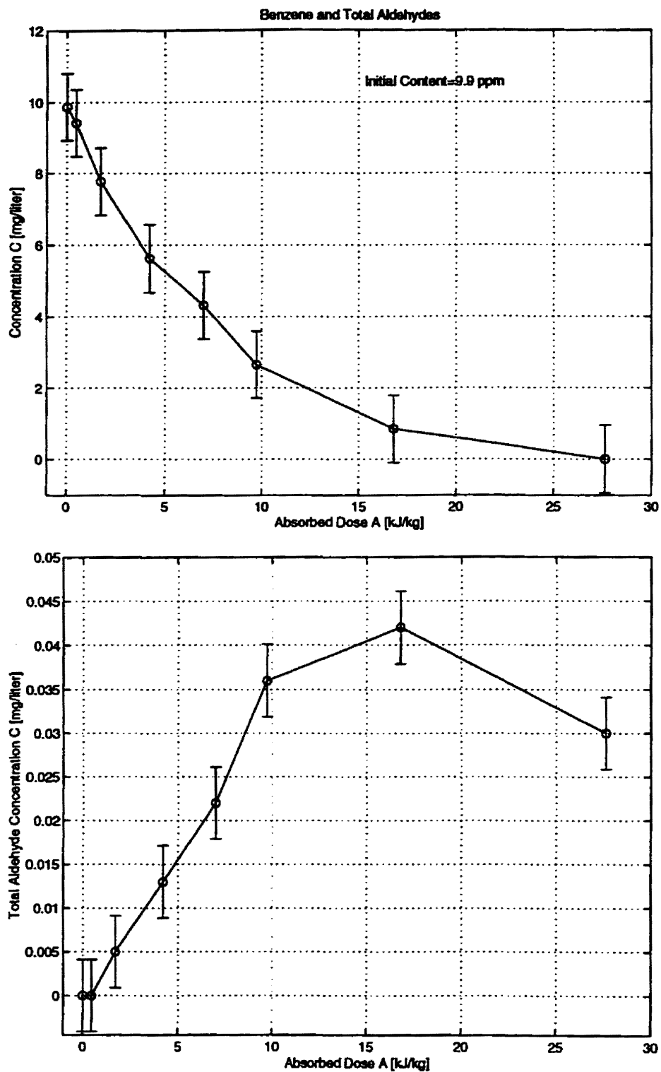
Figure 5.12. The dependence of the concentrations of benzene and total aldehydes on the estimated absorbed dose of electron beam radiation.
