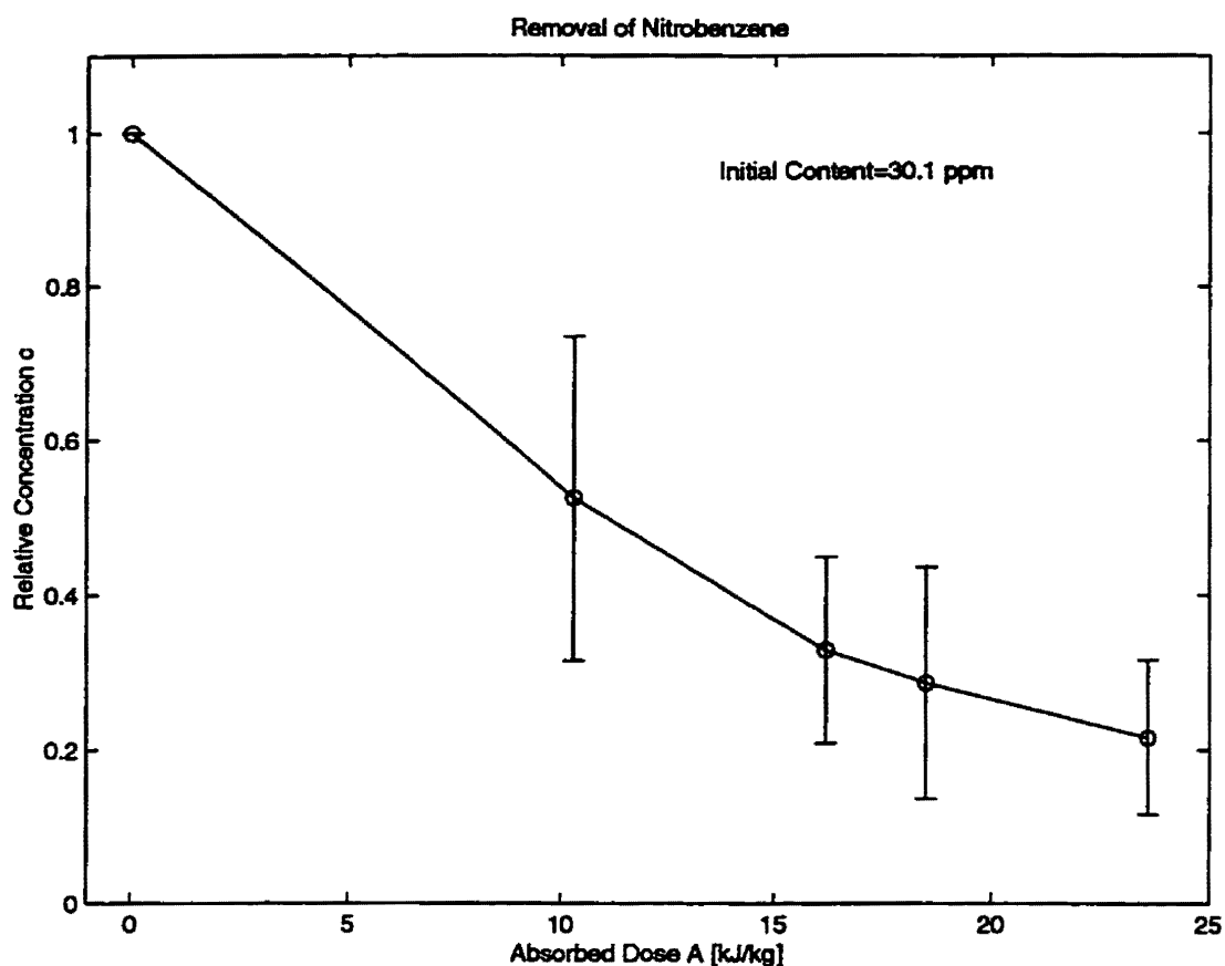
Figure 6.1. The dependence of the relative concentration of nitrobenzene vs. the estimated absorbed dose for 10 \mu\text{m} thick BN window and incident beam power P=40 W (accelerating voltage V_A=100 kV and electron beam current I_B=0.4 mA).
