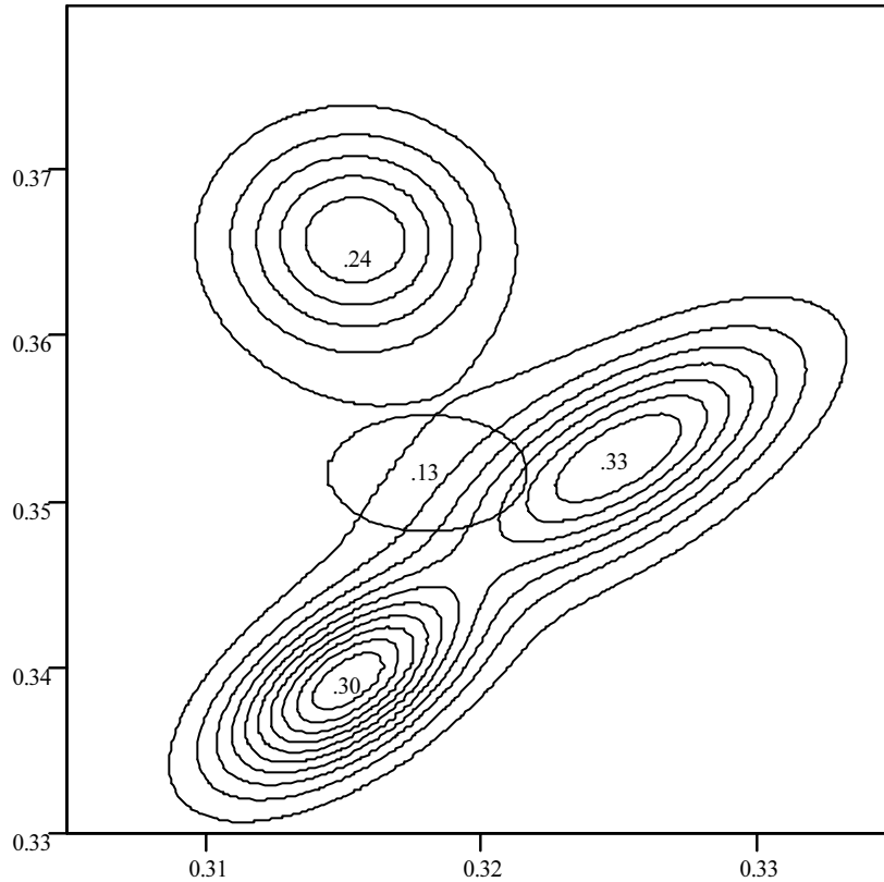
Figure 3.3.3 Contour plot for a Mixture Model of P(\bar{\mathbf{x}}) , where the central ellipse illustrates P(\bar{\mathbf{x}} | k = 4)
