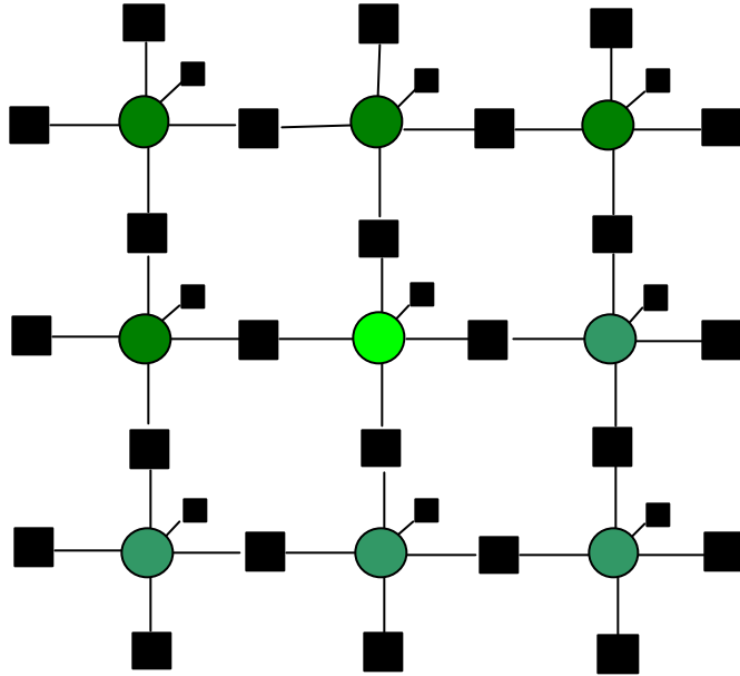
Figure 4.4.4 A factor graph a MRF model for an image (substructure is removed for clarity).
