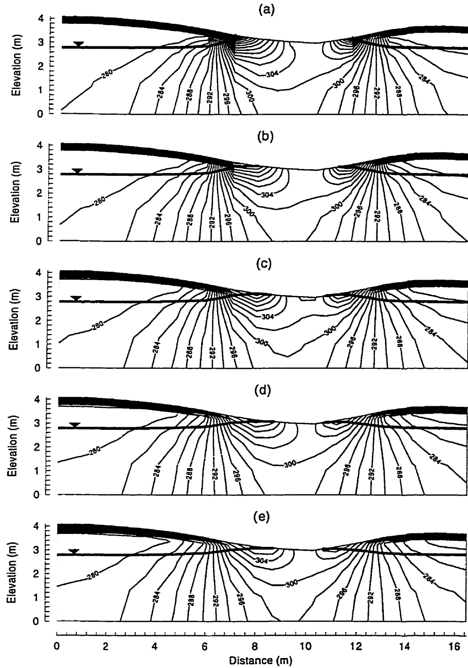
Figure 5-19. Total head and water table elevation along a representative cross section ( x = 40 m) at 50 minutes for first-order-coupled simulations. Solutions for initial hydraulic head of 278 cm and porous medium hydraulic conductivity equal to (a) 1 \times 10^{-5} \text{ m s}^{-1} (base case), (b) 2 \times 10^{-5} \text{ m s}^{-1} , (c) 3 \times 10^{-5} \text{ m s}^{-1} , (d) 4 \times 10^{-5} \text{ m s}^{-1} and (e) 5 \times 10^{-5} \text{ m s}^{-1} .
