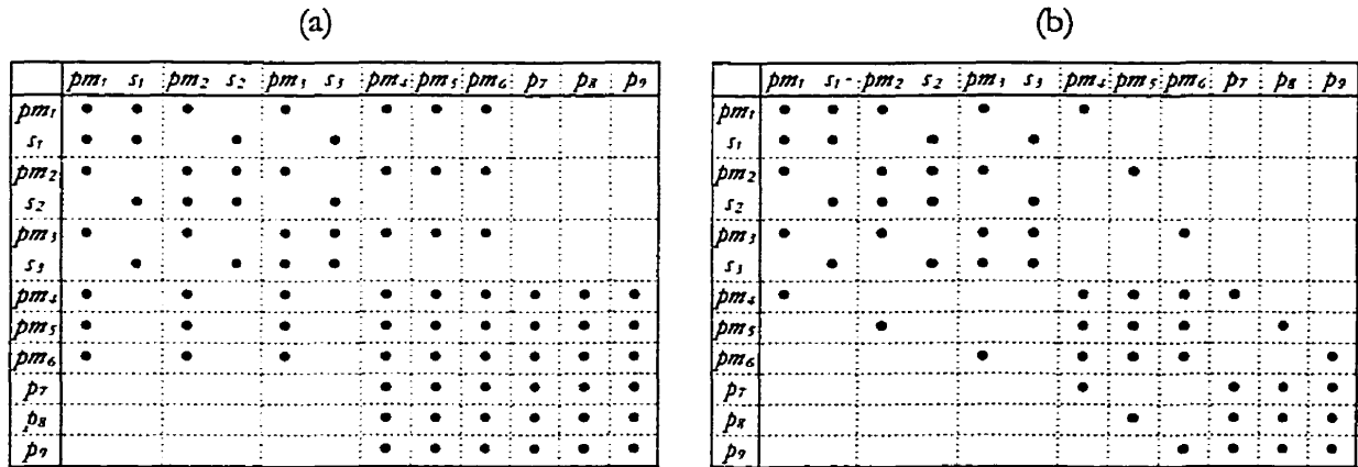
Figure 3-4. Jacobian structure for illustrative finite element mesh (Figure 3-2) assuming continuity of porous medium and macropore solutions: (a) connectivity arising from prism finite elements (78 entries) and (b) connectivity resulting from modified prisms (54 entries).
