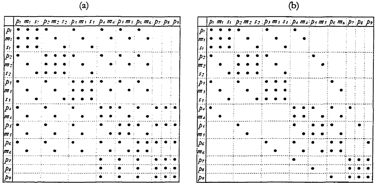
Figure 3-3. Jacobian structure for illustrative finite element mesh (Figure 3-2): (a) connectivity arising from prism finite elements (132 entries) and (b) connectivity resulting from modified prisms (95 entries).
