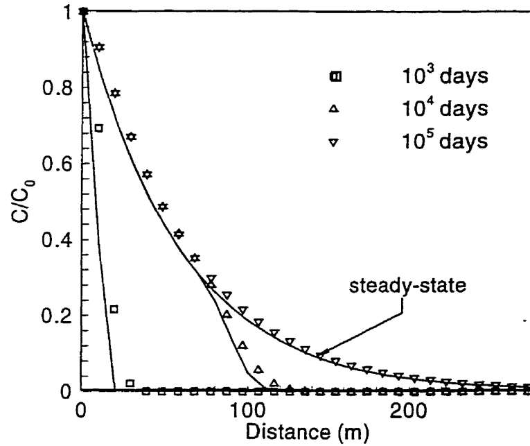
Figure 4-2. Concentration versus distance for parallel fracture transport verification problem [Sudicky and Frind, 1982 ]. Solid lines and symbols represent concentrations predicted by the analytical and numerical models, respectively.
