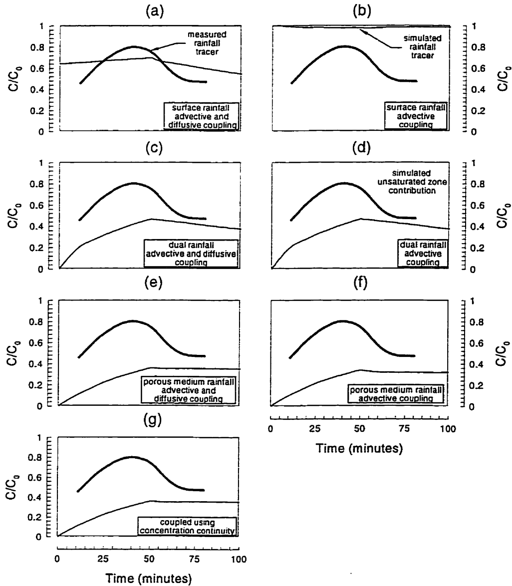
Figure 5-17. Comparison of measured and simulated rainfall tracer concentrations ( C_i ) in stream discharge water. Results for first-order-coupled simulations with rainfall applied to surface equations and (a) advective and diffusive coupling and (b) advective coupling only; rainfall applied to both the porous medium and surface equations using the dual rainfall algorithm with (c) advective and diffusive coupling and (d) advective coupling only; rainfall applied to porous medium equations with (e) advective and diffusive coupling and (f) advective coupling only; and (g) concentrations resulting from assuming continuity between the surface water and porous medium.
