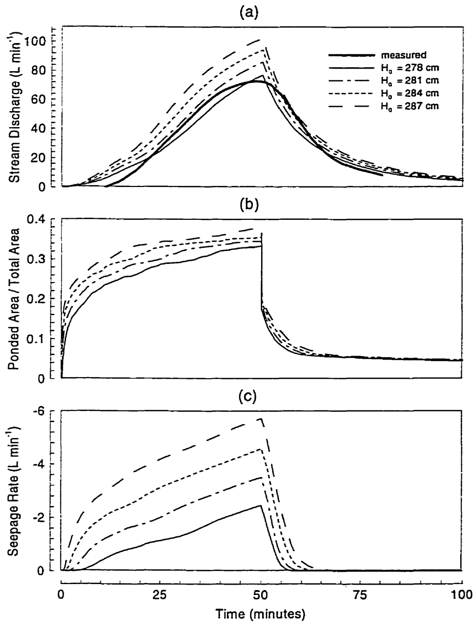
Figure 5-22. Illustration of rainfall-runoff sensitivity to initial water table elevation: (a) stream discharge, (b) relative contributing area, and (c) groundwater seepage. Solutions for porous medium hydraulic conductivity equal to 1 \times 10^{-5} \text{ m/s} .
