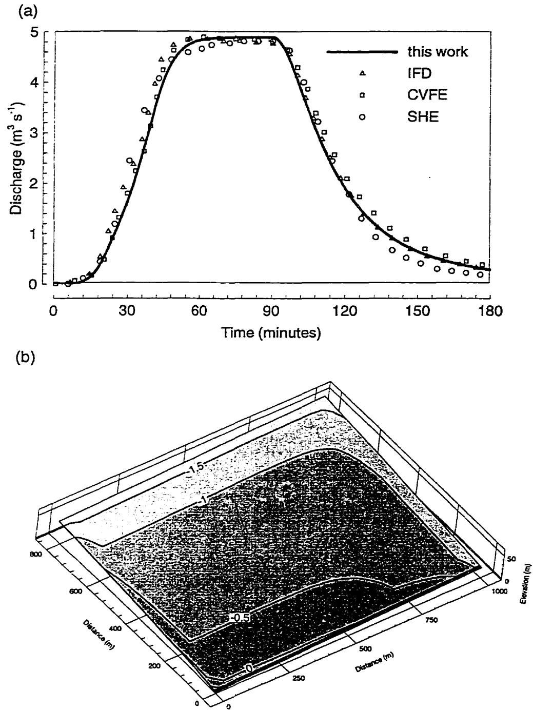
Figure 4-10. Evaluation of surface flow solution for tilted V-catchment verification problem: (a) comparison of simulated discharge with discharges presented by di Giammarco et al. [1996] for an integrated finite difference (IFD) model, a control volume finite element model (CVFE) and the SHE surface flow module, and (b) simulated water depths ( \log_{10}(\text{cm}) ) at ninety minutes (peak discharge) using the surface flow module developed in this work.
