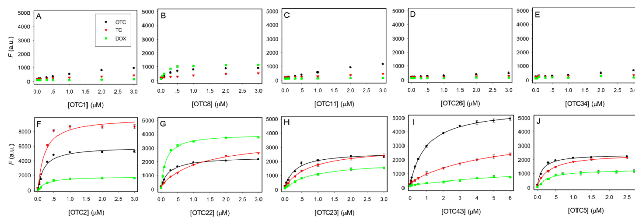
Figure 3. The aptamer-dependent fluorescence enhancement of the three tetracyclines (100 nM each) with the (A) OTC1, (B) OTC8, (C) OTC11, (D) OTC26, (E) OTC34, (F) OTC2, (G) OTC22, (H) OTC23, (I) OTC43 and (J) OTC5 aptamers. The buffer was pH 6.0 10 mM MES with 2 mM Mg^{2+} .
