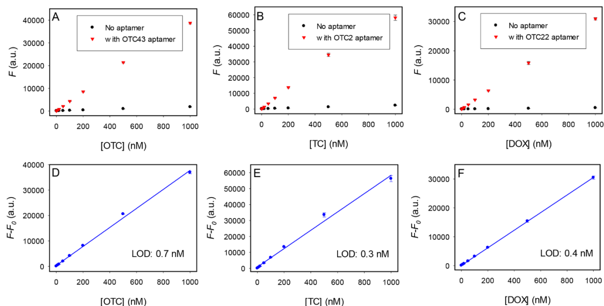
Figure 4. The fluorescence of different concentrations of (A) free OTC and after adding 2 \mu\text{M} OTC43 aptamer, (B) free TC and after adding 2 \mu\text{M} OTC2 aptamer, and (C) free DOX and after adding 2 \mu\text{M} OTC22 aptamer. The fluorescence intensity difference before and after adding the aptamers for the detection of (D) OTC, (E) TC, and (F) DOX using the aptamers in panels (A-C).
