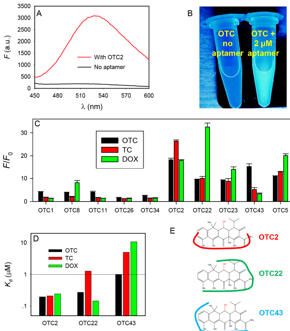
Figure 2. (A) Fluorescence spectra of 100 nM OTC before and after adding 2 μM OTC2 aptamer. (B) A fluorescent photograph of 500 nM OTC with (right) and without (left) 2 μM OTC2 aptamer. (C) The fold of fluorescence enhancement of the ten aptamers to the three tetracyclines. (D) The K_d values of the three aptamers. Note the y-axis is in log scale. (E) Structures showing aptamers binding to OTC in three different ways, which can explain their selectivity for the three tetracycline antibiotics.
