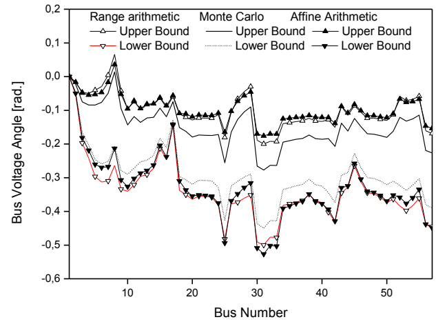
Fig. 3: Computed bus voltage angle intervals.
