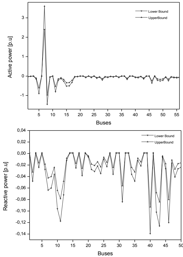
Fig. 1. Assumed active and reactive power input variations.
