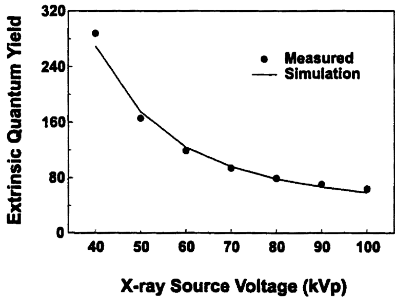
Figure 5.13: Response of detector for various X-ray source voltages (kVp) normalized to the number of incoming photons, collected over a period of 500 ms and 25 mAs .
