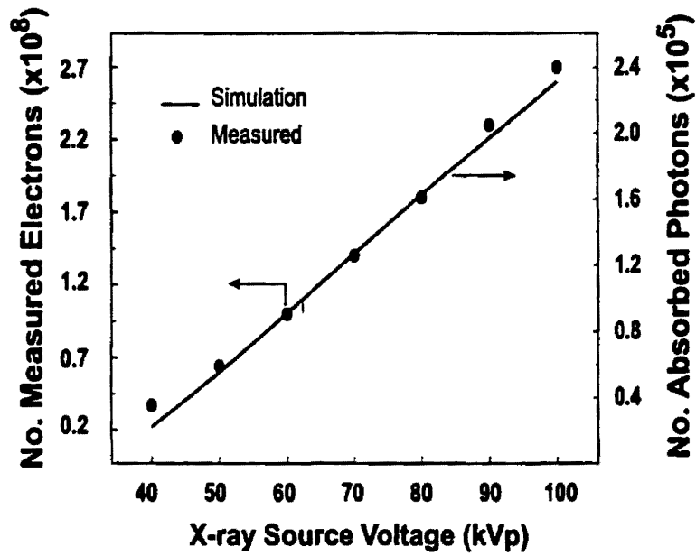
Figure 5.12: Response of detector for various X-ray source voltages (kVp), collected over a period of 500 ms .
