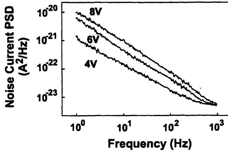
Figure 4.2: Measured power spectral densities for a 200 \mu m \times 200 \mu m device at the indicated values of the reverse bias.
