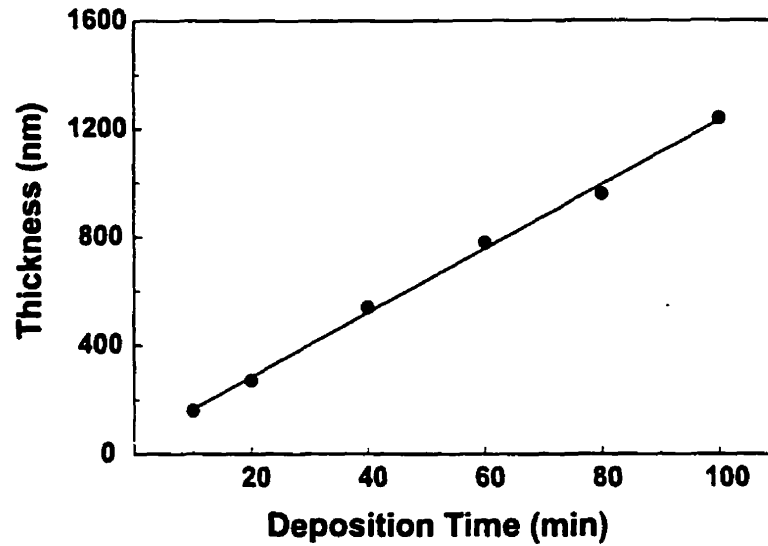
Figure 2.2: Variation of a-Si:H thickness with deposition time.
