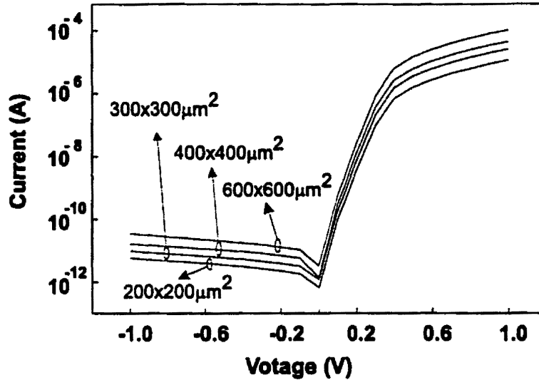
Figure 2.13: Typical I-V characteristic of fabricated Mo/a-Si:H Schottky diodes with various geometries.
