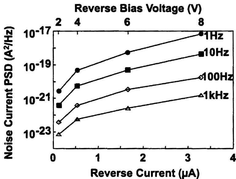
Figure 4.6: Measured power spectral densities as a function of bias for a 400 \mu\text{m} \times 400 \mu\text{m} at the indicated frequencies.
