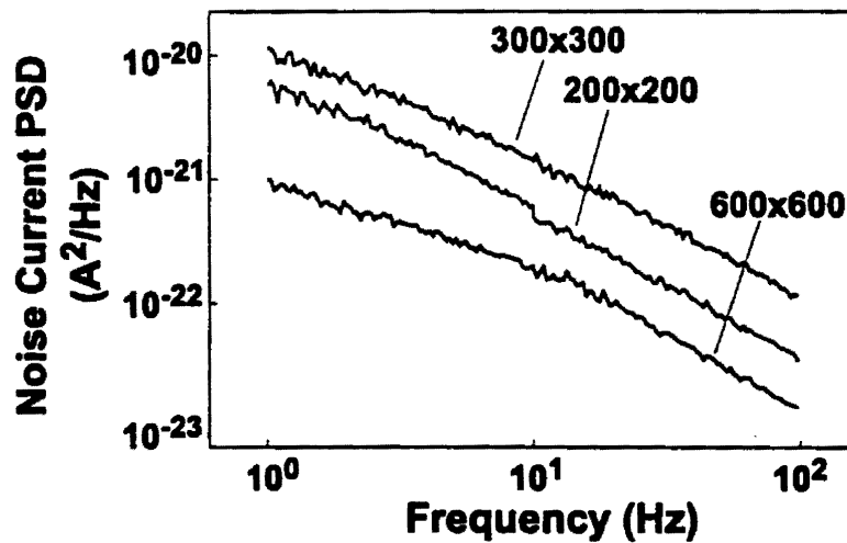
Figure 4.4: Measured power spectral densities for devices with various geometries (dimensions in \mu\text{m} ) at 6 V reverse bias.
