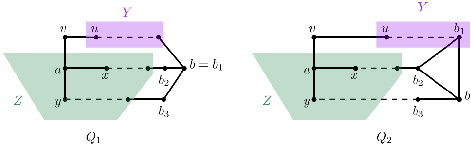
Fig. 7. Name conventions for vertices in the proof of Theorem 4.6 in the case when Q = Q_i is a theta ( i = 1 ) and when Q = Q_i is a pyramid ( i = 2 ). Dashed lines represent paths of arbitrary length (possibly zero).
