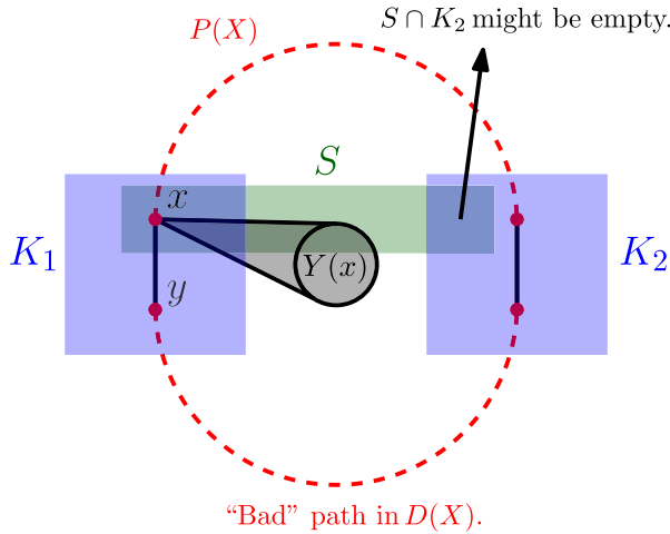
Fig. 10. Proof of Theorem 8.3 . We have shown that P(X) is disjoint from S , and that x has neighbours in both R' and \hat{R} , and so x \in S . Dashed lines represent paths of arbitrary length (possibly zero).
