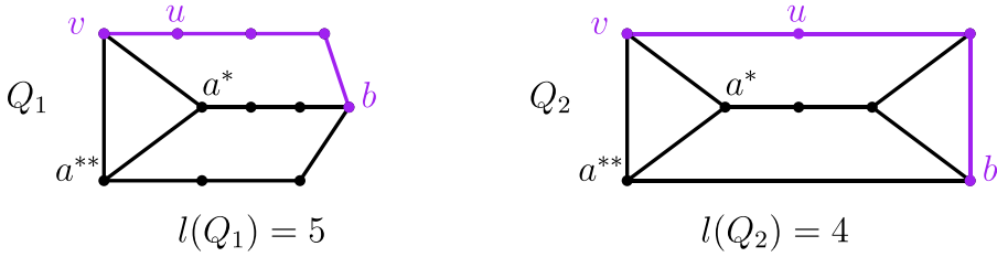
Fig. 3. In the proof of Theorem 4.3 , the choice of b = b(Q_i) and a path with l(Q_i) vertices of the form P_1(Q_i) \cup \{b\} in the case that Q_i is a pyramid ( i = 1 ) or Q_i is a prism ( i = 2 ).
