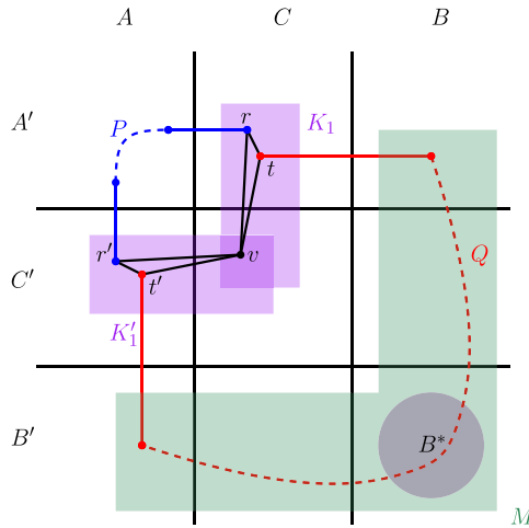
Fig. 8. The proof of Theorem 6.1. Dashed lines represent paths of arbitrary length (possibly zero).
