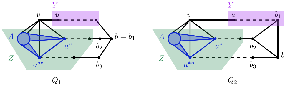
Fig. 4. The sets A , Y and Z in the proof of Theorem 4.3 , in the case that Q_i is a pyramid ( i = 1 ) or Q_i is a prism ( i = 2 ). Dashed lines represent paths of arbitrary length (possibly zero).
