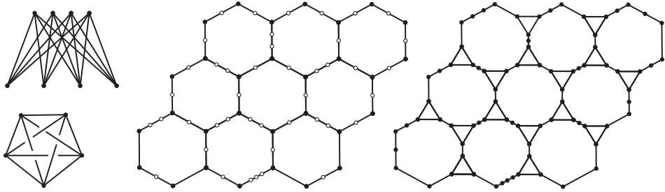
Fig. 1. The 4-basic obstructions.
