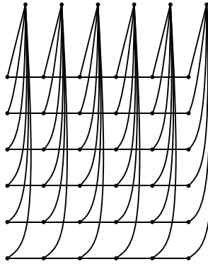
Fig. 2. A graph from the Pohoata–Davies construction.
