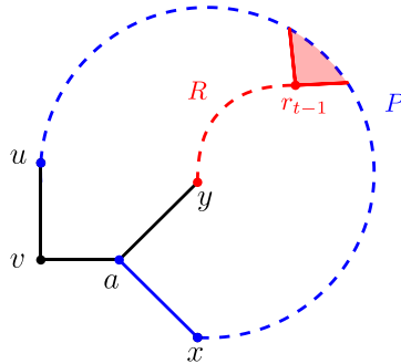
Fig. 6. Proof of Lemma 4.5. Dashed lines represent paths of arbitrary length (possibly zero).
