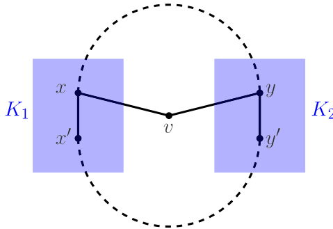
Fig. 9. Proof of Lemma 7.2. A clock in the case that some vertex in X is adjacent to both x and y . Dashed lines represent paths of arbitrary length (possibly zero).
