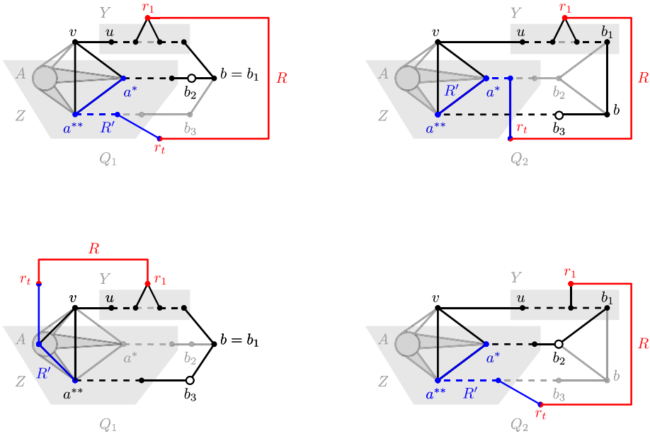
Fig. 5. Some of the cases for (7), assuming neither b_i nor v has a neighbour in R^* . In each case, b_i is depicted by a hollow node, and a better choice of Q has been highlighted (consisting of R, R' and bits of the previous choice of Q ). The vertex r_1 may have one neighbour or two consecutive neighbours in P_1(Q) ; this only affects whether the better choice for Q is a pyramid or a prism.
