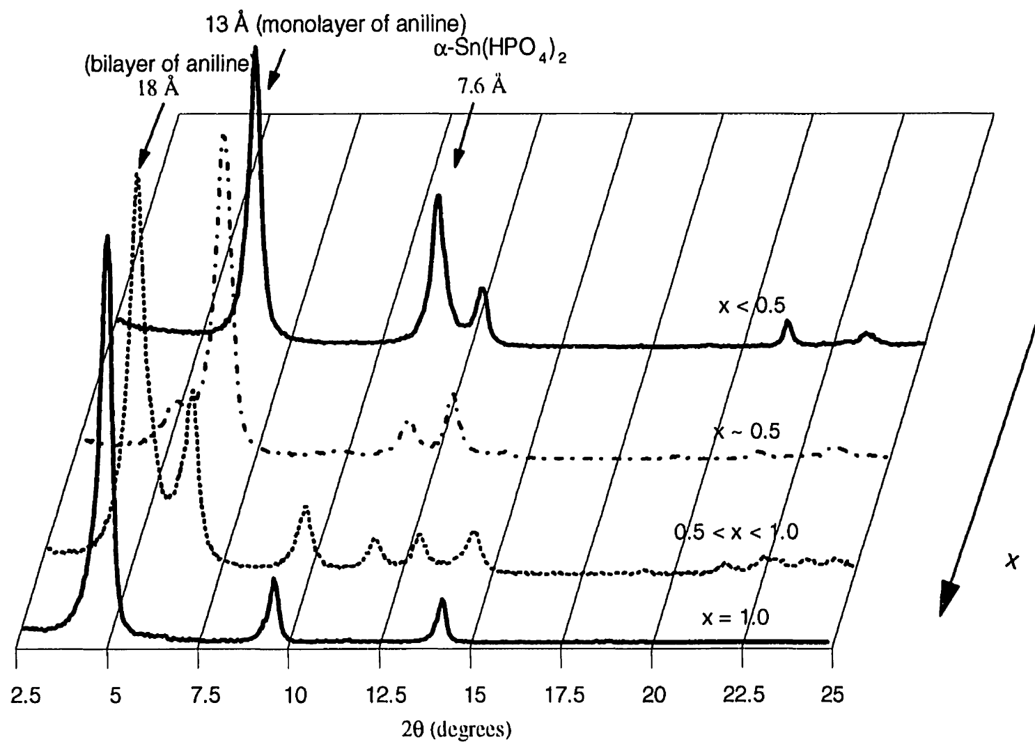
Figure 6.3 Powder XRD patterns of oriented films of (\text{Anilinium})_x\alpha\text{-Sn}(\text{OPO}_3)_x(\text{HOPO}_3)_{2-x} ( 0 < x \leq 1 )
