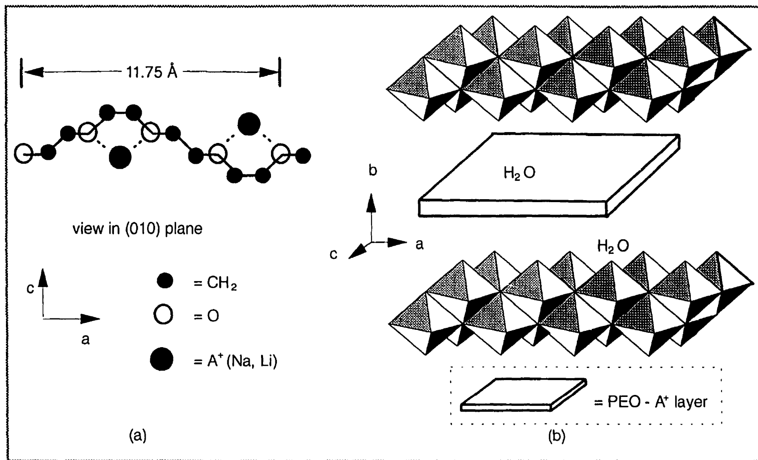
Figure 3.7 Schematic diagrams of the proposed structure of the monolayer (PEO) 0.4 [Na(H 2 O) n ] 0.25 MoO 3 nanocomposite showing views of (a) the plane parallel to and midway between the MoO 3 sheets and (b) the view of the plane perpendicular to the MoO 3 sheets ( 100 )
