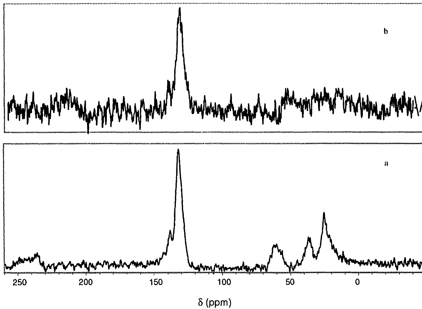
Figure 7.6 ^{13}\text{C} CPMAS NMR spectra of (a) (\text{PPV}^+)_{1.0}\alpha\text{-Sn}(\text{OPO}_3)_{1.0}(\text{HOPO}_3)_{1.0}\cdot\text{H}_2\text{O} and (b) (\text{PPV})_{1.0}\alpha\text{-Sn}(\text{HOPO}_3)_{2.0}
