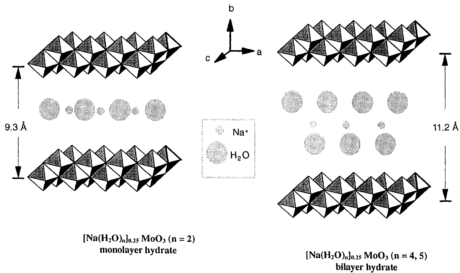
Figure 3.1 Proposed schematic structure of [\text{Na}(\text{H}_2\text{O})_2]_{0.25}\text{MoO}_3 (vacuum dried) and [\text{Na}(\text{H}_2\text{O})_n]_{0.25}\text{MoO}_3 ( n > 4 ) (air dried)
