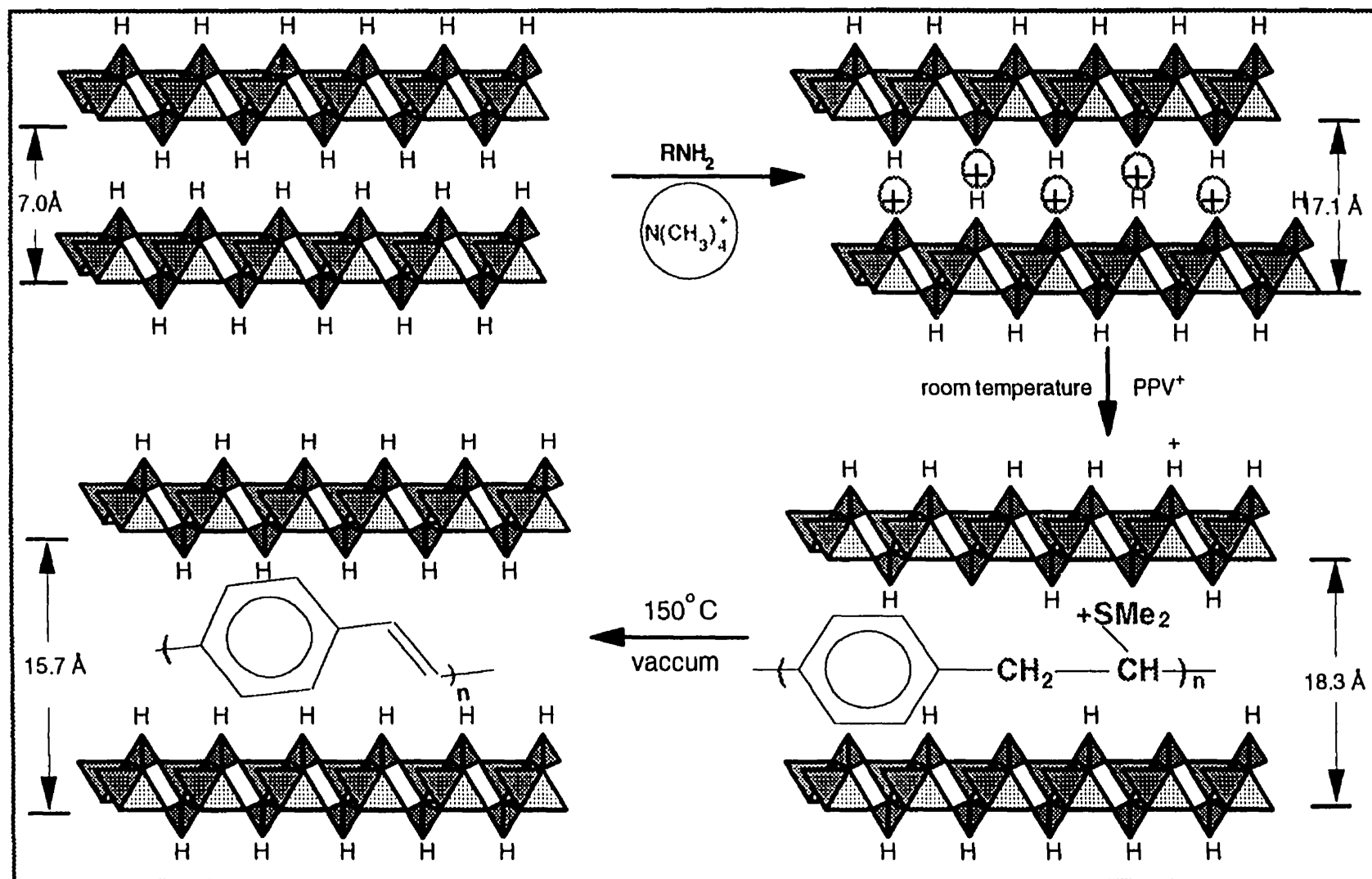
Figure 7.1 Synthetic scheme for (\text{PPV})_{1.0\alpha}\text{-Sn}(\text{HOPO}_3)_2
