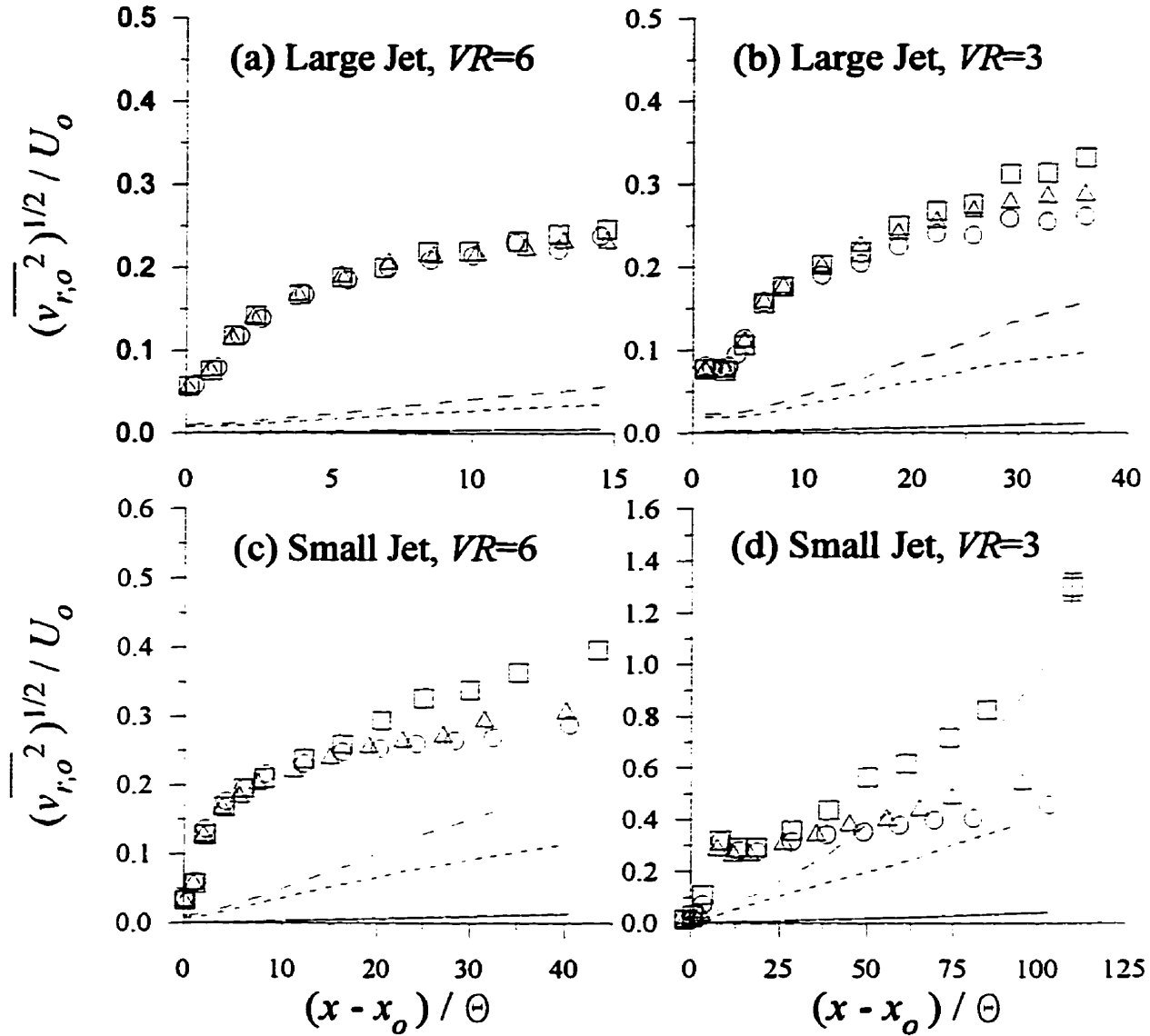
Figure 5.27: Jet centerline and external radial turbulent velocities normalized by U_o . Symbols refer to the jet centerline for a given grid: \circ , no grid; \Delta , small grid; \square , large grid. Lines refer to the external levels: —, no grid; ----, small grid; - · -, large grid.
