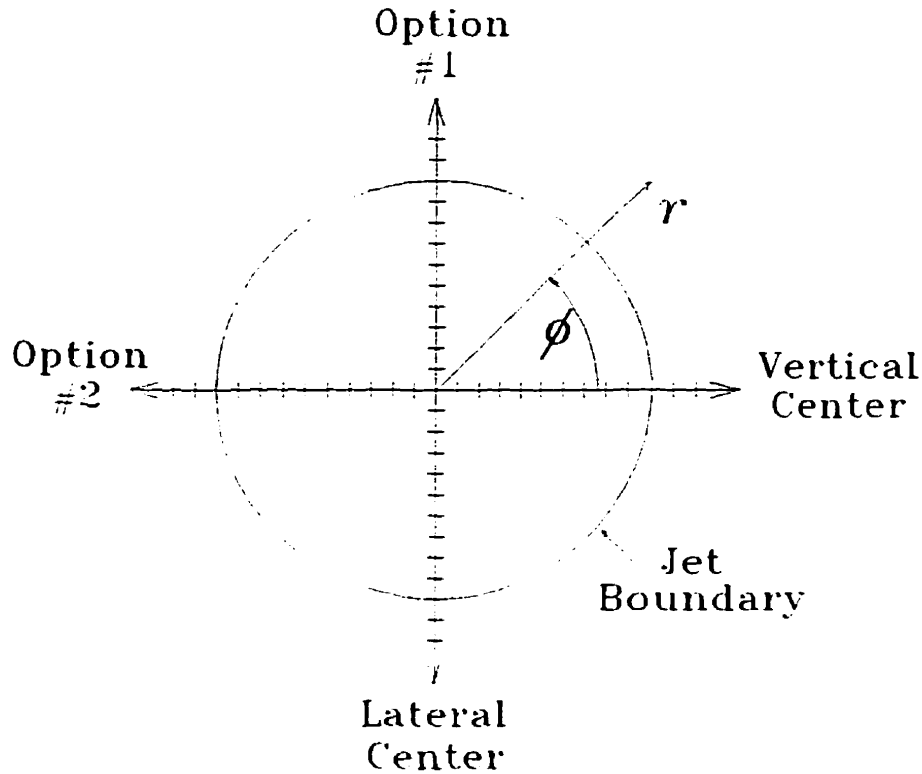
Figure 3.3: Illustration of the two traversing options available for LDA measurements on the jet centerline in the (r, \phi) plane.
