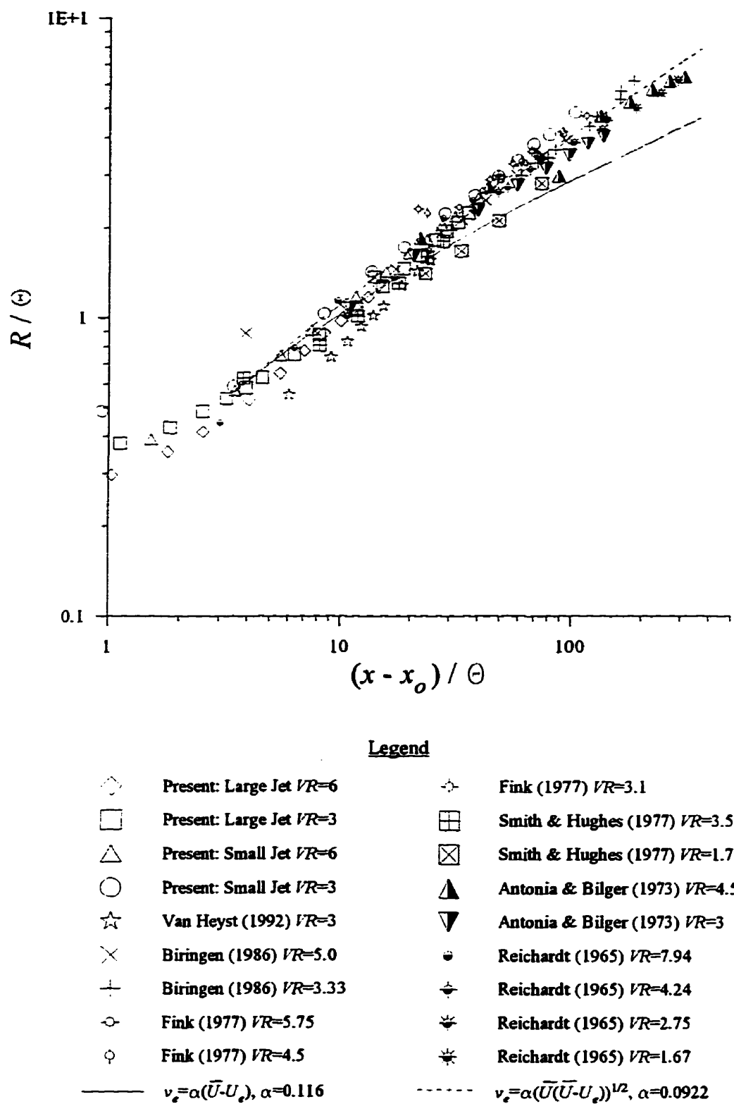
Figure 6.2: Comparison of predicted behaviour for R/\theta with experimental data for jets in laminar coflows.
