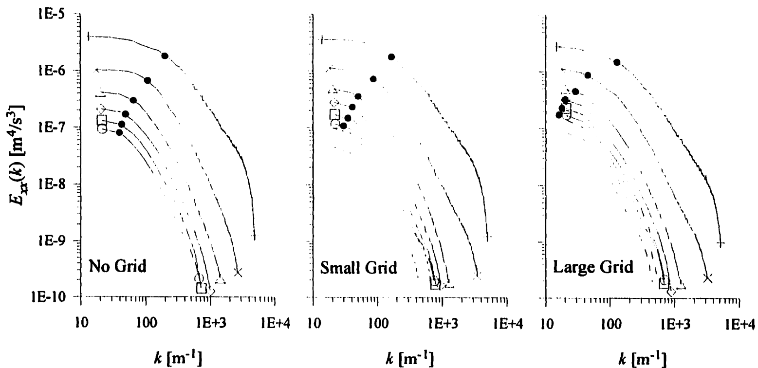
Figure 5.44: Average streamwise turbulent energy spectra for the small jet at V/R \approx 3 . x (cm): +, 10; x, 20; Δ, 40; ◇, 60; □, 80; ○, 100. (x-x_0)/\theta : +, 9.9; x, 19.6; Δ, 39.5; ◇, 60.3; □, 81.8; ○, 105.7. External spectra range: - - -, small grid; - - -, large grid. Solid bullets, ●, give approximate locations of L_{xx} on spectra.
