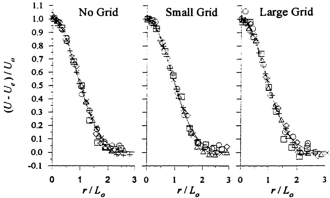
Figure 5.2: Excess mean velocity profiles for the large jet with VR \approx 3 . x (cm): +, 10; \times , 20; \Delta , 40; \diamond , 60; \square , 80; \circ , 100. (x - x_0)/\theta : +, 4.6; \times , 8.1; \Delta , 15.2; \diamond , 22.2; \square , 29.2; \circ , 36.2. —, Gaussian function.
