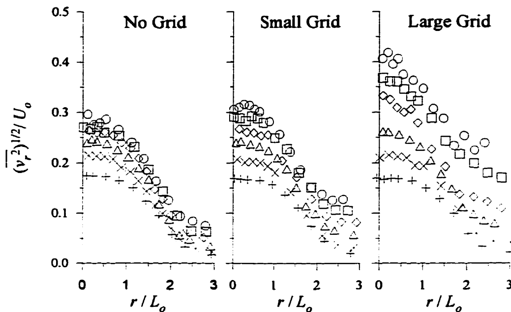
Figure 5.23: Radial turbulent velocity profiles for the small jet with VR \approx 6 normalized by U_o . x (cm): +, 10; ×, 20; Δ, 40; ◇, 60; □, 80; ○, 100. (x-x_o)/\theta : +, 3.3; ×, 7.3; Δ, 15.2; ◇, 23.4; □, 32.4; ○, 40.7.
