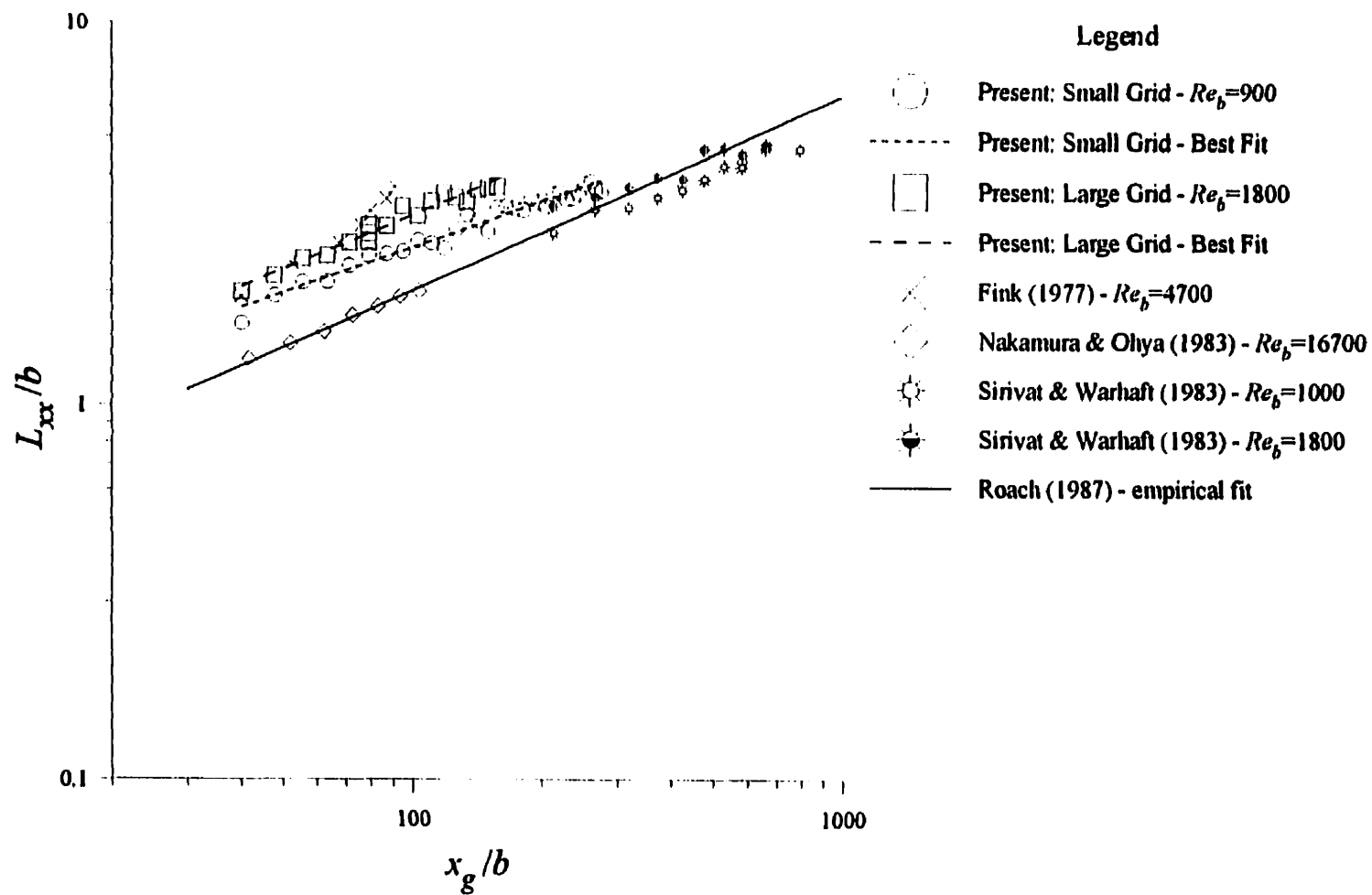
Figure 4.6: Normalized streamwise integral length scales produced by grid-generated turbulence.
