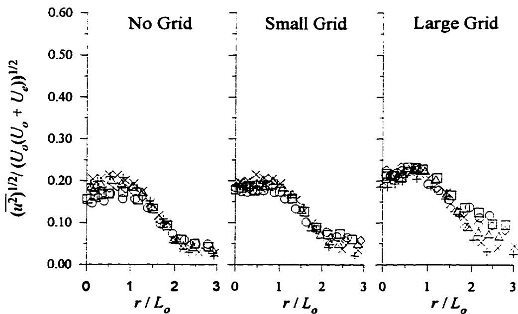
Figure 5.14: Streamwise turbulent velocity profiles for the small jet with VR \approx 6 normalized by ((U_o + U_e))^{1/2} . x (cm): +, 10; x, 20; \Delta , 40; \diamond , 60; \square , 80; \circ , 100. (x-x_o)/\theta : +, 3.3; x, 7.3; \Delta , 15.2; \diamond , 23.4; \square , 32.4; \circ , 40.7.
