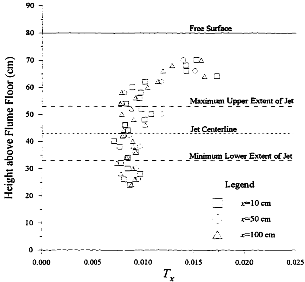
Figure 4.2: Vertical variation of the external streamwise turbulent intensity in the absence of any grid.
