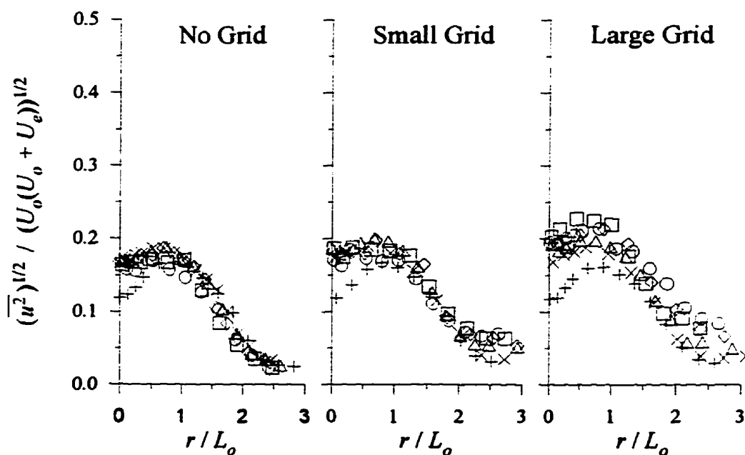
Figure 5.12: Streamwise turbulent velocity profiles for the large jet with VR \approx 3 normalized by (U_o(U_o + U_e))^{1/2} . x (cm): +, 10; ×, 20; Δ, 40; ◇, 60; □, 80; ○, 100. (x-x_o)/\theta : +, 4.6; ×, 8.1; Δ, 15.2; ◇, 22.2; □, 29.2; ○, 36.2.
