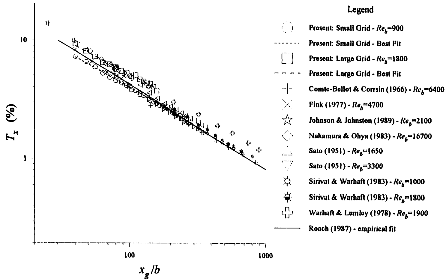
Figure 4.4: Streamwise turbulent intensities produced by grid-generated turbulence.
