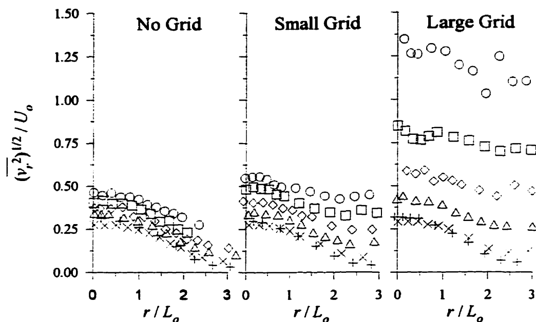
Figure 5.25: Radial turbulent velocity profiles for the small jet with VR \approx 3 normalized by U_o . x (cm): +, 10; ×, 20; Δ, 40; ◇, 60; □, 80; ○, 100. (x-x_o)/\theta : +, 9.9; ×, 19.6; Δ, 39.5; ◇, 60.3; □, 81.8; ○, 105.7.
