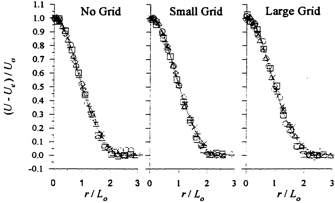
Figure 5.1: Excess mean velocity profiles for the large jet with VR \approx 6 . x (cm): +, 10; \times , 20; \Delta , 40; \diamond , 60; \square , 80; \circ , 100. (x - x_0)/\theta : +, 0.8; \times , 2.3; \Delta , 5.2; \diamond , 8.6; \square , 11.8; \circ , 14.8. —, Gaussian function.
