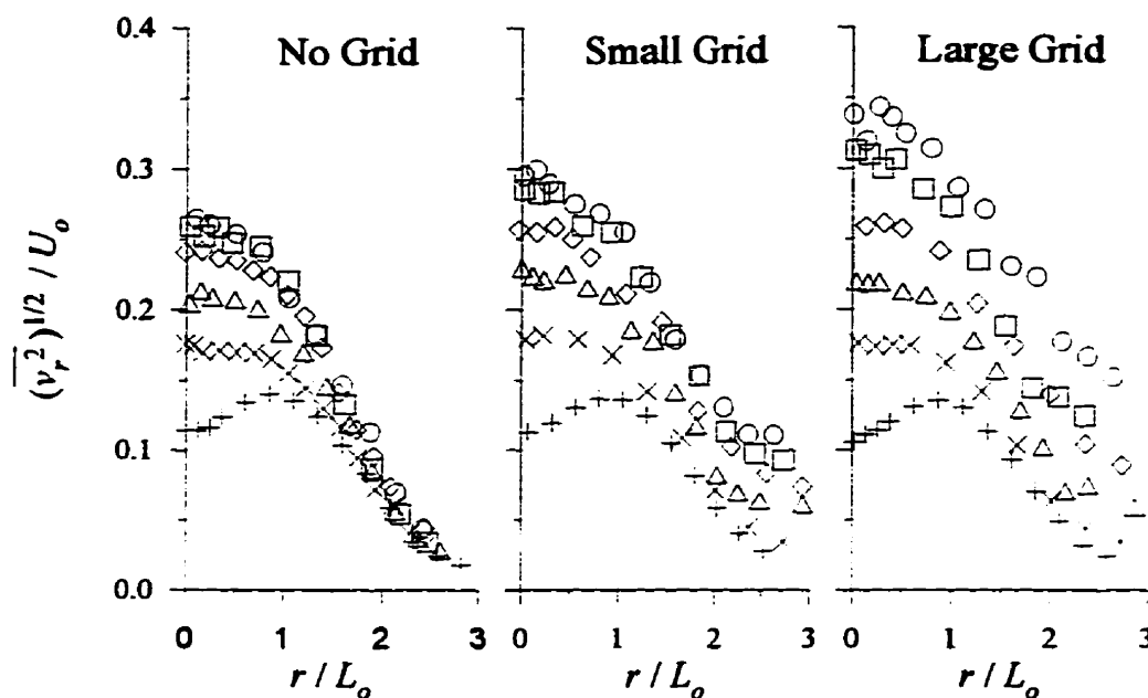
Figure 5.21: Radial turbulent velocity profiles for the large jet with VR \approx 3 normalized by U_o . x (cm): +, 10; ×, 20; Δ, 40; ◇, 60; □, 80; ○, 100. (x-x_o)/\theta : +, 4.6; ×, 8.1; Δ, 15.2; ◇, 22.2; □, 29.2; ○, 36.2.
