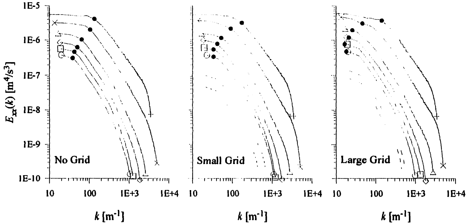
Figure 5.43: Average streamwise turbulent energy spectra for the small jet at V/R \approx 6 . x (cm): + , 10; \times , 20; \Delta , 40; \diamond , 60; \square , 80; \circ , 100. (x-x_0)/\theta : + , 3.3; \times , 7.3; \Delta , 15.2; \diamond , 23.4; \square , 32.4; \circ , 40.7. External spectra range: - - -, small grid; - - -, large grid. Solid bullets, \bullet , give approximate locations of L_{\alpha\alpha} on spectra.
