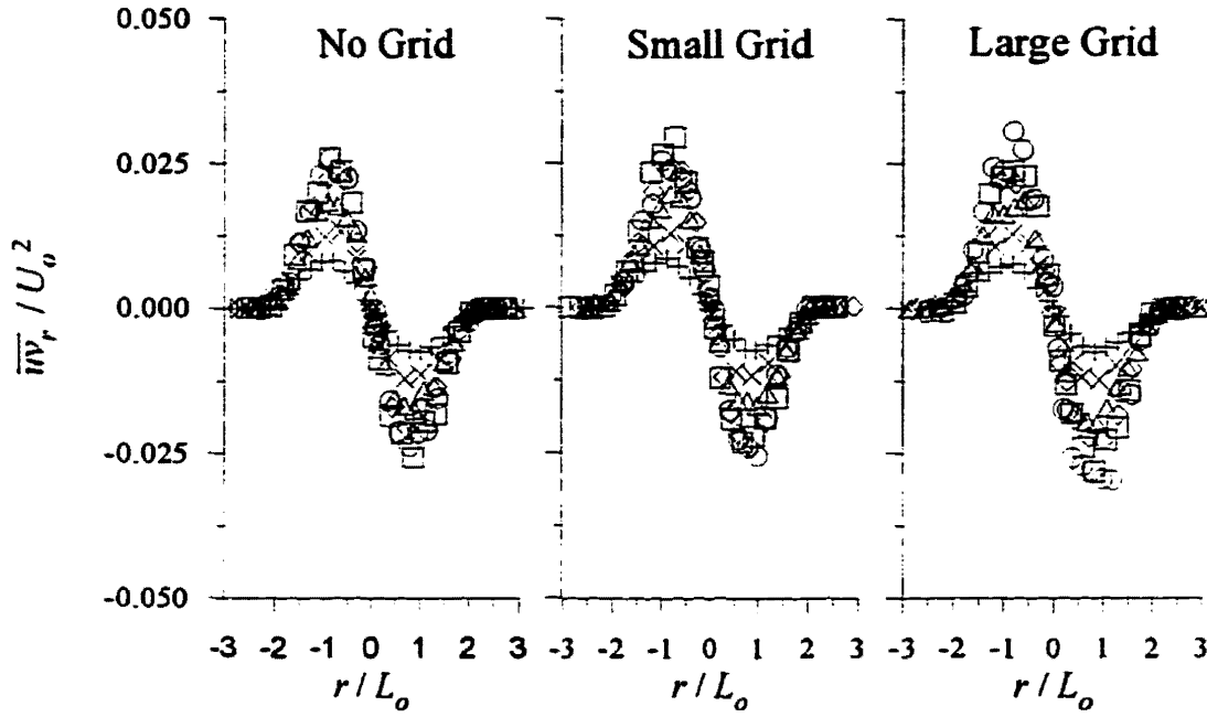
Figure 5.29 : Reynolds shear stress profiles for the large jet with VR \approx 6 normalized by U_o^2 . x (cm): +, 10; \times , 20; \Delta , 40; \diamond , 60; \square , 80; \circ , 100. (x-x_o)/\theta : +, 0.8; \times , 2.3; \Delta , 5.2; \diamond , 8.6; \square , 11.8; \circ , 14.8.
