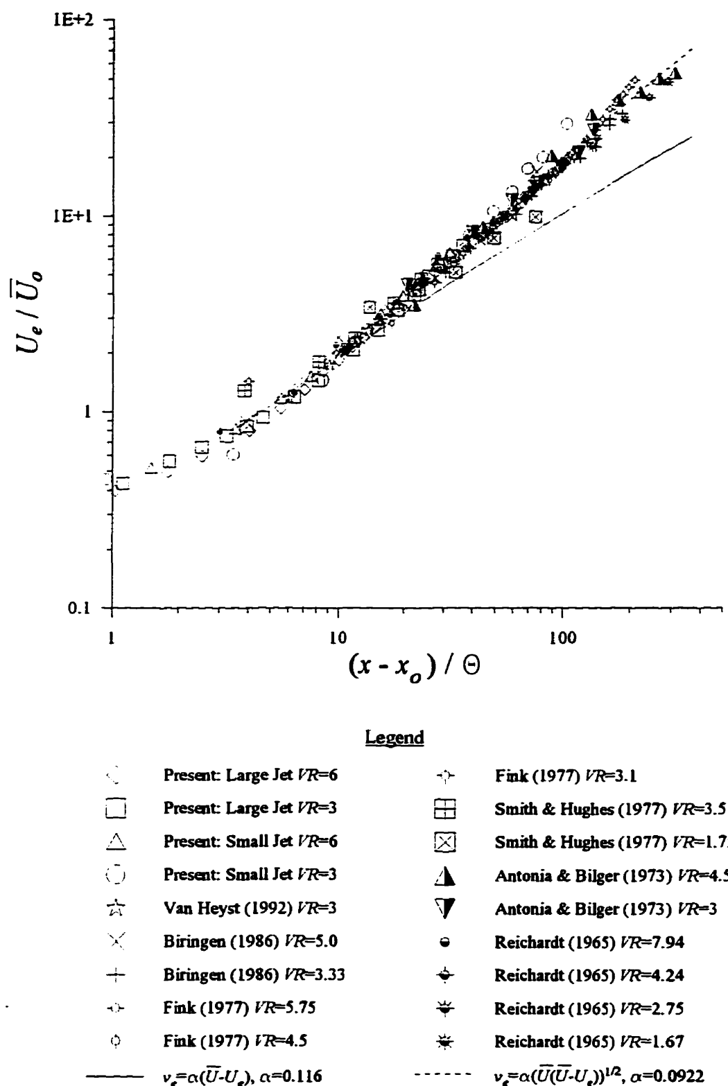
Figure 6.1: Comparison of predicted behaviour for U_e / U_o with experimental data for jets in laminar coflows.
