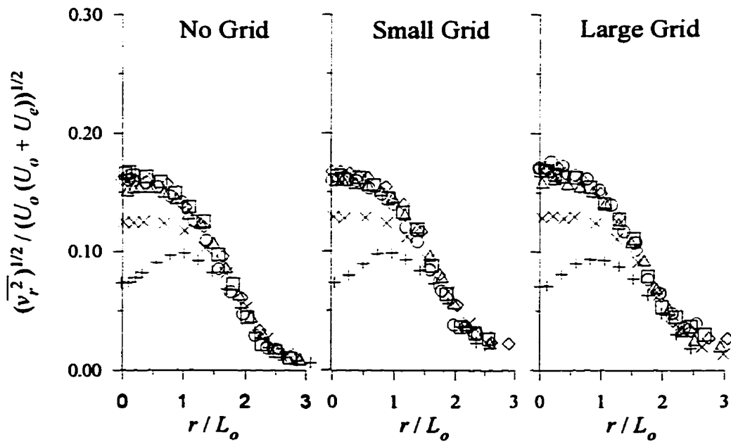
Figure 5.20: Radial turbulent velocity profiles for the large jet with VR \approx 6 normalized by (U_o(U_o+U_e))^{1/2} . x (cm): +, 10; ×, 20; Δ, 40; ◇, 60; □, 80; ○, 100. (x-x_o)/\theta : +, 0.8; ×, 2.3; Δ, 5.2; ◇, 8.6; □, 11.8; ○, 14.8.
