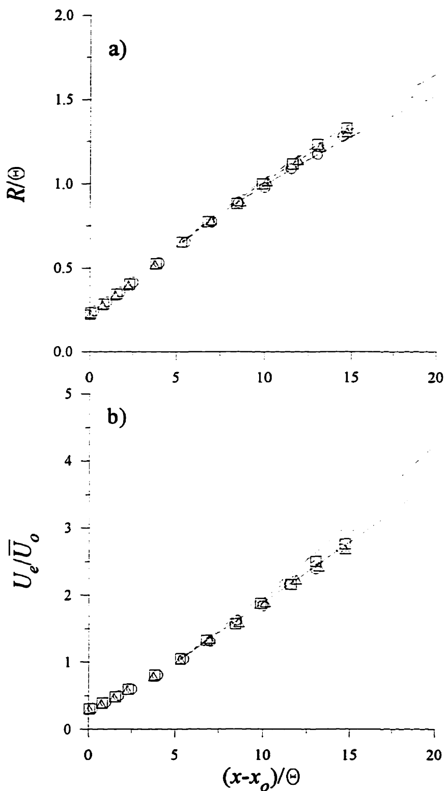
Figure 6.3: Comparison of predictions and experimental data for the large jet at VR \approx 6 . Data: \circ , no grid; \triangle , small grid; \square , large grid. Predictions: —, no grid; - - -, small grid; - · -, large grid.
