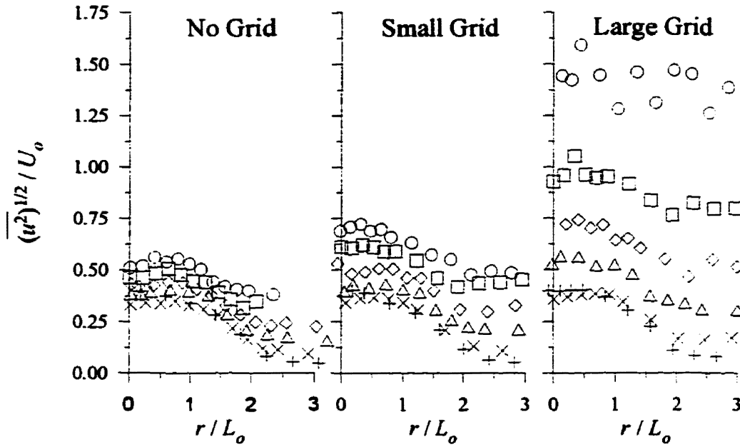
Figure 5.15: Streamwise turbulent velocity profiles for the small jet with VR \approx 3 normalized by U_o . x (cm): +, 10; ×, 20; Δ, 40; ◇, 60; □, 80; ○, 100. (x-x_o)/\theta : +, 9.9; ×, 19.6; Δ, 39.5; ◇, 60.3; □, 81.8; ○, 105.7.
