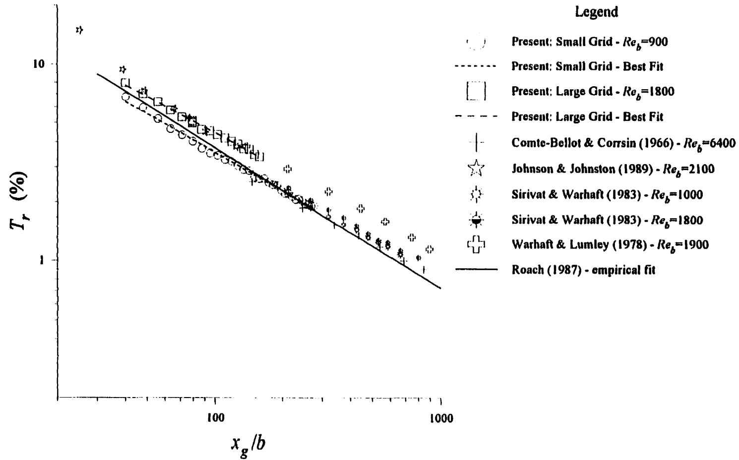
Figure 4.5: Radial or transverse turbulent intensities produced by grid-generated turbulence.
