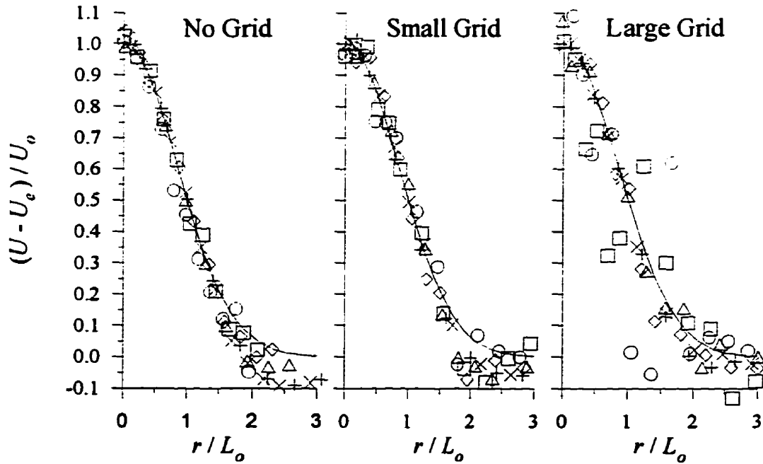
Figure 5.4: Excess mean velocity profiles for the small jet with VR \approx 3 . x (cm): +, 10; \times , 20; \Delta , 40; \diamond , 60; \square , 80; \circ , 100. (x - x_o) / \theta : +, 9.9; \times , 19.6; \Delta , 39.5; \diamond , 60.3; \square , 81.8; \circ , 105.7. —, Gaussian function.
