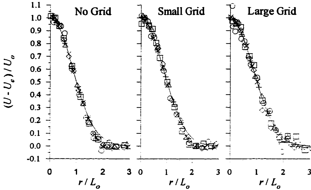
Figure 5.3 : Excess mean velocity profiles for the small jet with VR \approx 6 . x (cm): +, 10; \times , 20; \Delta , 40; \diamond , 60; \square , 80; \circ , 100. (x - x_o) / \theta : +, 3.3; \times , 7.3; \Delta , 15.2; \diamond , 23.4; \square , 32.4; \circ , 40.7. —, Gaussian function.
