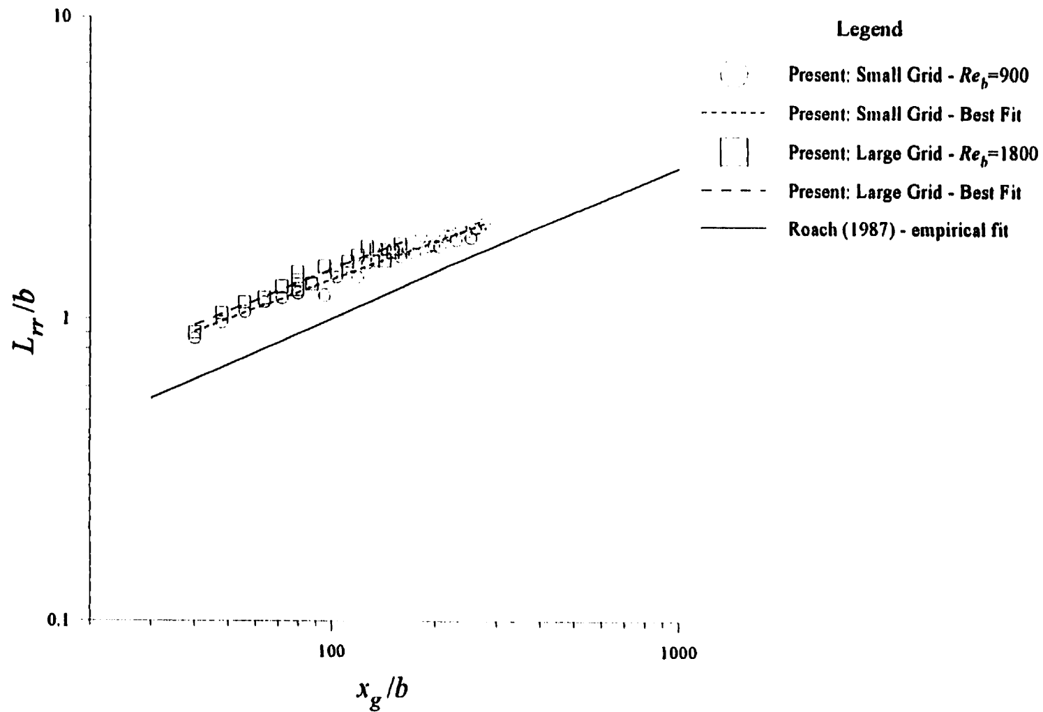
Figure 4.7: Normalized transverse integral length scales produced by grid-generated turbulence.
