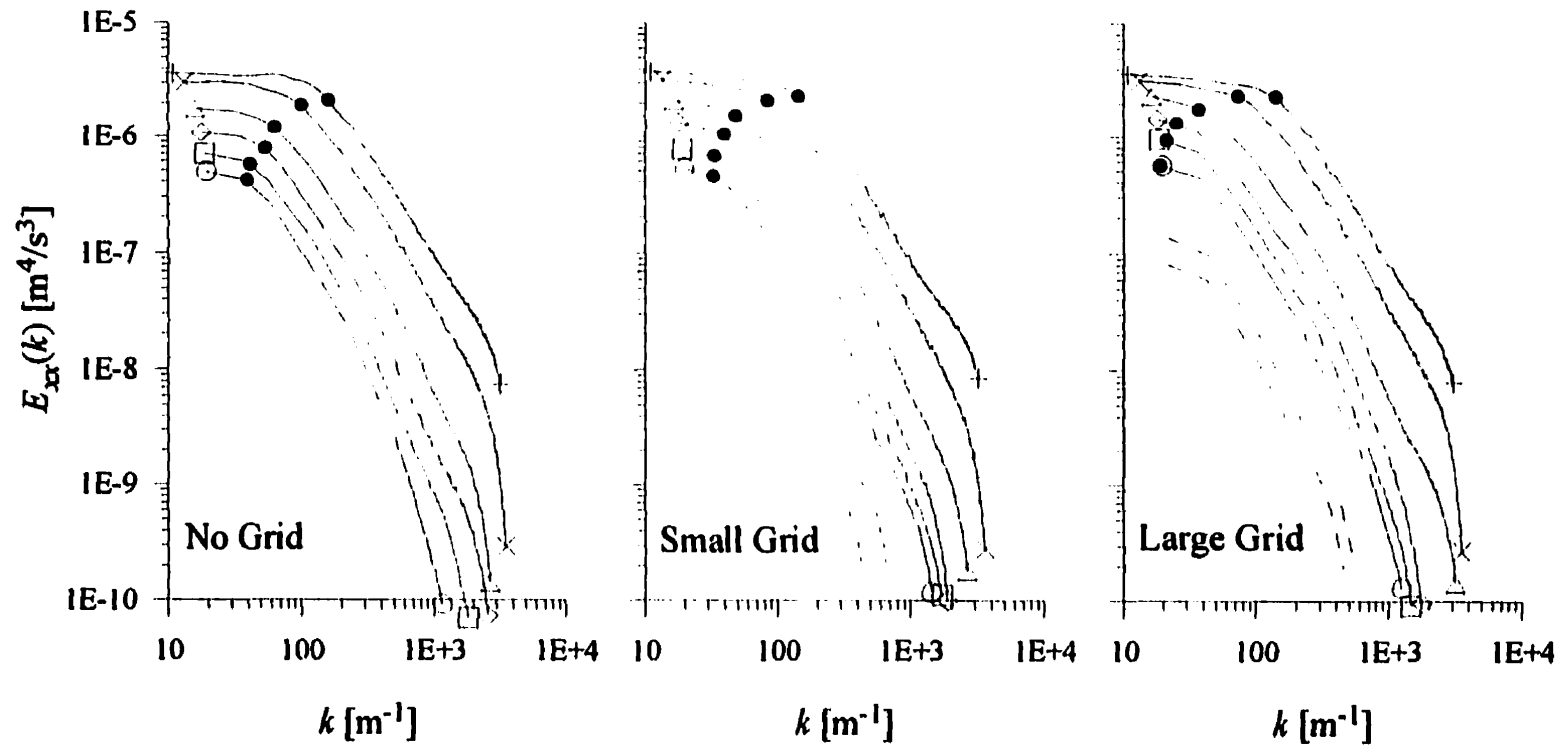
Figure 5.42: Average streamwise turbulent energy spectra for the large jet at V/R \approx 3 . x (cm): +, 10; ×, 20; Δ, 40; ◇, 60; □, 80; ○, 100. (x-x_0)/\theta : +, 4.6; ×, 8.1; Δ, 15.2; ◇, 22.2; □, 29.2; ○, 36.2. External spectra range: - - -, small grid; - · -, large grid. Solid bullets, •, give approximate locations of L_{xx} on spectra.
