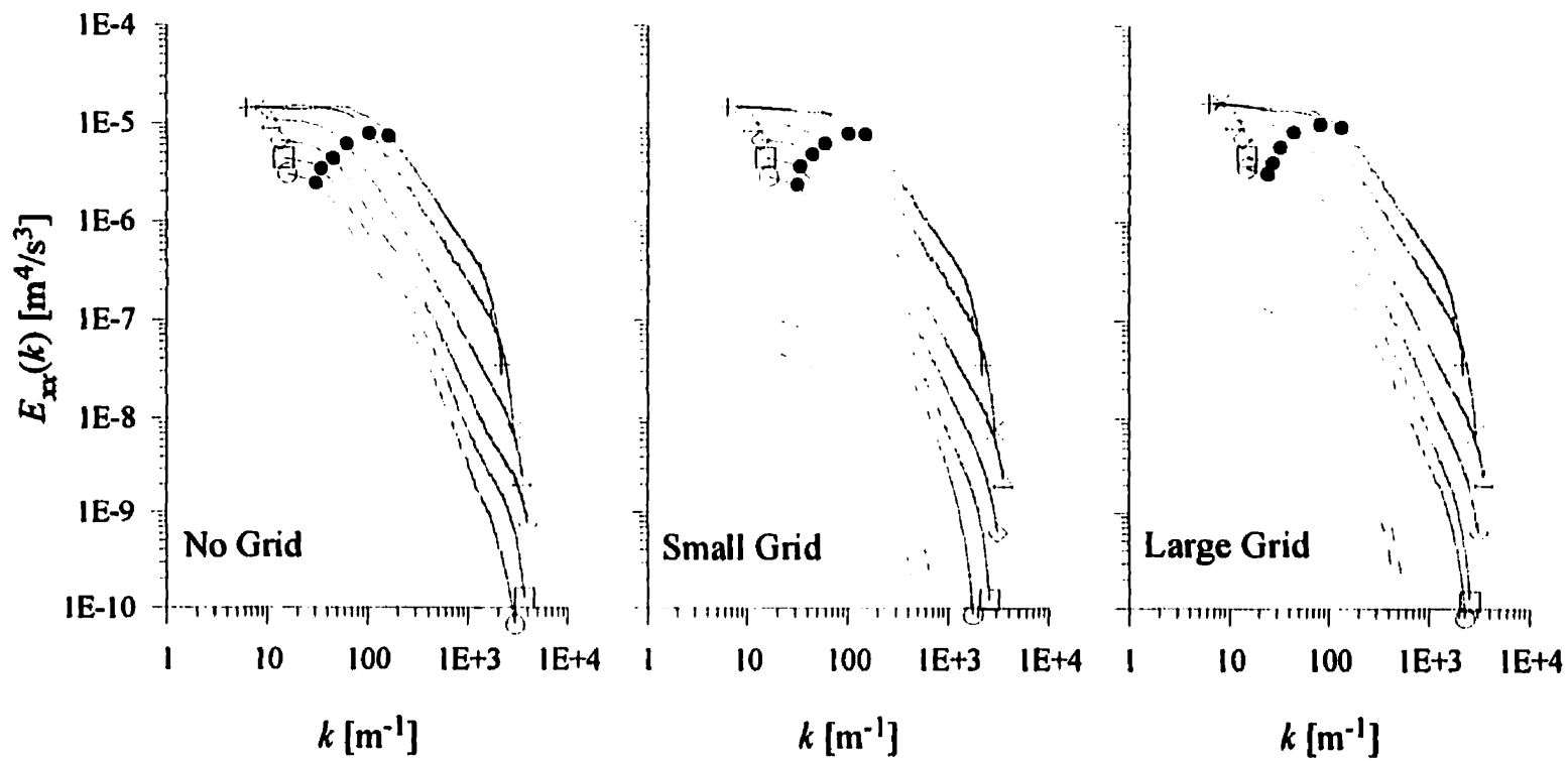
Figure 5.41: Average streamwise turbulent energy spectra for the large jet at VR \approx 6 . x (cm): +, 10; ×, 20; Δ, 40; ◇, 60; □, 80; ○, 100. (x-x_o)/\theta : +, 0.8; ×, 2.3; Δ, 5.2; ◇, 8.6; □, 11.8; ○, 14.8. External spectra range: - - - -, small grid; - - -, large grid. Solid bullets, •, give approximate locations of L_{xx} on spectra.
