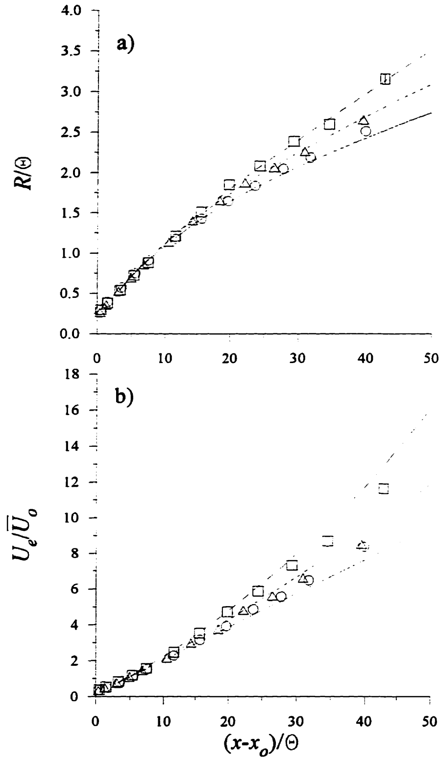
Figure 6.5: Comparison of predictions and experimental data for the small jet at VR \approx 6 . Data: \circ , no grid; \triangle , small grid; \square , large grid. Predictions: —, no grid; - - -, small grid; - · - · -, large grid.
