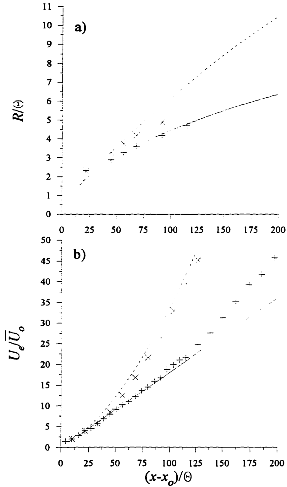
Figure 6.9: Comparison of predictions and experimental data for Fink's jet at VR \approx 3.1 . Data: +, no grid; ×, grid. Predictions: —, no grid; - - -, grid.
