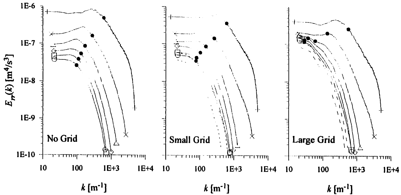
Figure 5.48: Average radial turbulent energy spectra for the small jet at V/R \approx 3 . x (cm): +, 10; ×, 20; Δ, 40; ◇, 60; □, 80; ○, 100. (x-x_0)/\theta : +, 9.9; ×, 19.6; Δ, 39.5; ◇, 60.3; □, 81.8; ○, 105.7. External spectra range: - - - , small grid; - - , large grid. Solid bullets, ●, give approximate locations of L_r on spectra.
