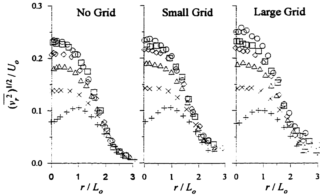
Figure 5.19: Radial turbulent velocity profiles for the large jet with VR \approx 6 normalized by U_o . x (cm): +, 10; ×, 20; Δ, 40; ◇, 60; □, 80; ○, 100. (x-x_o)/\theta : +, 0.8; ×, 2.3; Δ, 5.2; ◇, 8.6; □, 11.8; ○, 14.8.
