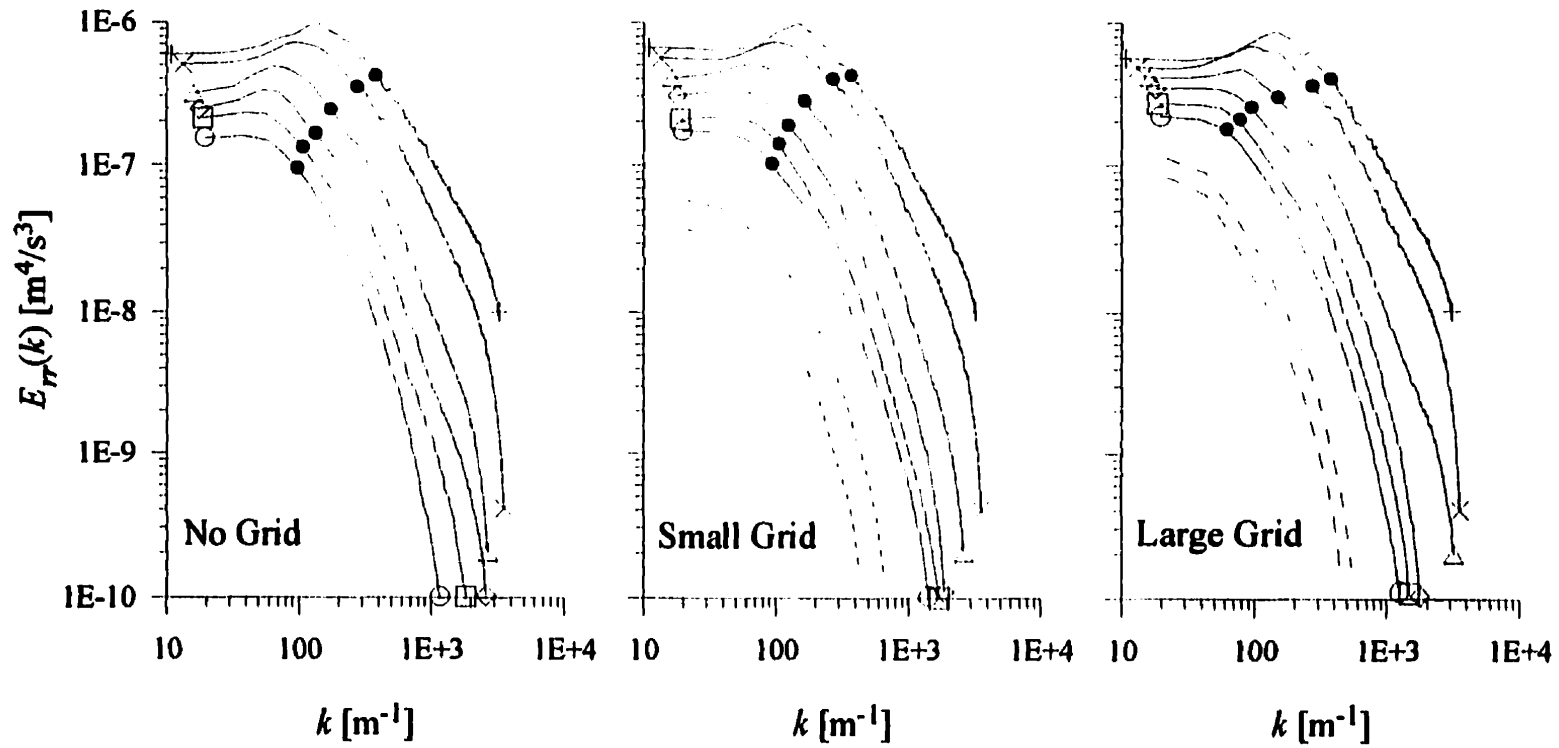
Figure 5.46: Average radial turbulent energy spectra for the large jet at V/R \approx 3 . x (cm): + , 10; \times , 20; \triangle , 40; \diamond , 60; \square , 80; \circ , 100. (x-x_0)/\theta : + , 4.6; \times , 8.1; \triangle , 15.2; \diamond , 22.2; \square , 29.2; \circ , 36.2. External spectra range: - - - , small grid; - - , large grid. Solid bullets, \bullet , give approximate locations of L_r on spectra.
