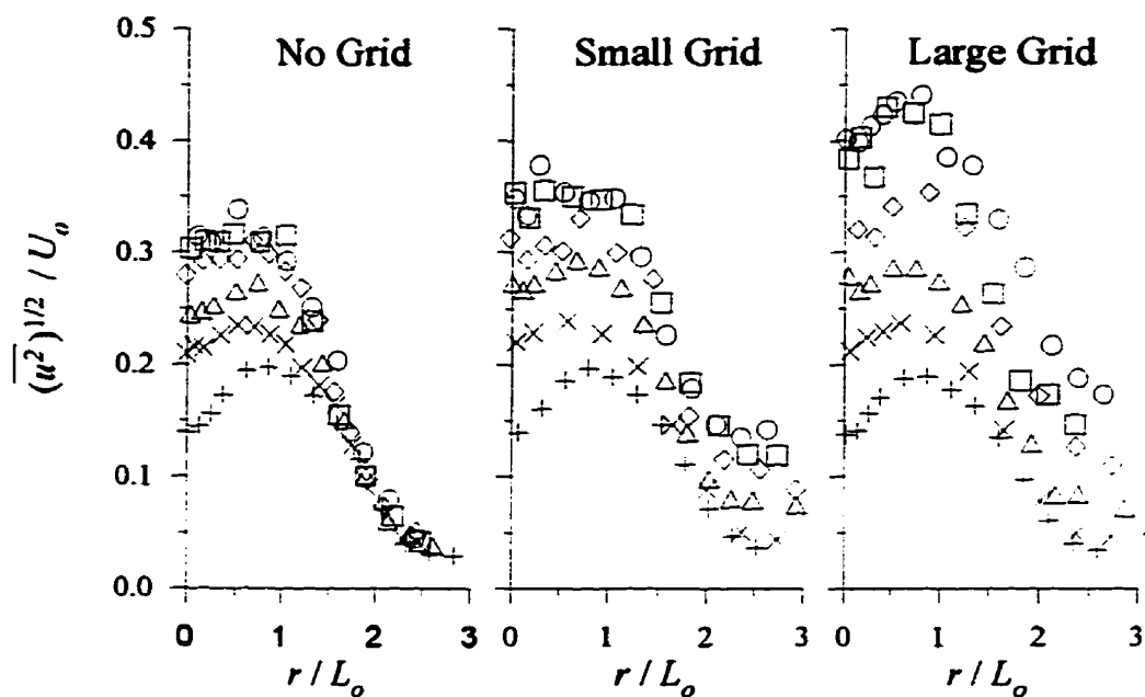
Figure 5.11: Streamwise turbulent velocity profiles for the large jet with VR \approx 3 normalized by U_o . x (cm): +, 10; ×, 20; Δ, 40; ◇, 60; □, 80; ○, 100. (x-x_o)/\theta : +, 4.6; ×, 8.1; Δ, 15.2; ◇, 22.2; □, 29.2; ○, 36.2.
