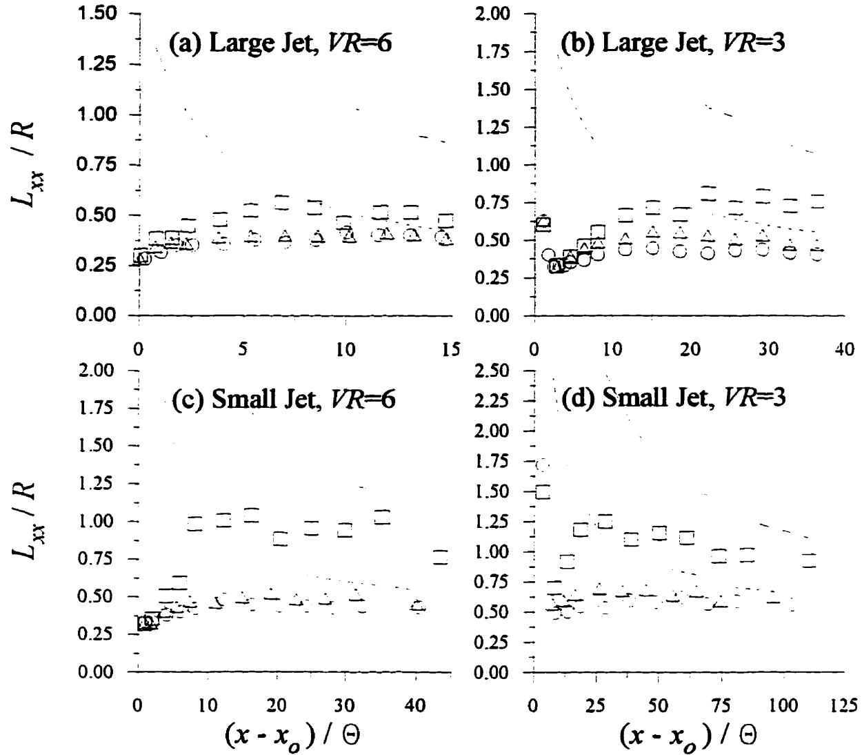
Figure 5.39: Average streamwise integral length scales normalized by the jet radius. Symbols refer to the jet for a given grid: ○, no grid; △, small grid; □, large grid. Lines refer to levels in the external flow also normalized by R : - - -, small grid; - - -, large grid.
