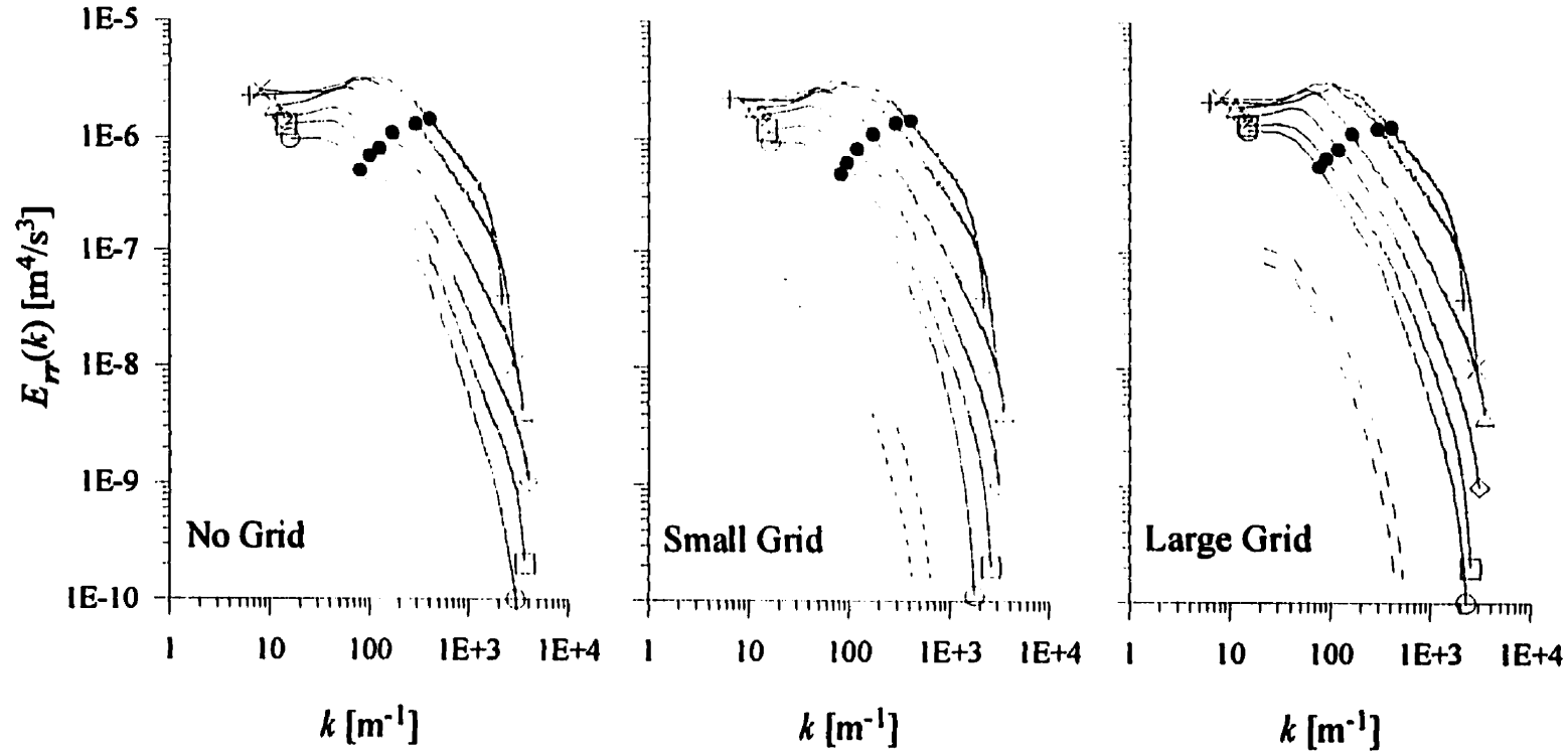
Figure 5.45: Average radial turbulent energy spectra for the large jet at VR \approx 6 . x (cm): +, 10; \times , 20; \Delta , 40; \diamond , 60; \square , 80; \circ , 100. (x-x_0)/\theta : +, 0.8; \times , 2.3; \Delta , 5.2; \diamond , 8.6; \square , 11.8; \circ , 14.8. External spectra range: - - -, small grid; - . -, large grid. Solid bullets, \bullet , give approximate locations of L_r on spectra.
