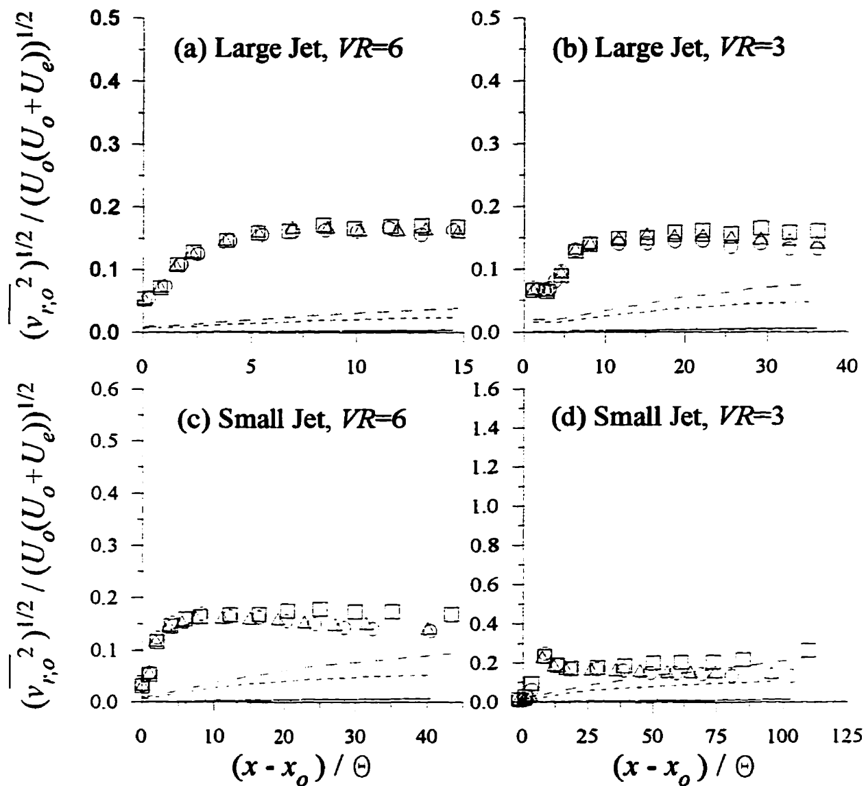
Figure 5.28: Jet centerline and external radial turbulent velocities normalized by (U_o(U_o + U_e))^{1/2} . Symbols refer to the jet centerline for a given grid: \circ , no grid; \Delta , small grid; \square , large grid. Lines refer to the external levels: —, no grid; ----, small grid; - - -, large grid.
