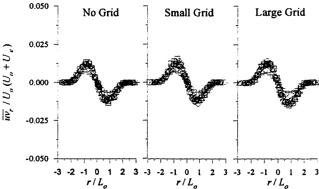
Figure 5.30 : Reynolds shear stress profiles for the large jet with VR \approx 6 normalized by U_o(U_o + U_e) . x (cm): +, 10; \times , 20; \Delta , 40; \diamond , 60; \square , 80; \circ , 100. (x-x_o)/\theta : +, 0.8; \times , 2.3; \Delta , 5.2; \diamond , 8.6; \square , 11.8; \circ , 14.8.
