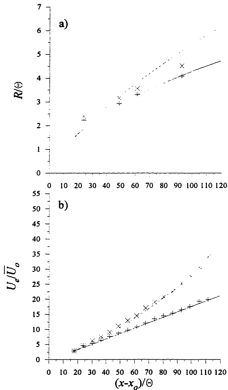
Figure 6.8: Comparison of predictions and experimental data for Fink's jet at VR \approx 4.5 . Data: +, no grid; ×, grid. Predictions: —, no grid; - - -, grid.
