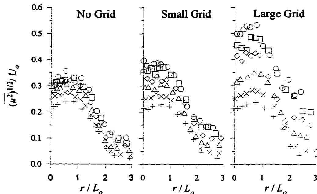
Figure 5.13: Streamwise turbulent velocity profiles for the small jet with VR \approx 6 normalized by U_o . x (cm): +, 10; x, 20; \Delta , 40; \diamond , 60; \square , 80; \circ , 100. (x-x_o)/\theta : +, 3.3; x, 7.3; \Delta , 15.2; \diamond , 23.4; \square , 32.4; \circ , 40.7.
