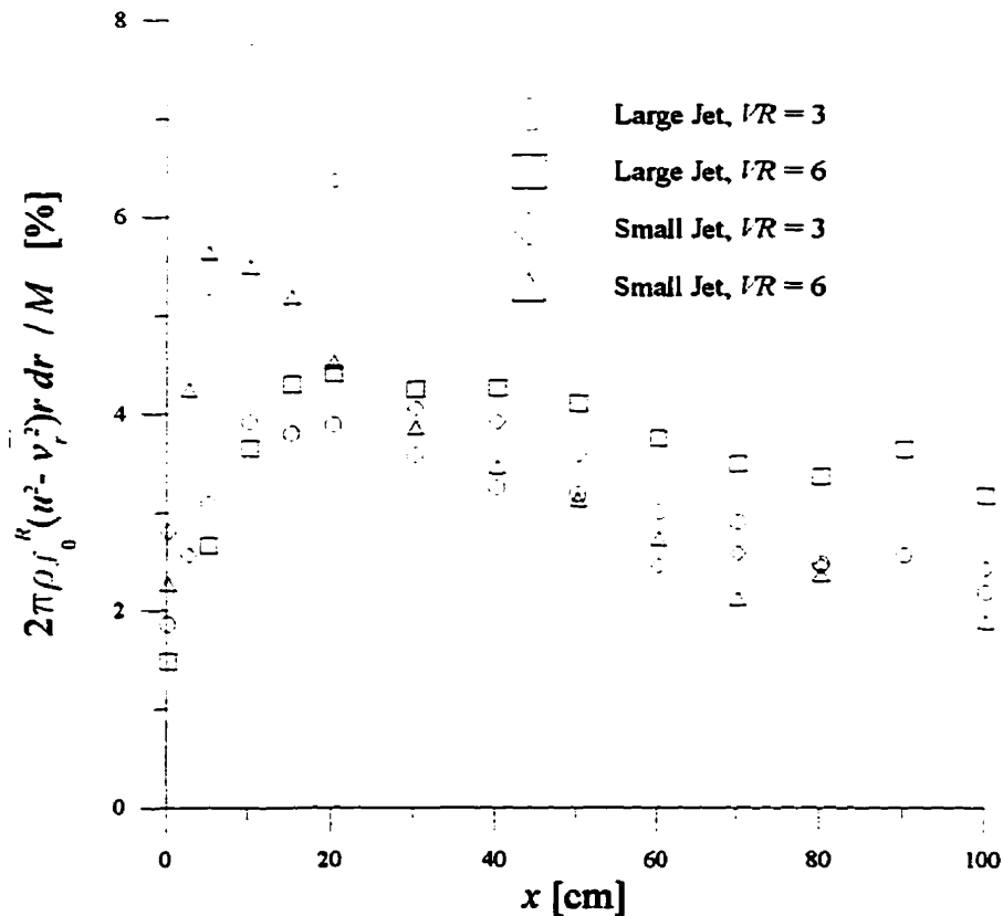
Figure 3.6: Percent contribution of the (\overline{u'^2} - \overline{v'^2}) term in the momentum integral (equation 3.3) to the total momentum for jets in a low turbulent coflow.
