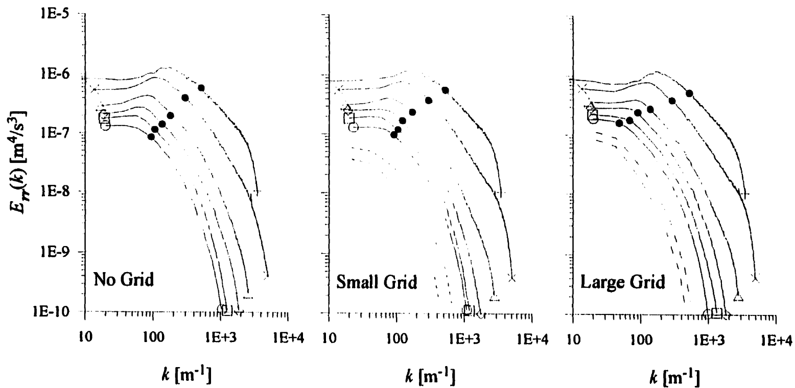
Figure 5.47: Average radial turbulent energy spectra for the small jet at VR \approx 6 . x (cm): + , 10; \times , 20; \Delta , 40; \diamond , 60; \square , 80; \circ , 100. (x-x_o)/\theta : + , 3.3; \times , 7.3; \Delta , 15.2; \diamond , 23.4; \square , 32.4; \circ , 40.7. External spectra range: - - -, small grid; - · -, large grid. Solid bullets, \bullet , give approximate locations of L_{rr} on spectra.
