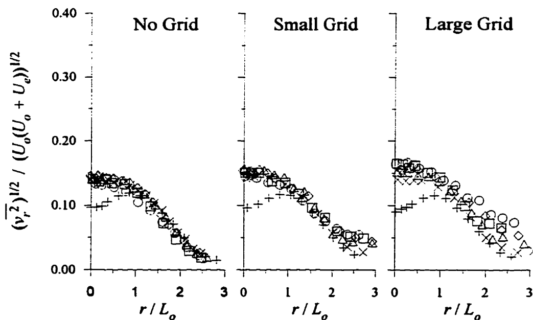
Figure 5.22: Radial turbulent velocity profiles for the large jet with VR \approx 3 normalized by (U_o(U_o+U_e))^{1/2} . x (cm): +, 10; ×, 20; Δ, 40; ◇, 60; □, 80; ○, 100. (x-x_o)/\theta : +, 4.6; ×, 8.1; Δ, 15.2; ◇, 22.2; □, 29.2; ○, 36.2.
