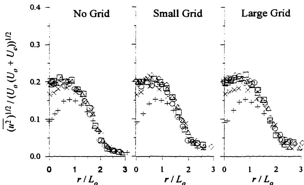
Figure 5.10: Streamwise turbulent velocity profiles for the large jet with VR \approx 6 normalized by (U_o(U_o+U_e))^{1/2} . x (cm): +, 10; ×, 20; Δ, 40; ◇, 60; □, 80; ○, 100. (x-x_o)/\theta : +, 0.8; ×, 2.3; Δ, 5.2; ◇, 8.6; □, 11.8; ○, 14.8.
