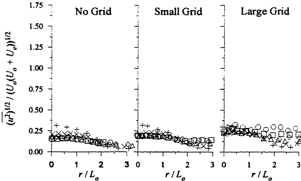
Figure 5.16: Streamwise turbulent velocity profiles for the small jet with VR \approx 3 normalized by (U_o(U_o + U_o))^{1/2} . x (cm): +, 10; ×, 20; Δ, 40; ◇, 60; □, 80; ○, 100. (x-x_o)/\theta : +, 9.9; ×, 19.6; Δ, 39.5; ◇, 60.3; □, 81.8; ○, 105.7.
