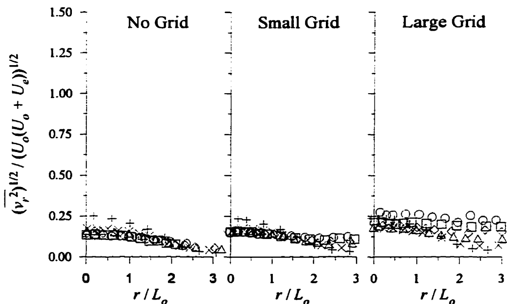
Figure 5.26: Radial turbulent velocity profiles for the small jet with VR \approx 3 normalized by (U_o(U_o + U_e))^{1/2} . x (cm): +, 10; ×, 20; Δ, 40; ◇, 60; □, 80; ○, 100. (x-x_o)/\theta : +, 9.9; ×, 19.6; Δ, 39.5; ◇, 60.3; □, 81.8; ○, 105.7.
