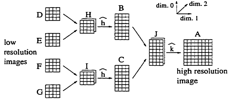
Figure 5.2: Wavelet reconstruction.
