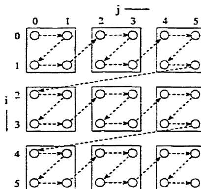
Figure 7.6: Iteration-space traversal of a tiled loop nest.
