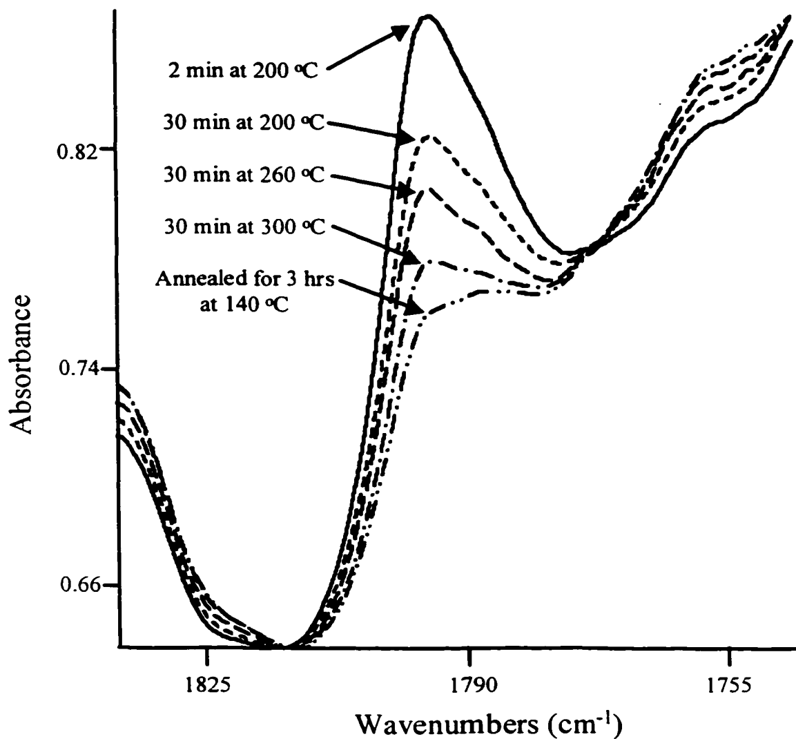
Figure 5.10. FT-IR Spectra of the Model Interfacial Reaction Between the Polymer Tracers in Molten PP at Different Temperatures to Investigate the Possibility of a Reverse Reaction
