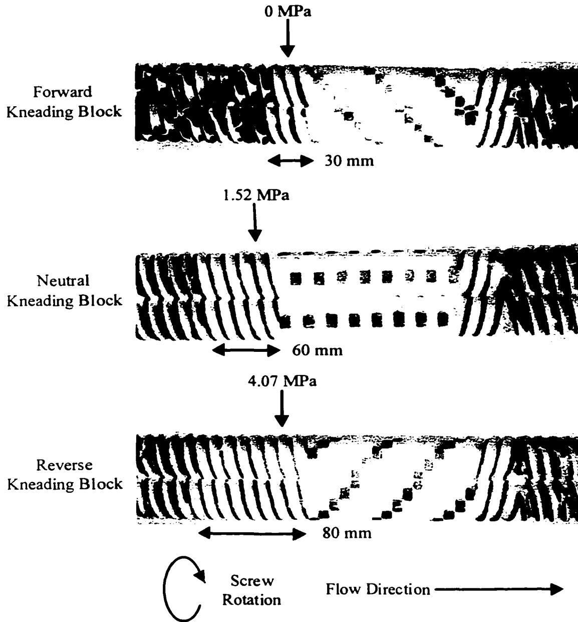
Figure 7.9. Fill Distribution in the Conveying Section and the Kneading Block at 100 g/min and 100 rpm
