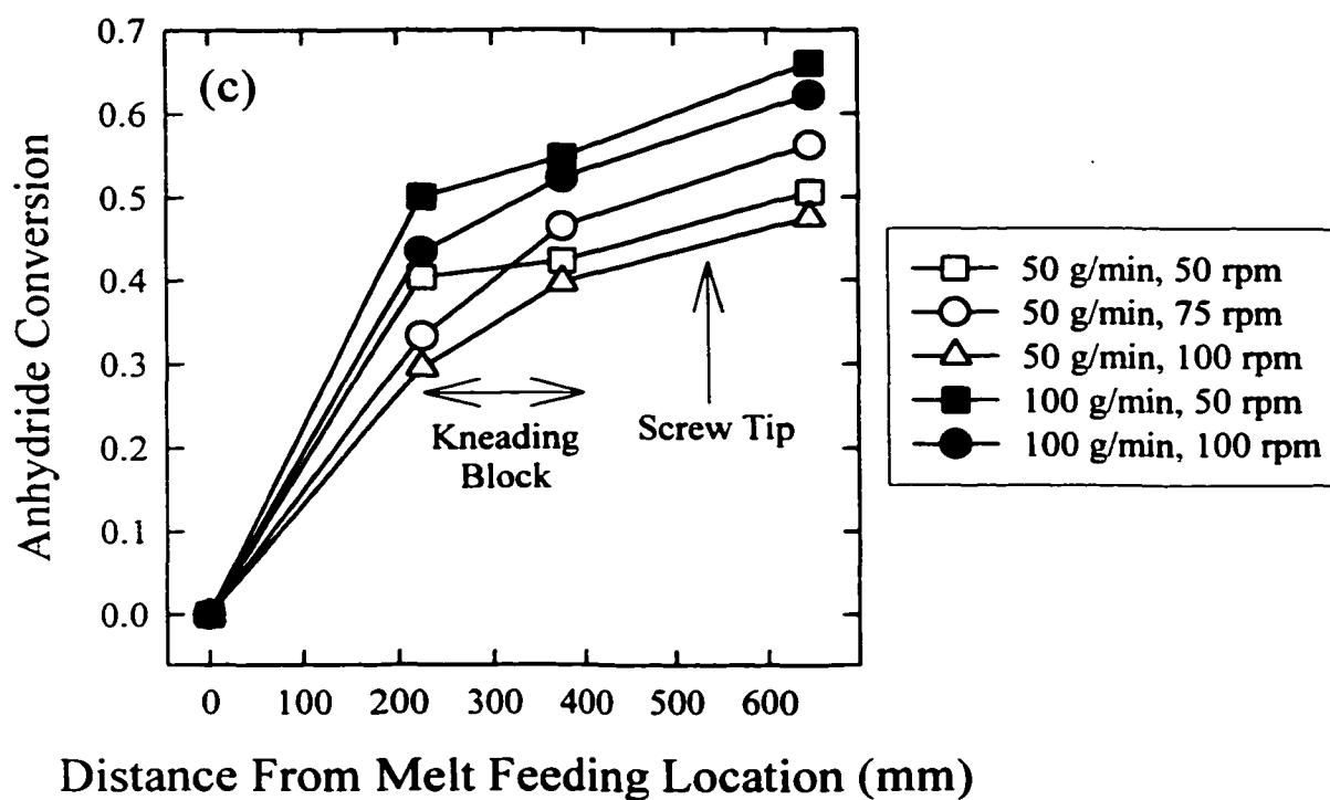
Figure 7.2. Distributive Mixing Profile Along the Length of the Melt-melt Blending Section of the Twin Screw Extruder
