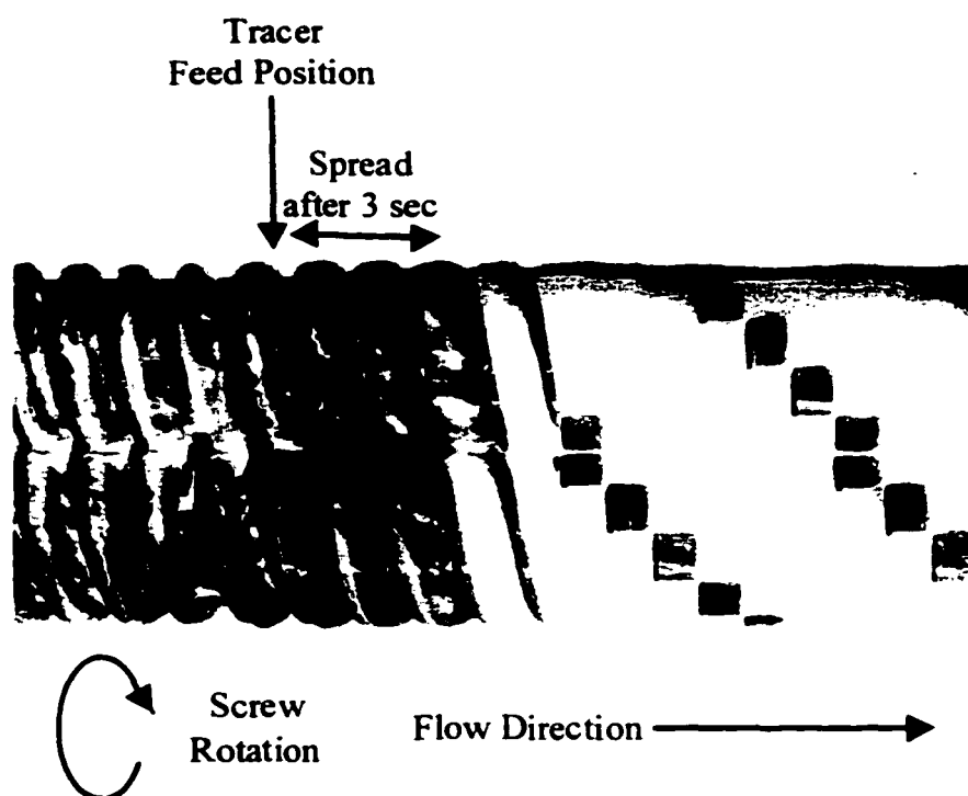
Figure 7.15. Photograph of the Pulse of the Carbon Black Tracer Shortly After its Addition to the Twin Screw Extruder (0.5wt% \text{TiO}_2 Added to the PP to Increase the Contrast)
