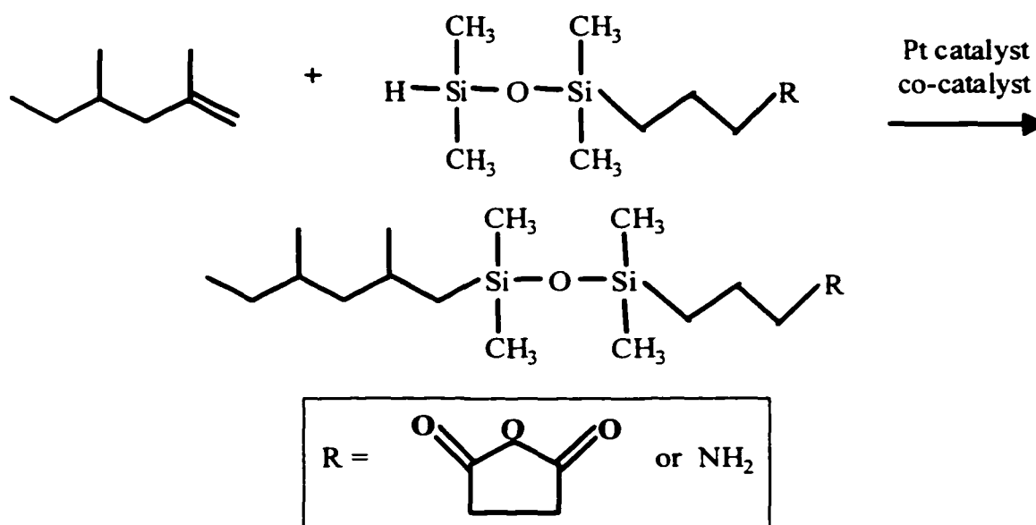
Figure 3.16. Possible Functionalization Method to Introduce Primary Amines and Anhydrides to Unsaturated Polymers Via Hydrosilylation
