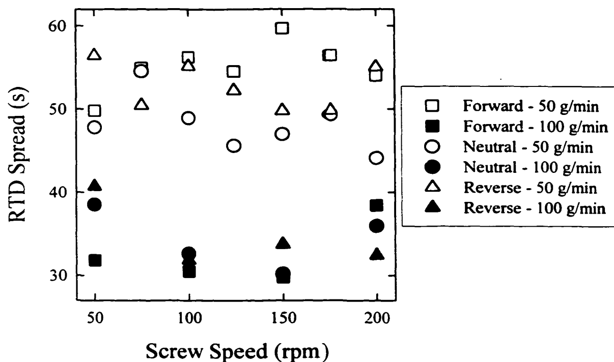
Figure 6.12. RTD Spread Results for all Three Screw Configurations
