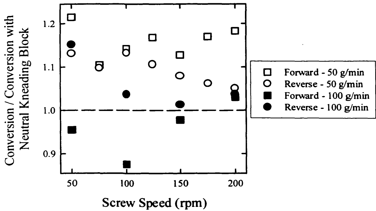
Figure 6.5. Relative Mixing Performances Using the Results from the Screw Configuration with the Neutral Kneading Block as a Basis
