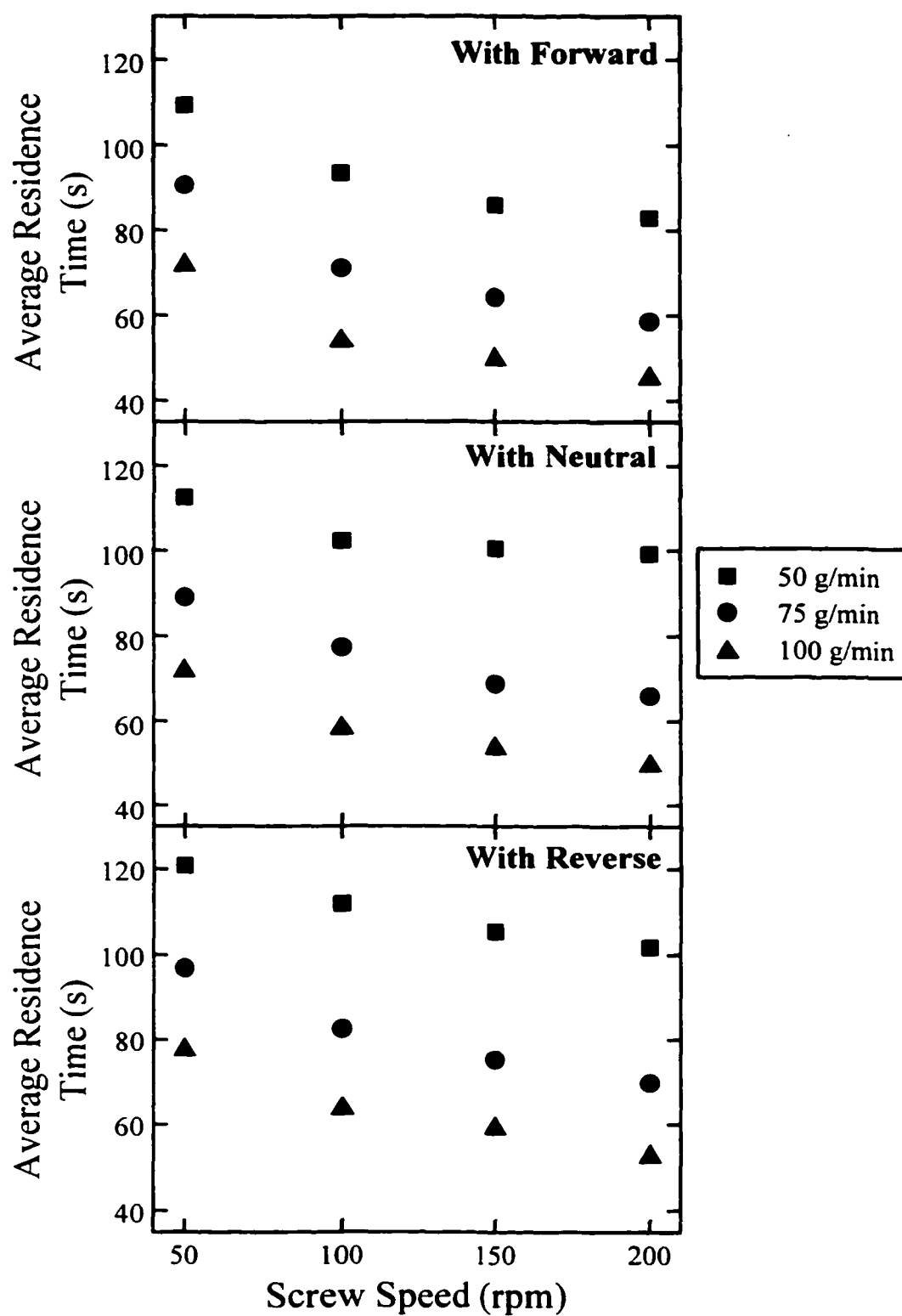
Figure 7.18. Local Residence Time In the Combination of the Conveying Section and the Kneading Block
