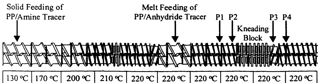
Figure 4.4. Example of Screw Configuration for Melt-melt Blending
