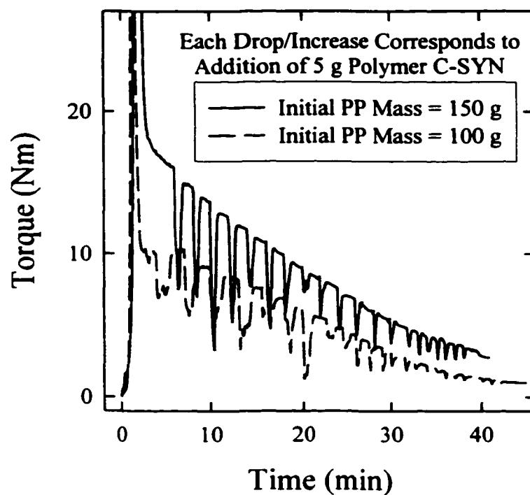
Figure 5.2. Torque Plots from the Blending of Polymer C-SYN and Petrothene PP in the Batch Mixer
