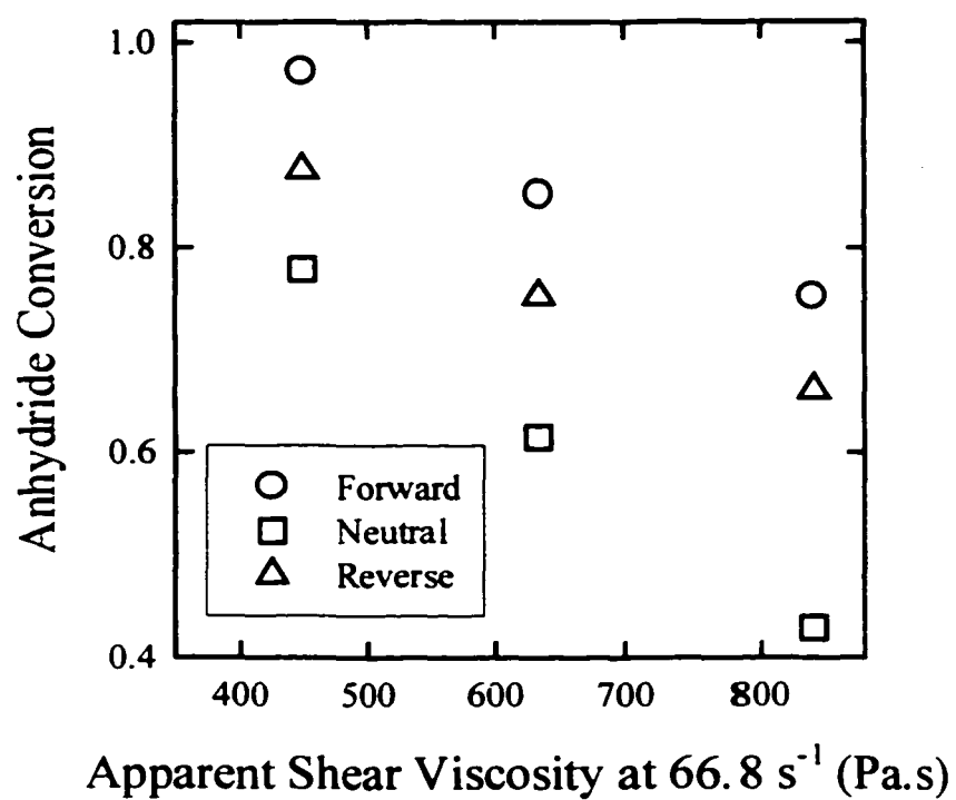
Figure 5.16. Relationships Between Mixing Performance and Polymer Viscosity
