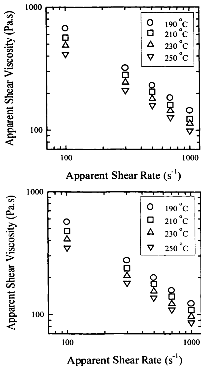
Figure 5.11. Apparent Shear Viscosity Results (Top) Pure KF6100 PP (Bottom) KF6100 PP + 5wt% Polymer C-SYN
