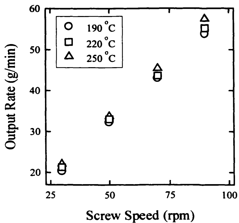
Figure 4.6. Example of Single Screw / Adapter Output Curve for KF6100 PP with 5wt% Polymer C-SYN
