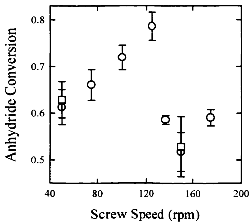
Figure 5.13. Screw Speed Effect on Mixing During Polymer Melt-melt Blending
