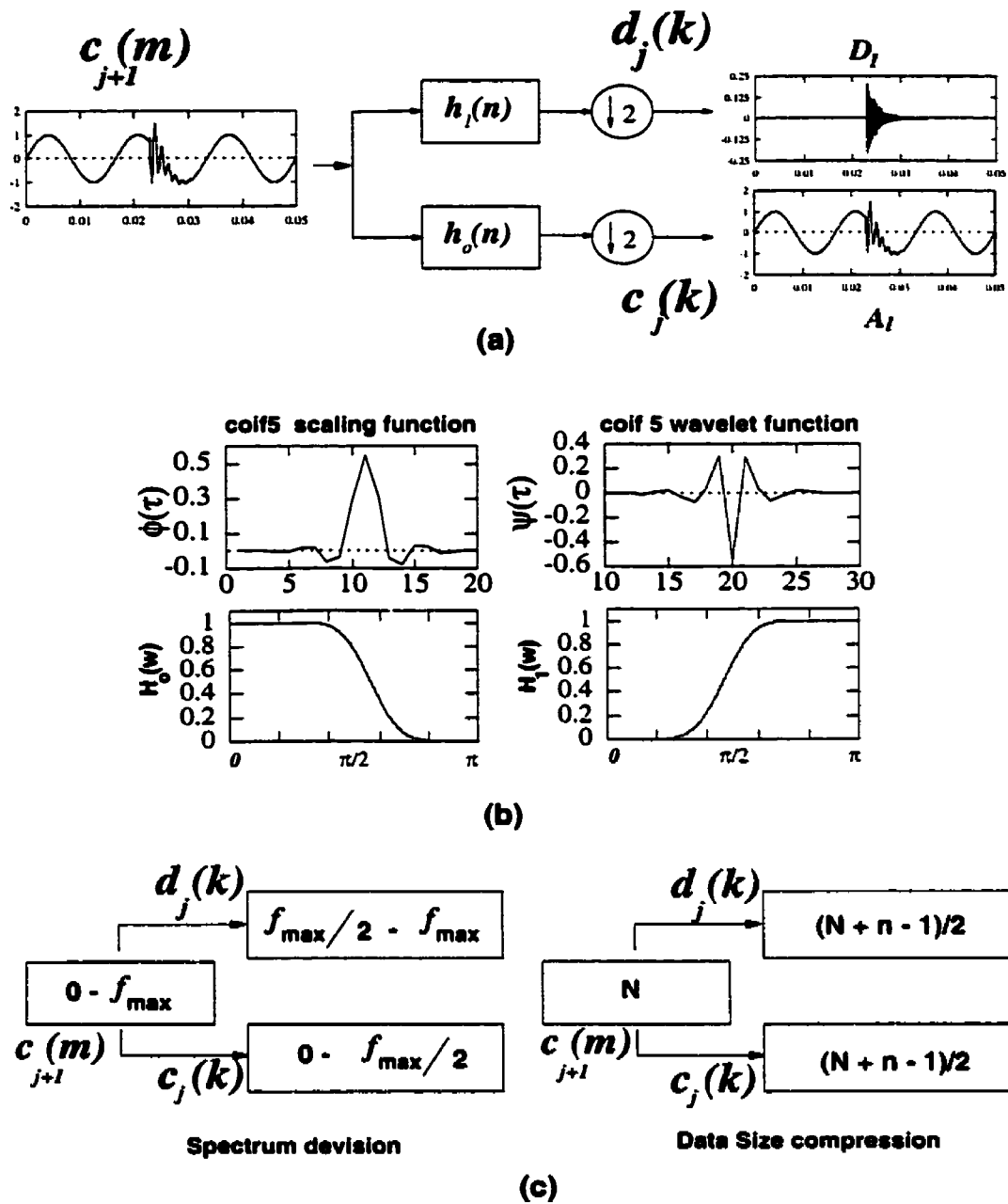
Figure 4.8: One stage of MRA and wavelet filters
