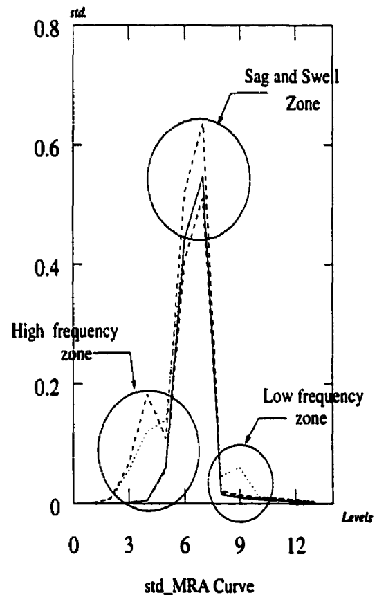
Figure 6.8: std-MRA curve for different Power quality problems.
