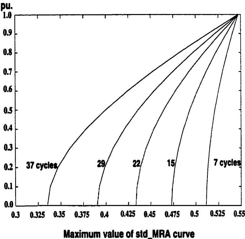
Figure 7.2: The variation of signal magnitude during different sag intervals with the changes in the maximum value of the std-MRA curve
