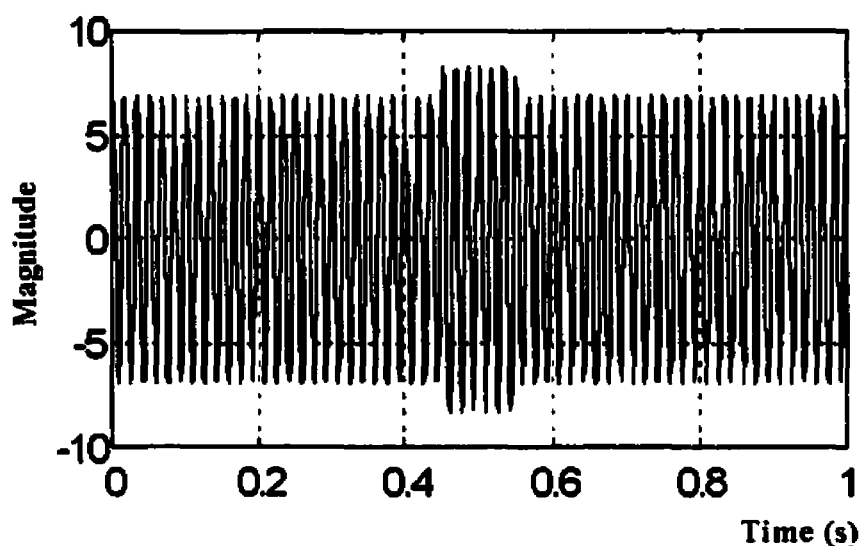
Figure 2.5: Voltage swell
