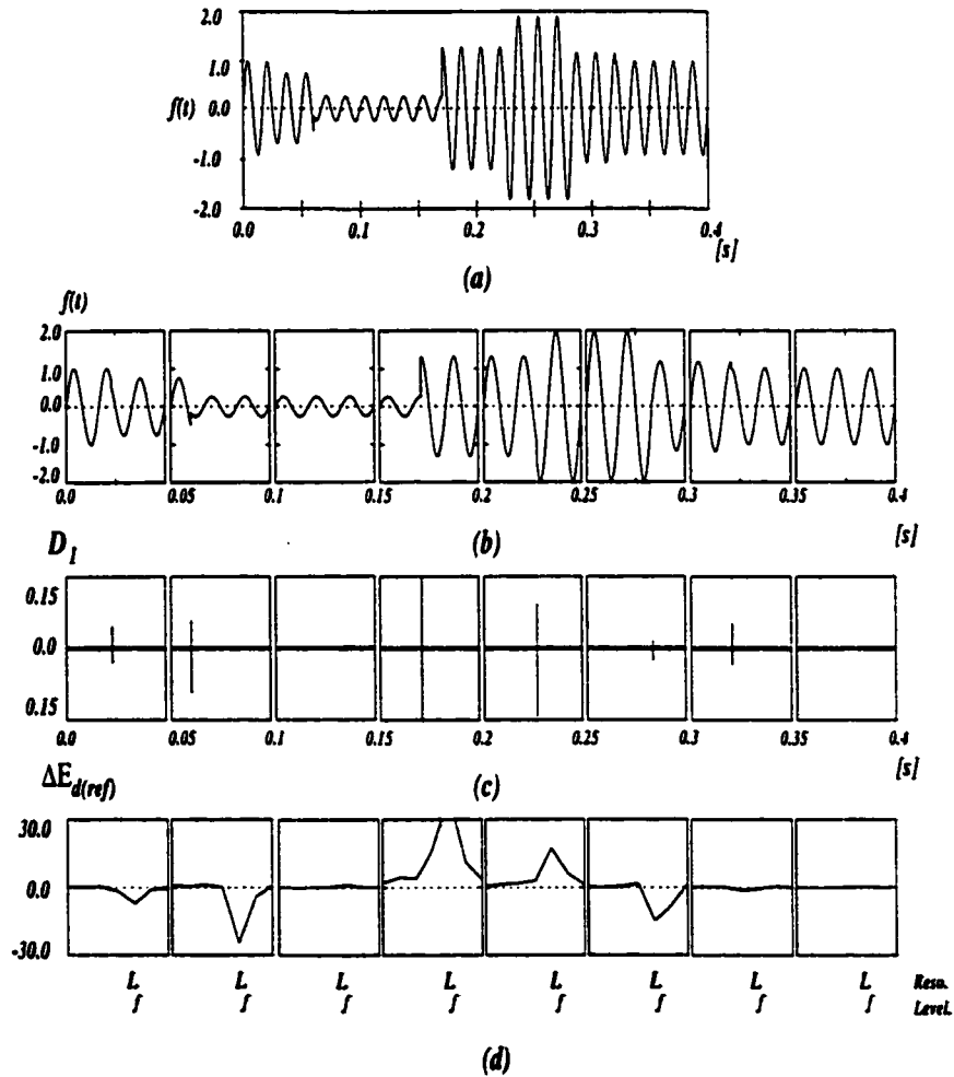
Figure 7.4: RMS variation monitoring
