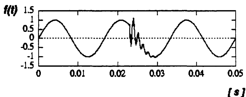
Figure 8.3: Distorted Signal with a capacitor switching phenomena
