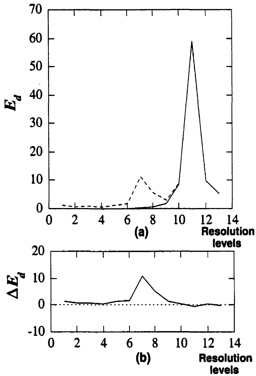
Figure 6.16: Distribution of energy of the signal at different resolution levels
