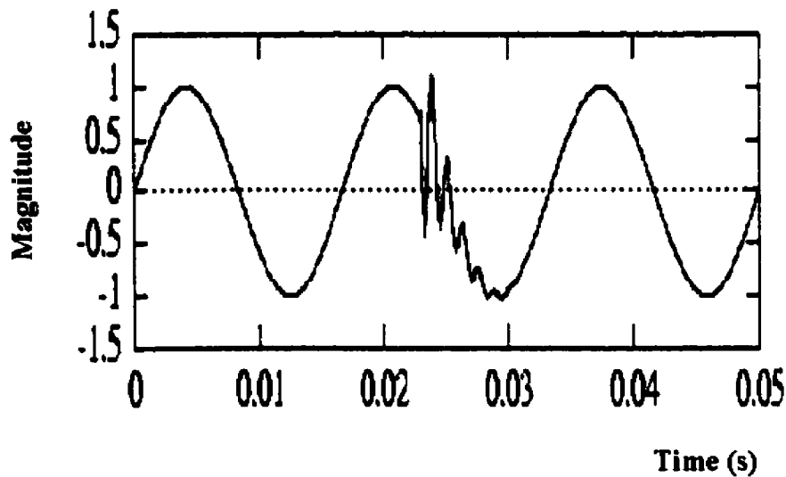
Figure 2.11: Capacitor switching phenomena
