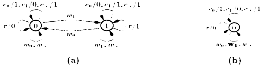
Figure 7.8: Cell behavior: (a) correct, (b) s -sa-0.
