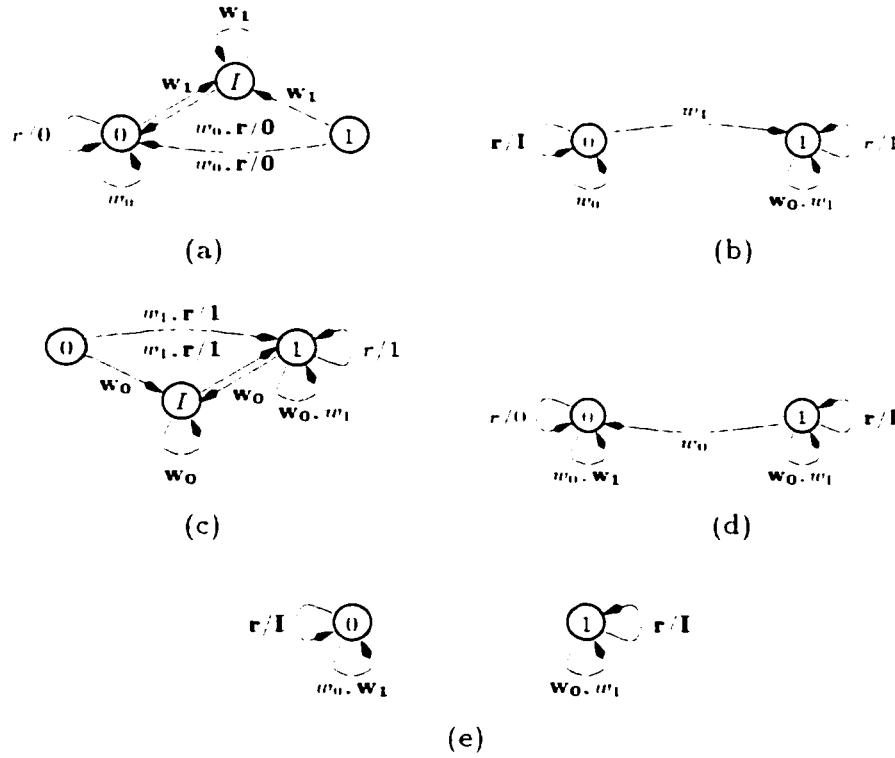
Figure 10.3: Faulty behaviors of an SRAM cell: (a) b\text{-}sa\text{-}0 , (b) b\text{-}sa\text{-}1 , (c) \bar{b}\text{-}sa\text{-}0 , (d) \bar{b}\text{-}sa\text{-}1 , (e) w\text{-}sa\text{-}0 .
