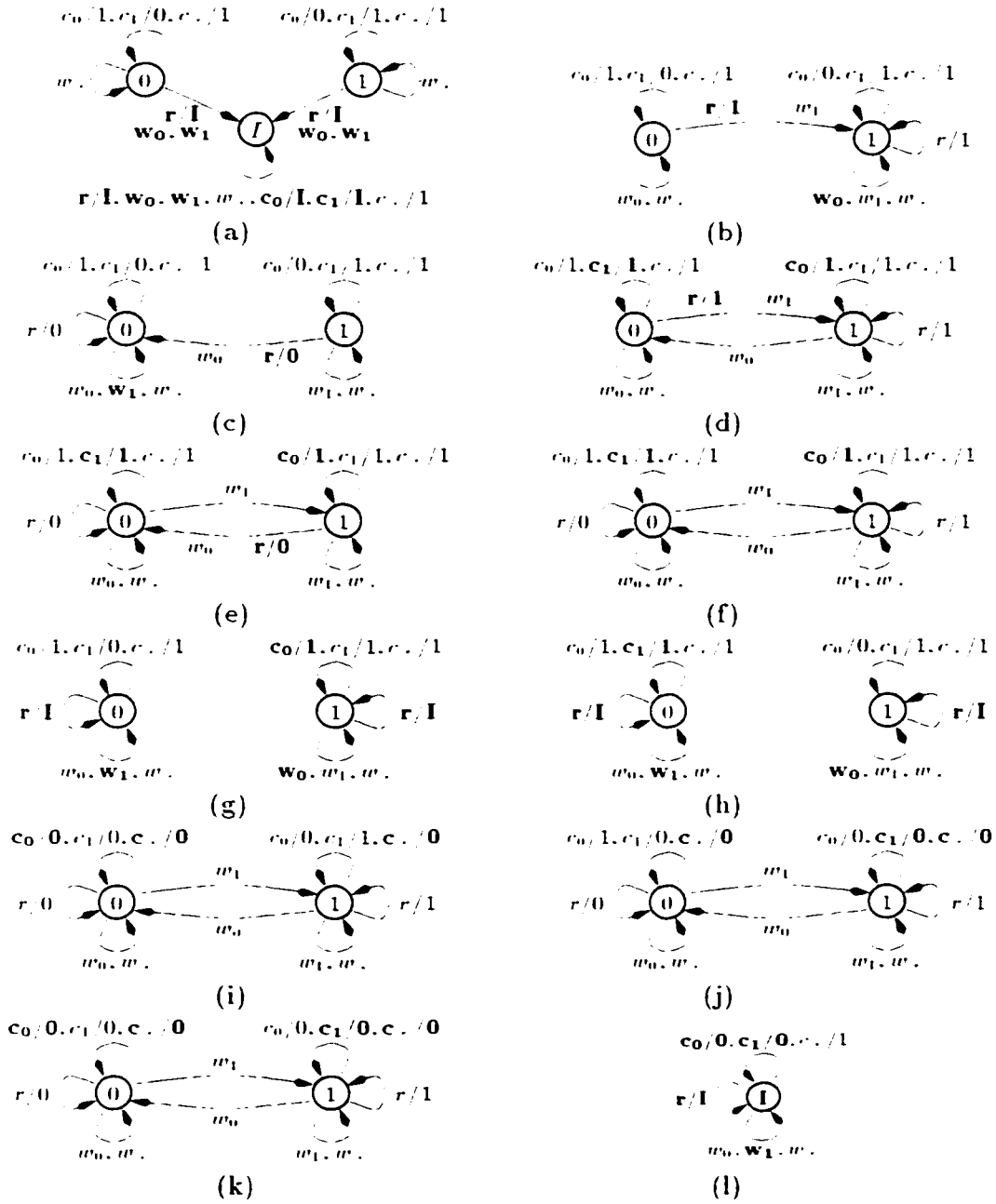
Figure 7.15: FSM models for faults: (a) b\text{-}\bar{b}\text{-hrd} , (b) b\text{-}w\text{-hrd} , (c) \bar{b}\text{-hrd} , (d) b\text{-}m\text{-hrd} , (e) \bar{b}\text{-}m\text{-hrd} , (f) c\text{-}\bar{c}\text{-hrd} , (g) c\text{-}w\text{-hrd} , (h) \bar{c}\text{-}w\text{-hrd} , (i) c\text{-}m\text{-hrd} and c\text{-}m\text{-res} , (j) \bar{c}\text{-}m\text{-hrd} and \bar{c}\text{-}m\text{-res} , (k) m\text{-}w\text{-hrd} and m\text{-}w\text{-res} , (l) s\text{-}\bar{s}\text{-hrd} .
