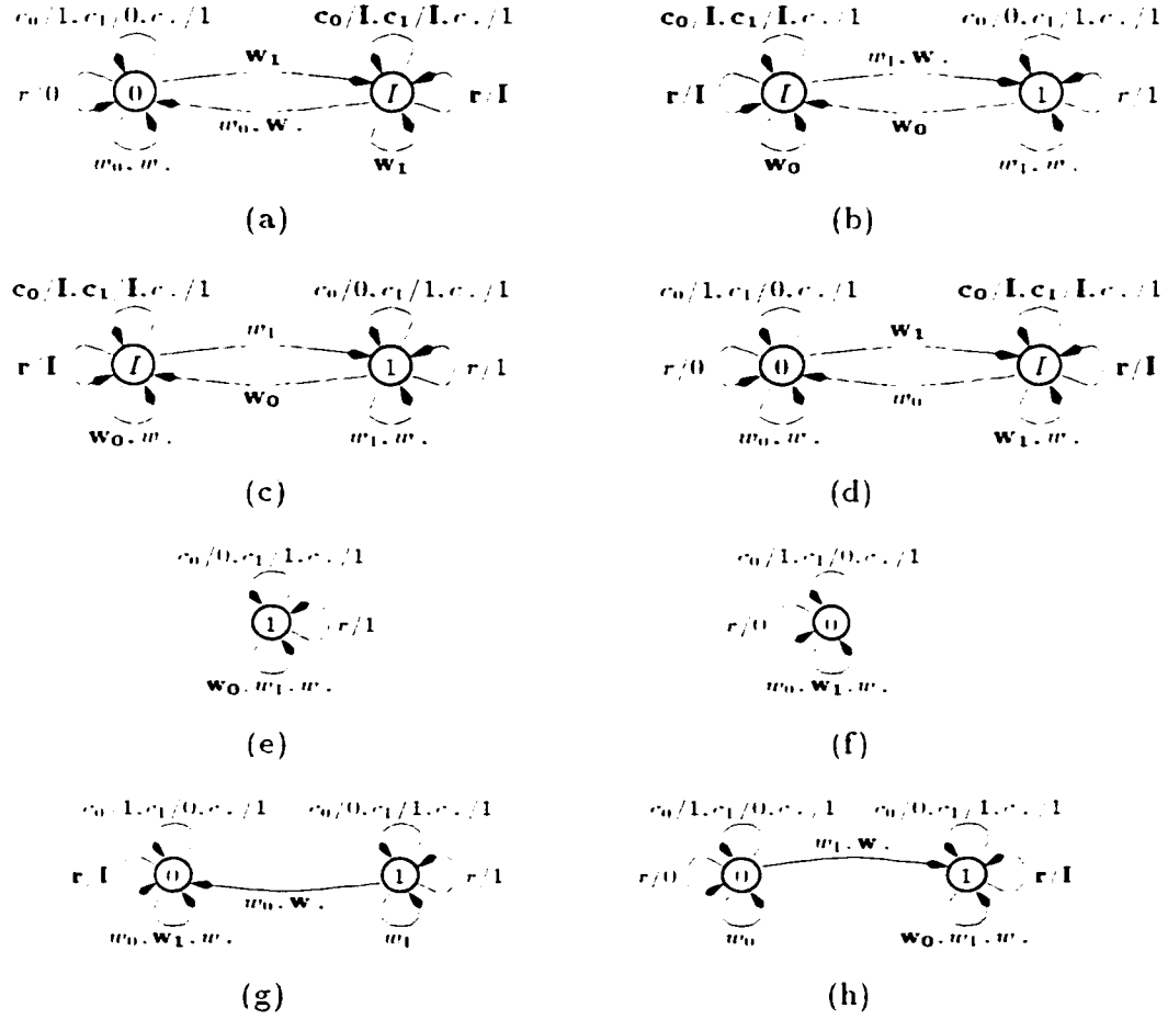
Figure 7.11: FSM models for faults: (a) T_1 -on, T_2 -open and T_3 -open, (b) T_1 -open, T_2 -on and T_3 -on, (c) T_3 -on, (d) T_4 -on, (e) T_5 -on, (f) T_6 -on, (g) T_5 -open, (h) T_6 -open.
