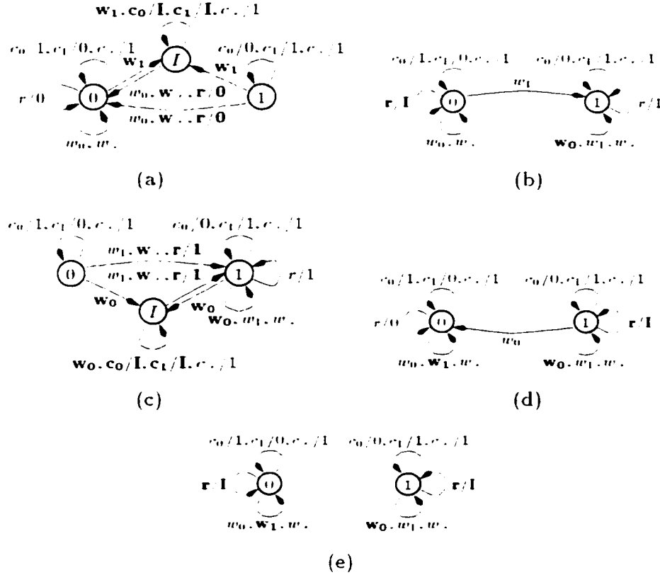
Figure 7.6: FSM models for faults: (a) b-sa-0 , (b) b-sa-1 , (c) b̄-sa-0 , (d) b̄-sa-1 , (e) w-sa-0 .
