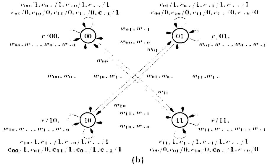
Figure 7.14: Behavior of two adjacent CAM cells: (a) correct. (b) \bar{c}' -c-hrd.
