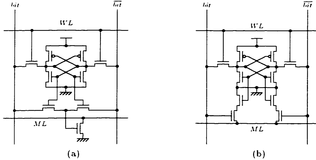
Figure 5.2: CMOS implementations of a single-port static CAM cell.
