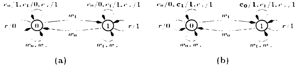
Figure 7.13: Cell behavior: (a) correct, (b) c\text{-}\bar{c}\text{-hrd} .
