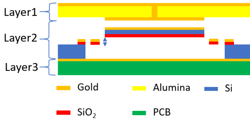
Figure 3.15: Cross-section of a mechanically tunable reflectarray.
