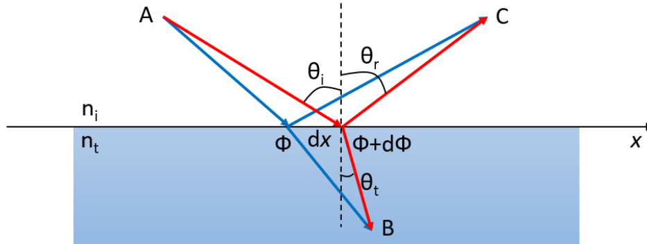
Figure 2.13: Schematic diagram of generalized Snell's Law based on Fermat's principle[61]
