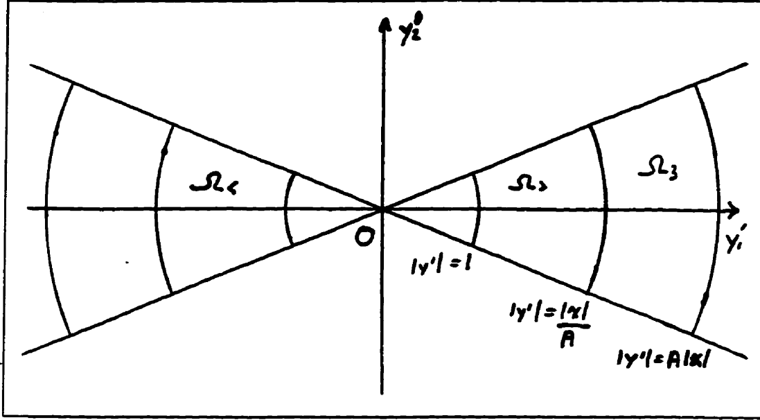
Figure 3.1: The regions \Omega_2 , \Omega_3 and \Omega_4
