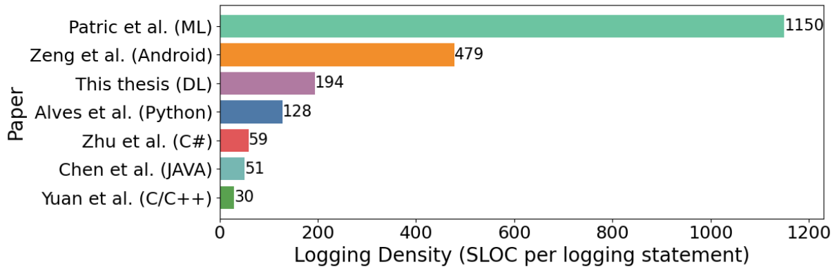
Figure 4.3: Distribution of logging density across different systems.
