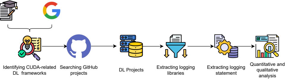
Figure 3.1: Overview of our research workflow.
