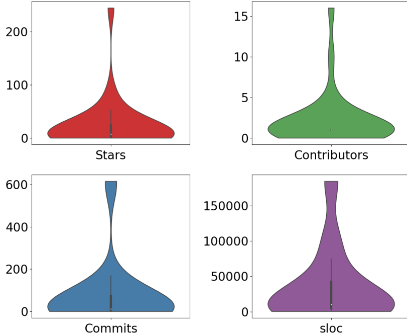
Figure 4.1: Distribution of selected deep learning projects across metrics
