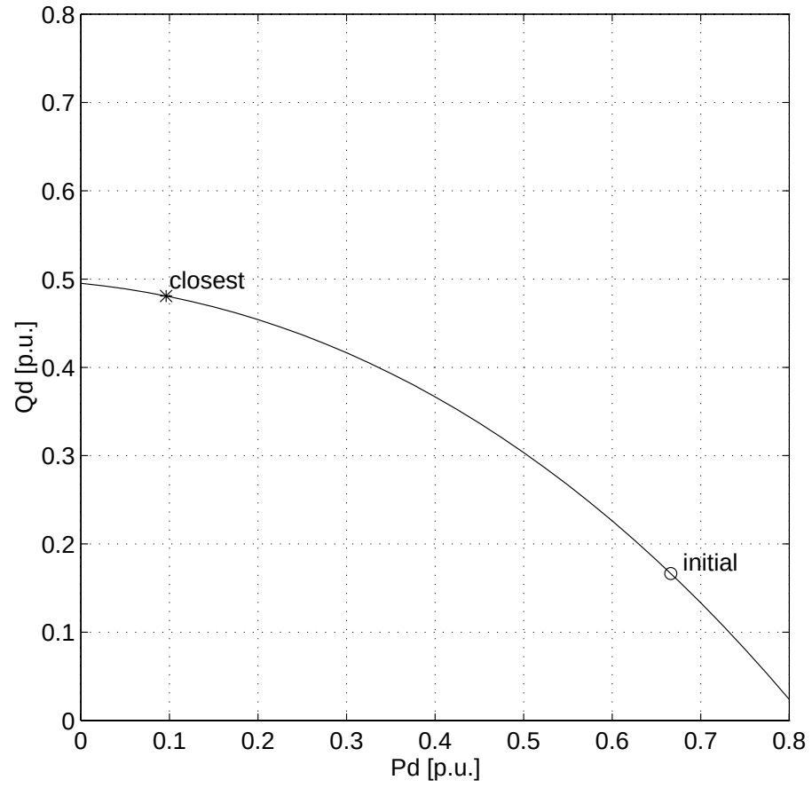
Fig. 3. Hypersurface of saddle-node bifurcations when \lambda = [P_d \ Q_d]^T .
