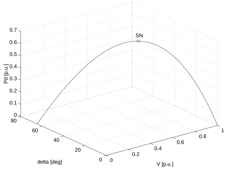
Fig. 2. Bifurcation manifold in state-parameter space when \lambda = P_d . SN stands for the saddle-node bifurcation point.
