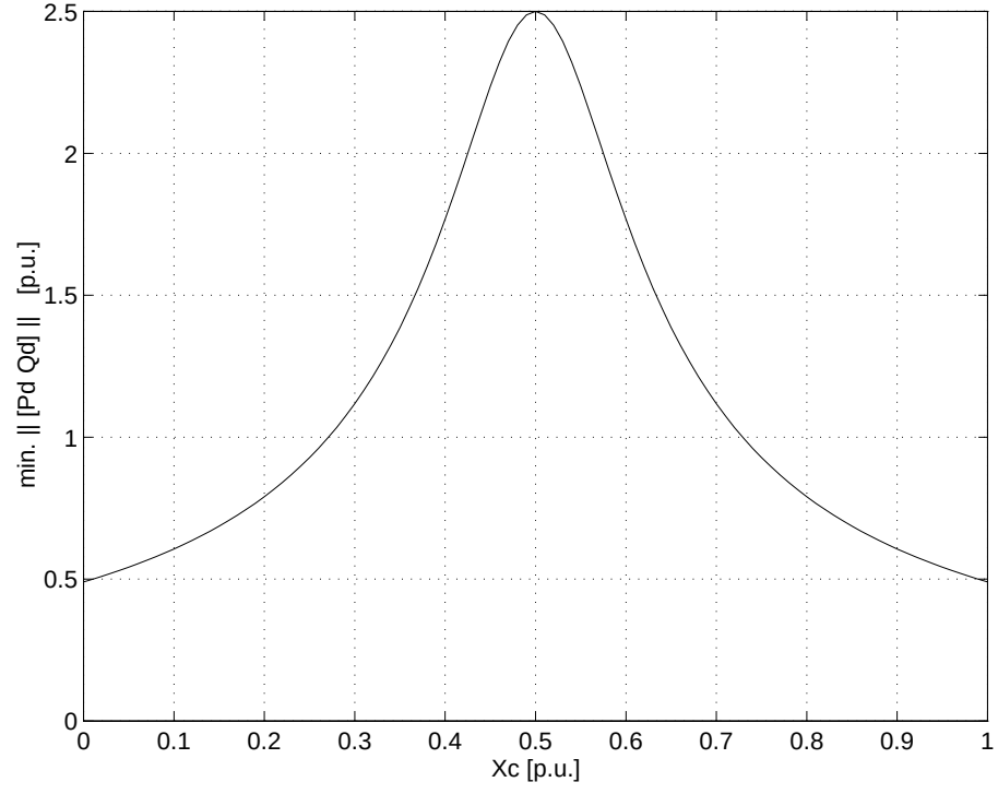
Fig. 7. Minimum \|\lambda\|_2 as series X_C compensation changes.
