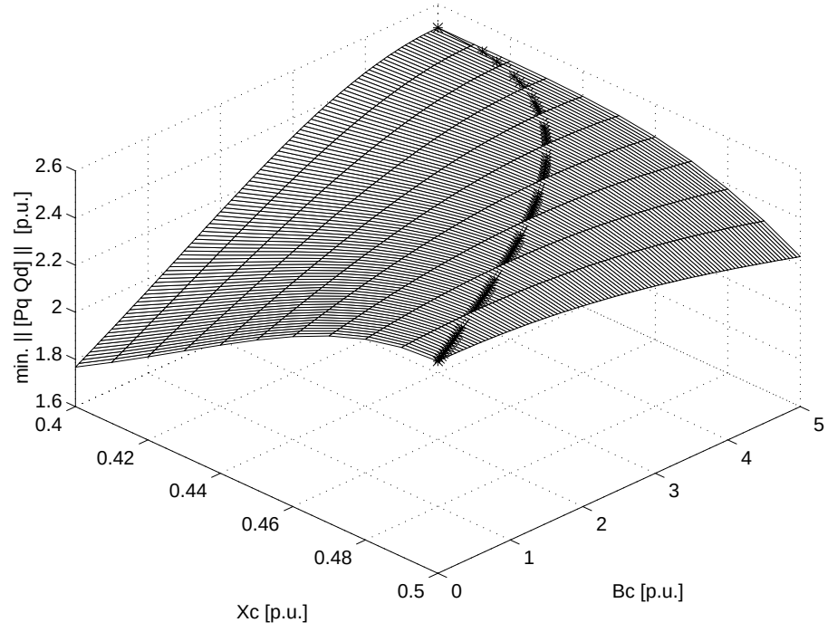
Fig. 9. Minimum \|\lambda\|_2 as series X_C and shunt B_C compensation changes. Optimal closest bifurcation points are marked with *.
