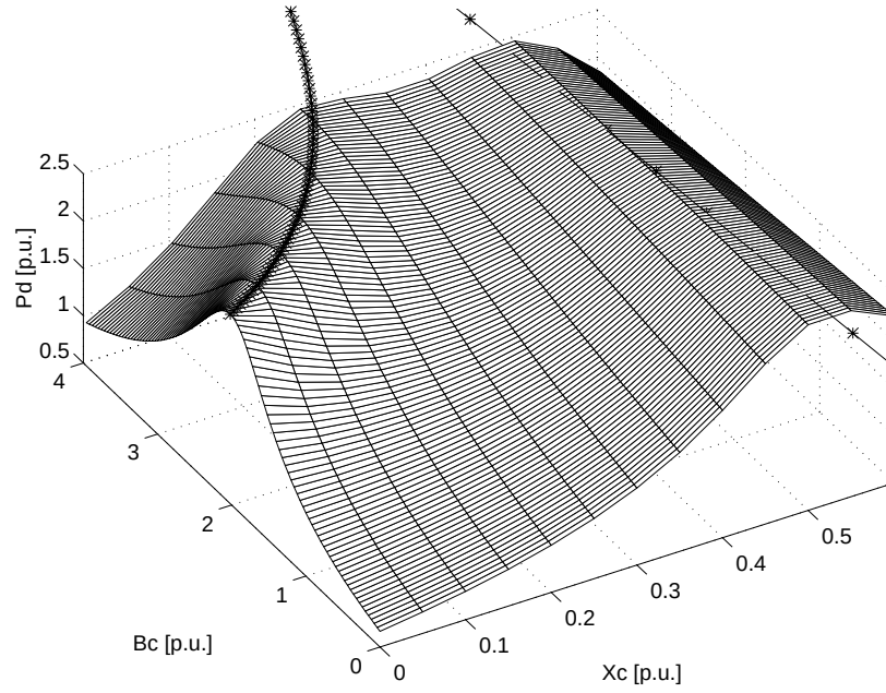
Fig. 8. Hypersurface of saddle-node bifurcations in parameter space. Optimal bifurcations are marked with *.
