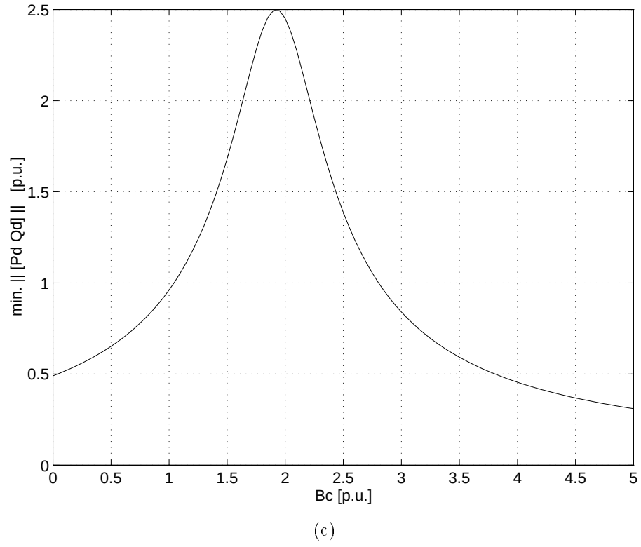
Fig. 5. Saddle-node bifurcation hypersurfaces for \lambda = [P_d \ Q_d]^T with shunt B_C compensation changes: (a) Bifurcation points in parameter space with closest bifurcations marked with *; (b) bifurcation points in \lambda space with closest bifurcations marked with * for values of B_C from 0 to 1.6 p.u.; (c) minimum value of \|\lambda\|_2 (objective function).
