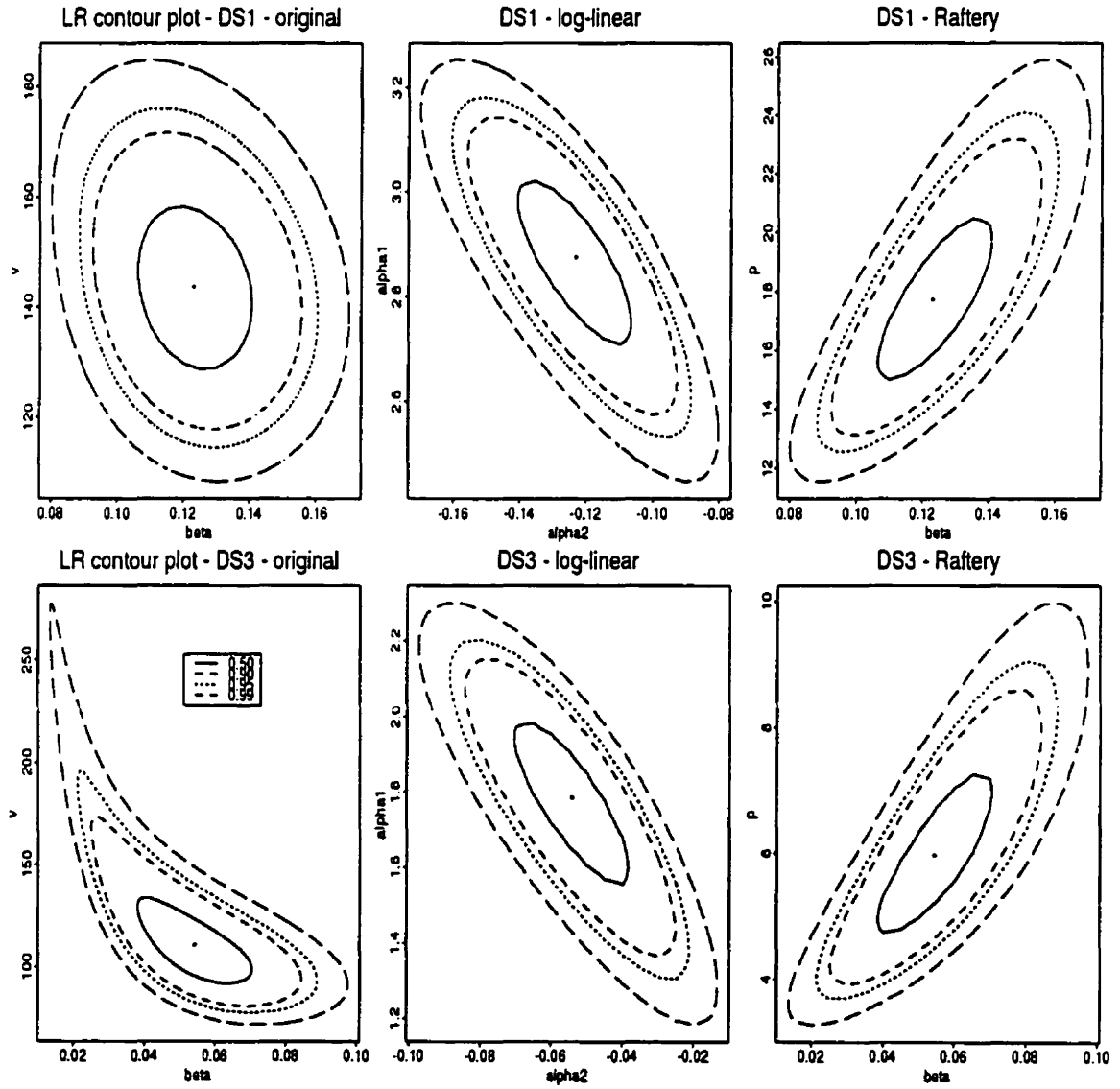
Figure 2.3: LR contour plots using three parameterizations for EOSN and DS1.3.
