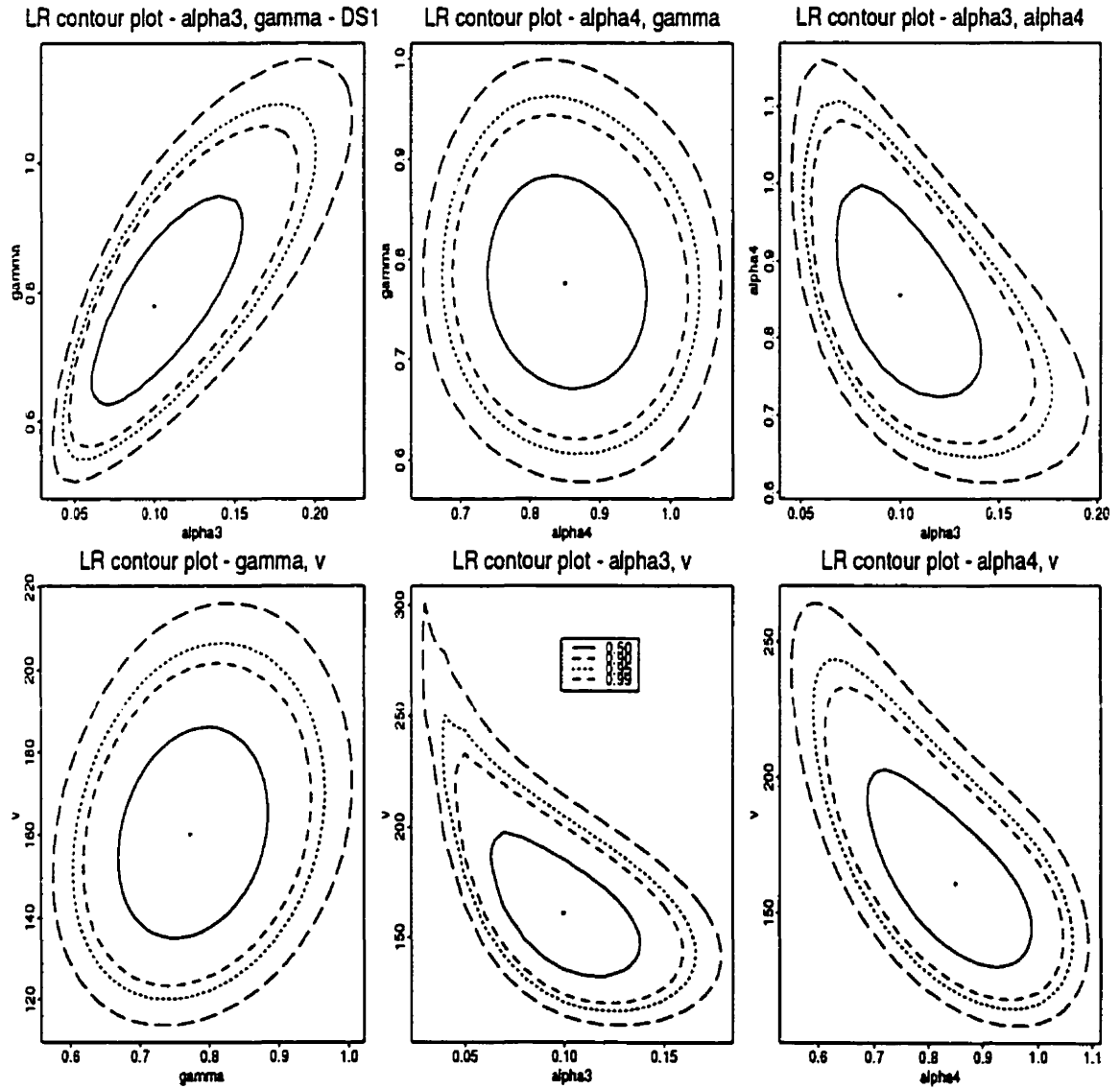
Figure 3.5: Profile LR contour plots of v , \gamma , \alpha_3 , and \alpha_4 for the NEWN model and DS1.
