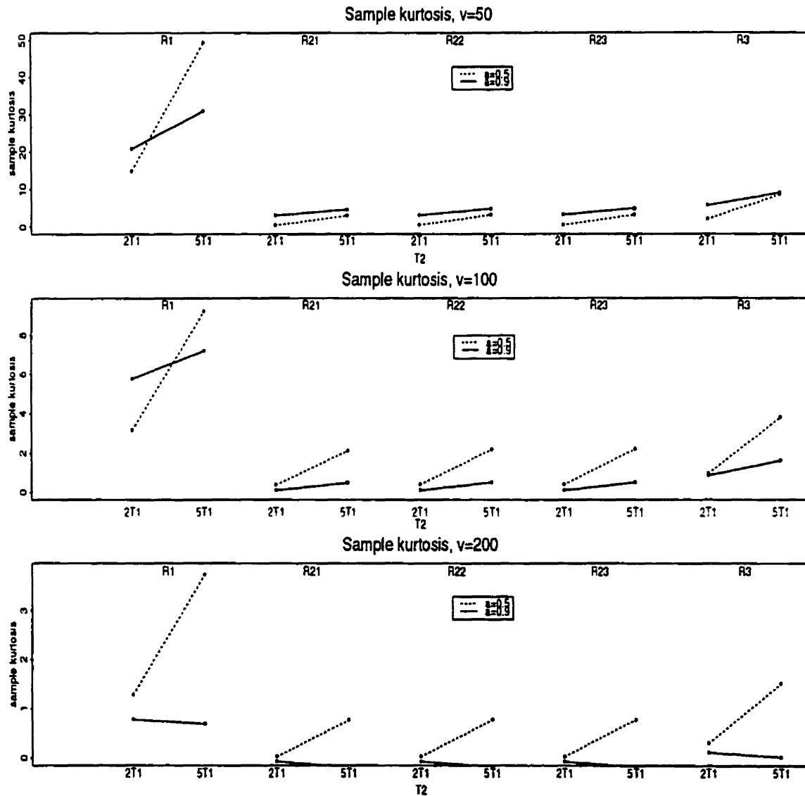
Figure 4.4: Plots of the sample kurtosis ( \hat{\gamma}_2 ) as T_2 increases from 2 \cdot T_1 to 5 \cdot T_1 and v increases from 50 to 200 for one set of bootstrap distributions based on EOSN.
