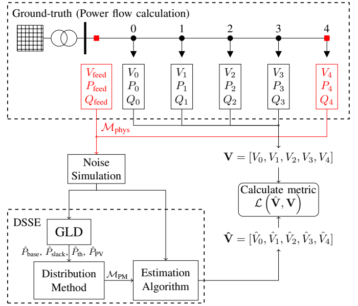
Fig. 8: Evaluation procedure for the accuracy of DSSE algorithms using power flow calculation as ground-truth, with assumed physical measurements marked as ■.
