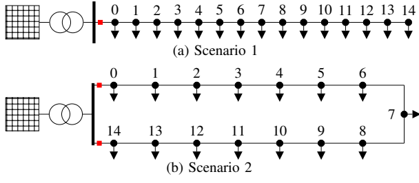
Fig. 7: Considered LV feeder scenarios.
