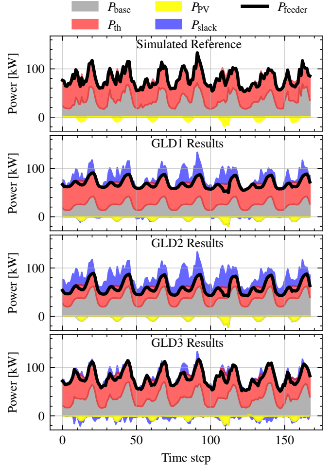
Fig. 10: Disaggregated components for one week of data for GLD1, GLD2, and GLD3.
