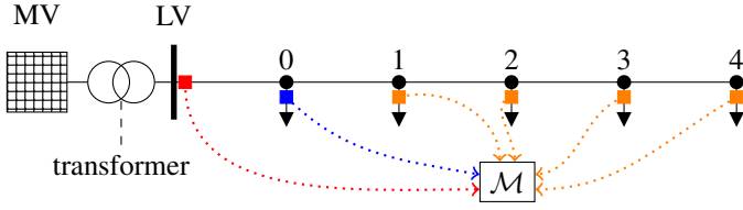
Fig. 2: Exemplary LV feeder measurements, where ■ depicts a feeder measurement, ■ corresponds to an SM measurement, and ■ illustrates a PM.
