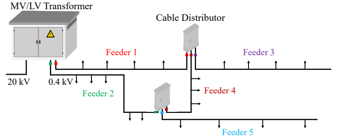
Fig. 1: Schematic of a 400 V LV grid with a 20 kV/400 V transformer supplying multiple buildings through two cable distributors and five feeders.
