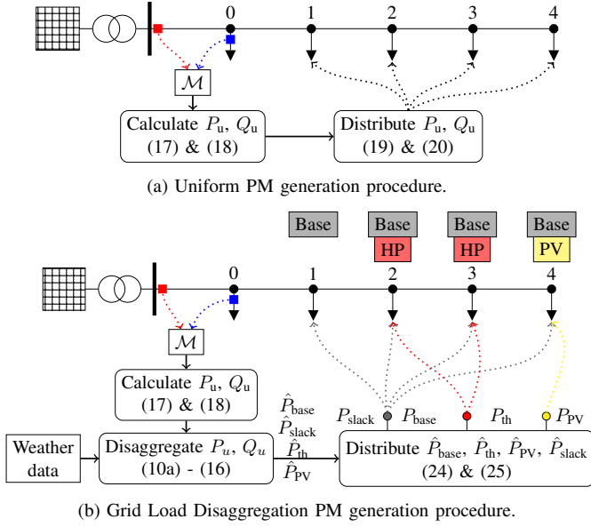
Fig. 6: PM generation with (a) UPM and (b) GLD methods for a sample 5-node radial feeder, with feeder measurements ■, and SM measurements ■.
