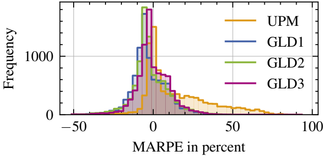
Fig. 13: Histogram of MARPE for household 6 for all methods using the best distribution technique.
