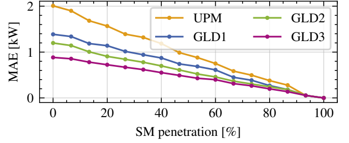
Fig. 12: Error of PM generation techniques for radial feeder and varying SM penetrations for UPM and proposed disaggregation techniques.
