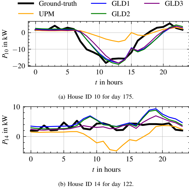
Fig. 11: Ground-truth power injections and PMs using different disaggregation techniques.
