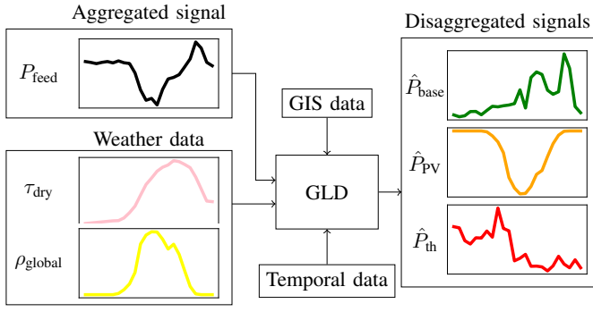
Fig. 4: Schematic of the proposed GLD methodology for disaggregation of LV grid measurements.
