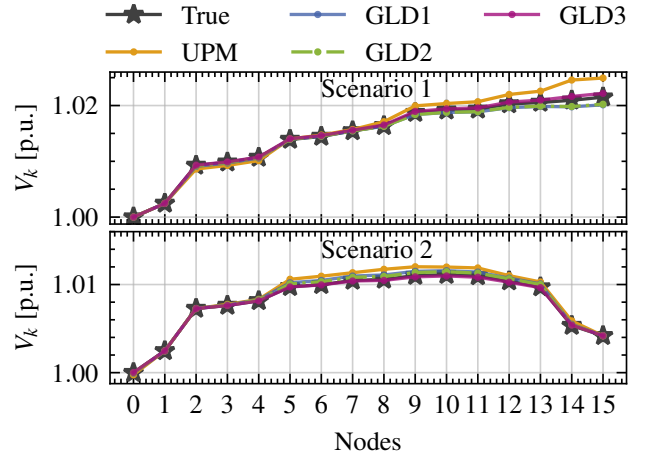
Fig. 14: Voltage estimates for t = 3421 h.
