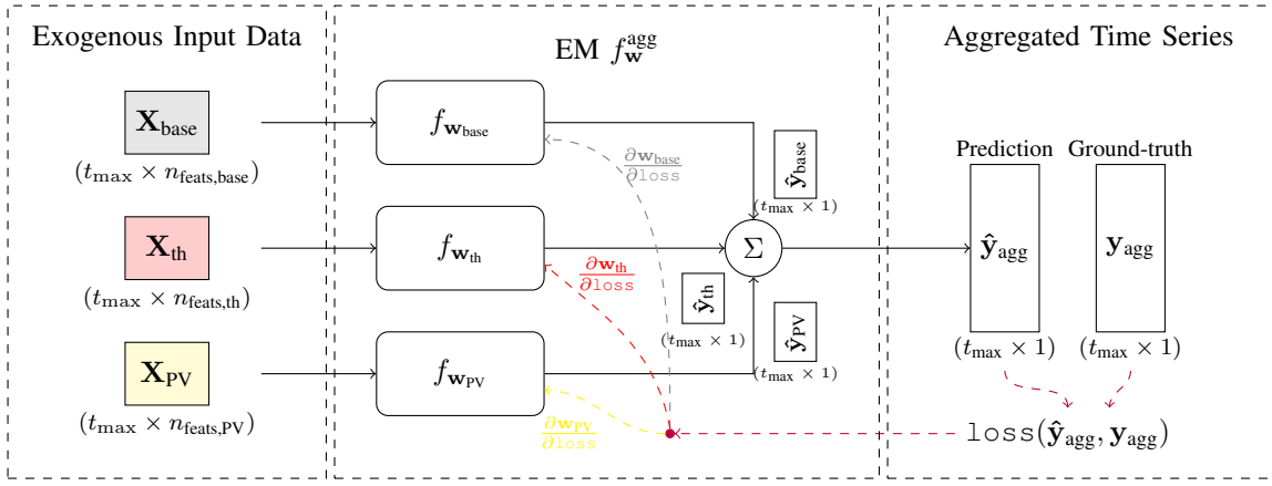
Fig. 5: Data flow in the EM training for GLD.
