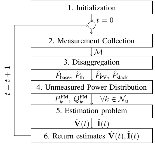
Fig. 3: Flowchart of the proposed multi-timestep DSSE algorithm.
