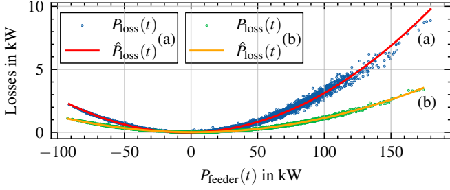
Fig. 9: Losses P_{\text{loss}}(t) for the feeder in (a) Scenario 1 and (b) Scenario 2 with respect to feeder power flows for ground-truth calculations for one year of data and quadratic \hat{P}_{\text{loss}}(t) as per (23).
