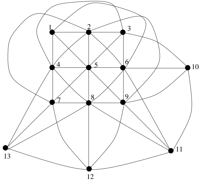
Figure 2.2: Diagram for the projective plane of order 3.
