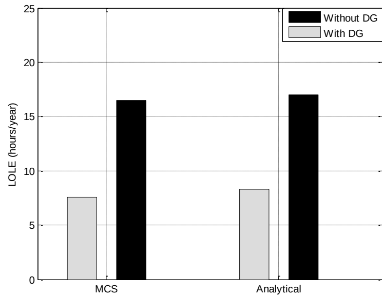
Figure 5-9 Comparison between LOL with and without DG units
