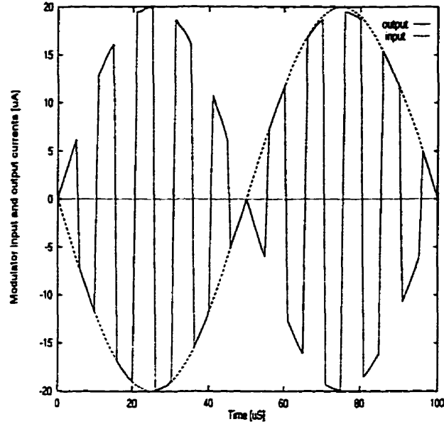
Figure 5.10: Modulator output .
