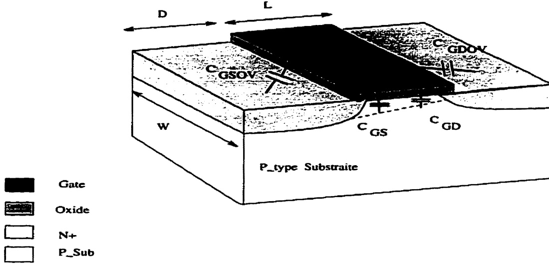
Figure 6.2: The structure of a MOS transistor with its parasitic capacitances.
