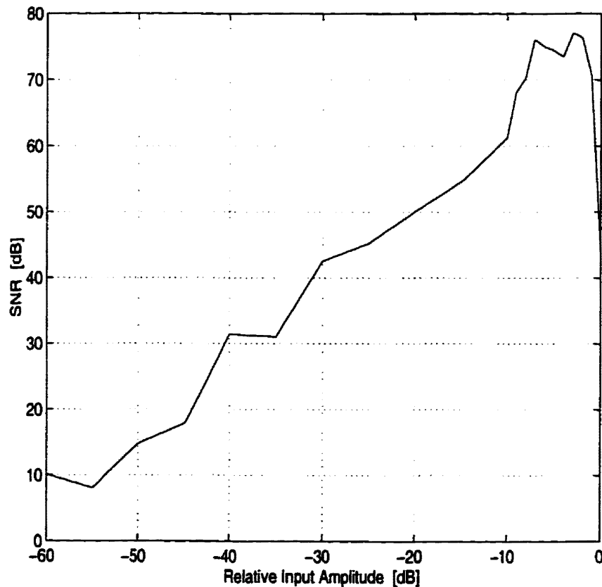
Figure 3.4: Signal to noise ratio vs. input amplitude for the DSM in Fig. 3.2.
