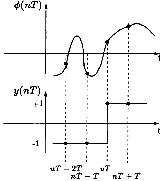
Figure 3.12: The input and output of the clocked comparator.
