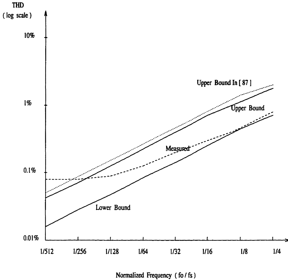
Figure 6.7: Comparing the measured THD of the circuit in Fig.6.1 with results predicted by our method.
