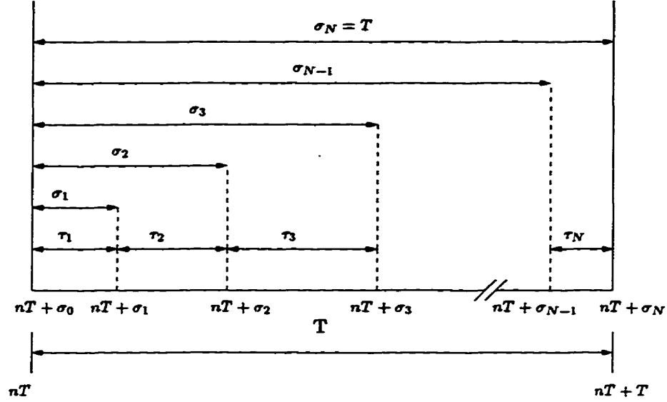
Figure 4.1: Timing definitions for an N-phase switched network.
