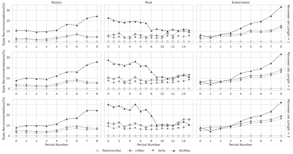
Figure A.1: The proportions of stale to all recommendations (y-axis). The period numbers are normalized, with zero representing the oldest period.
