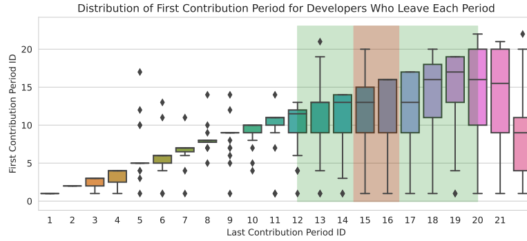
(a) Roslyn
