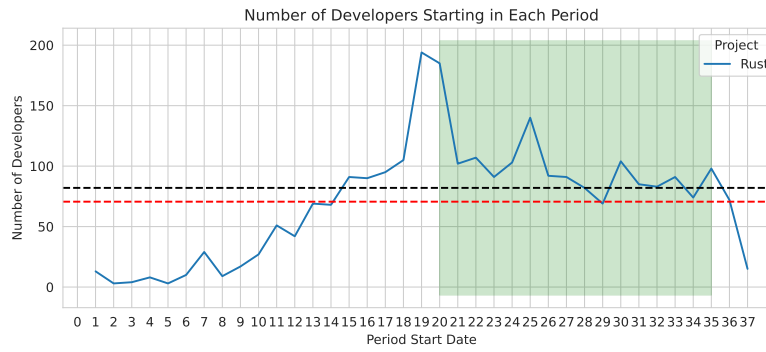
(b) Rust
