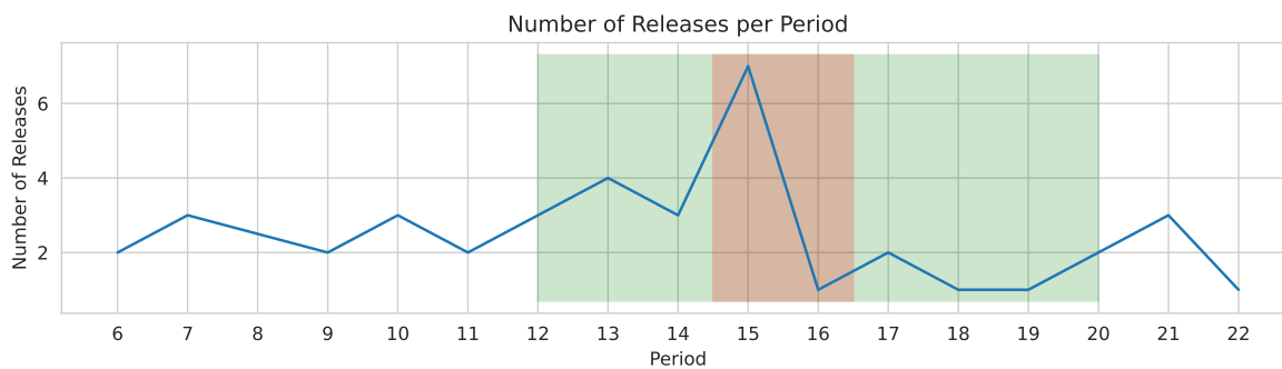
(a) Roslyn
