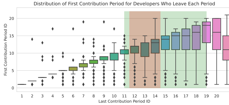
(c) Kubernetes
