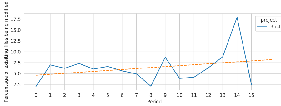
(b) Rust
