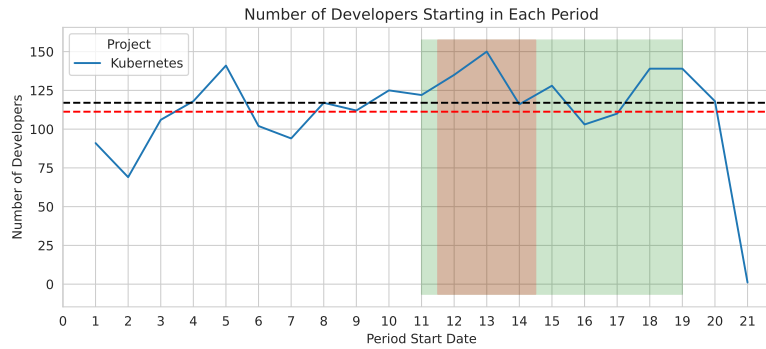
(c) Kubernetes
