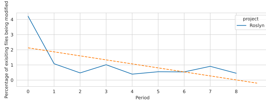
(a) Roslyn
