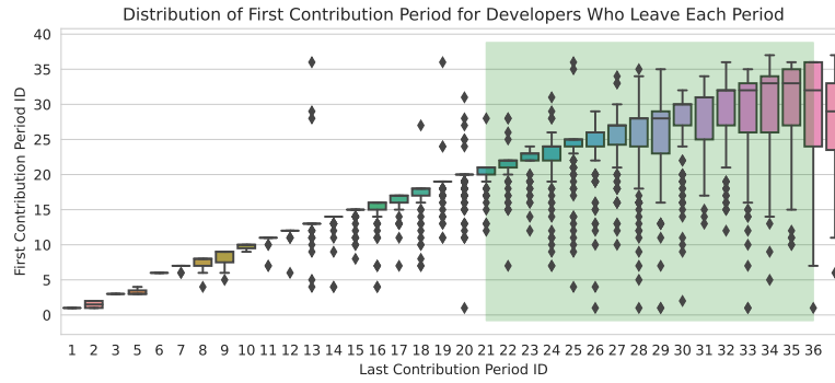
(b) Rust
