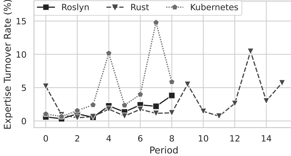
Figure 4.6: Developer expertise turnover rate for the studied periods over time. We consider the first studied period to be zero in all projects.
