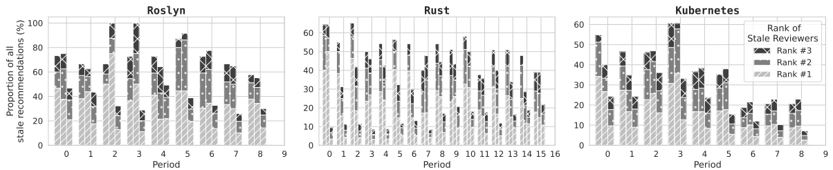
Figure 4.7: The share of top-3 reviewers’ recommendations of all stale recommendations for cHRev (leftmost bar), Sofia (middle bar), and WLRRec (right bar) for studied quarterly periods with reviewer set length of one.
