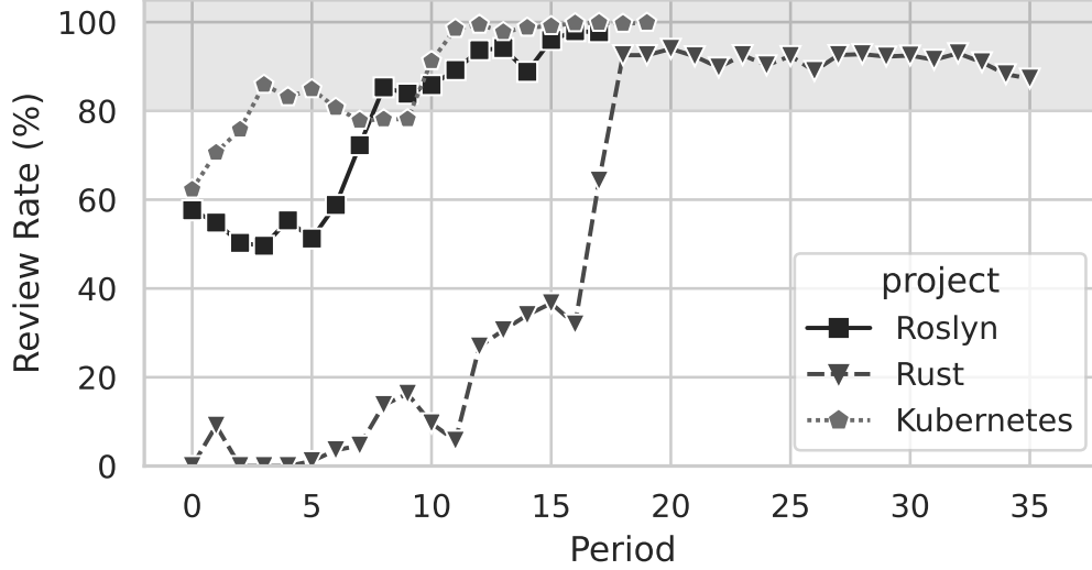
Figure 4.2: Quarterly review rates of Rust, Roslyn and Kubernetes projects.
