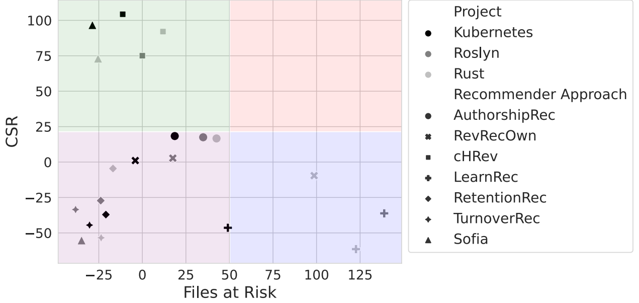
Figure 5.2: Relation analysis of CSR and FaR .
