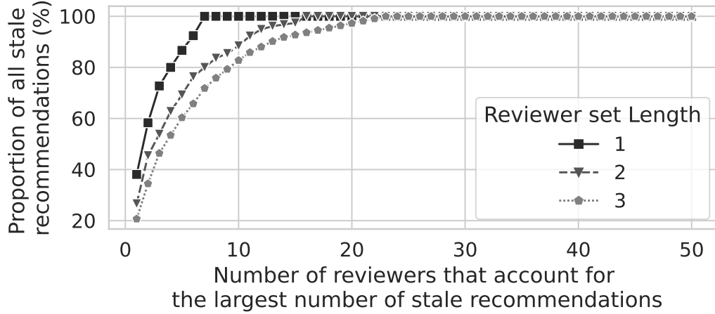
Figure 4.8: Change of top-N reviewers’ share in stale recommendations with value of N when Sofia is applied to Roslyn (reviewer set lengths 1-3).
