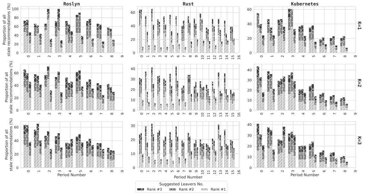
Figure A.3: The top-3 most frequently stale recommendations and their share of all suggested leavers for cHRev (leftmost bar), Sofia (middle bar), and WLRRec (right bar) for various periods under different conditions
