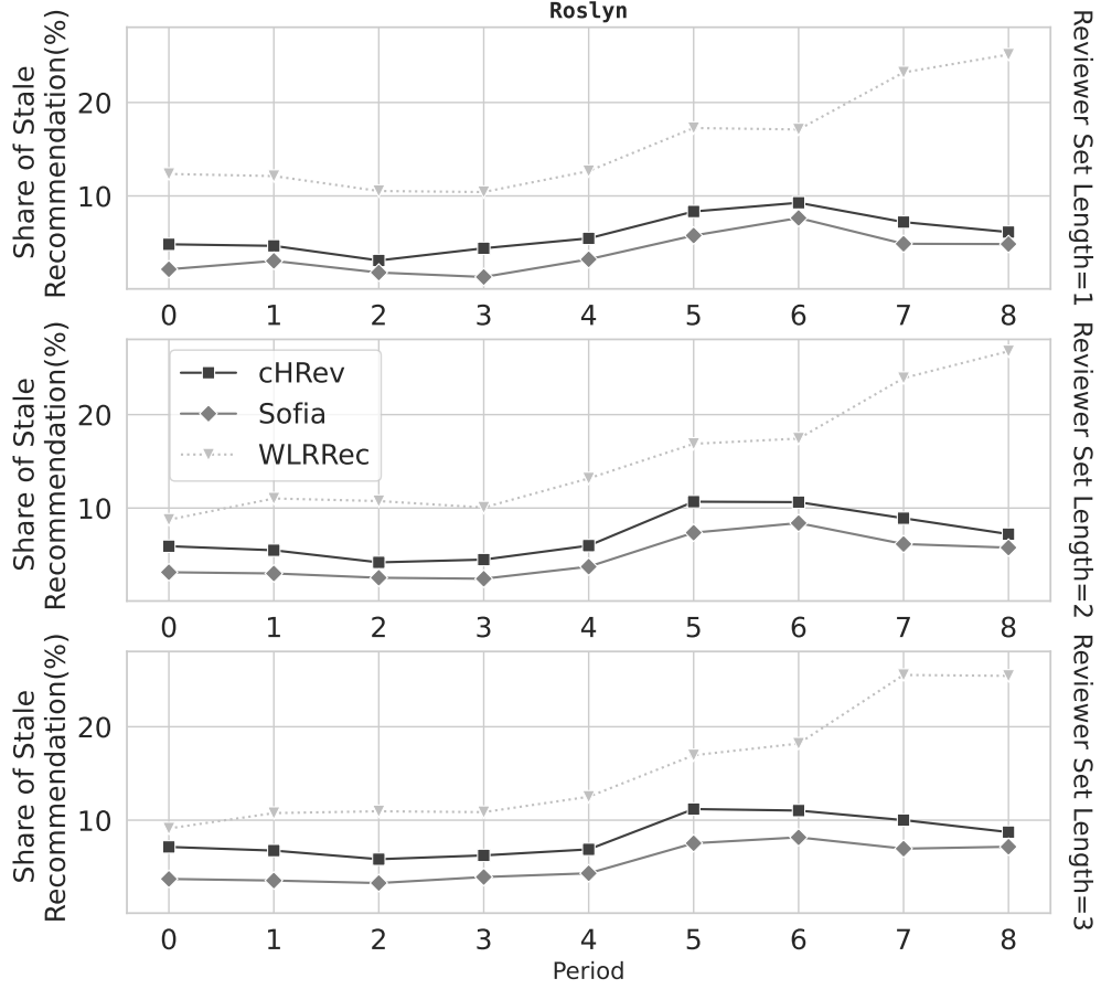
Figure 4.3: Share of stale recommendations over time for studied projects. Rows indicate variations for reviewer set sizes ranging from 1 to 3.
