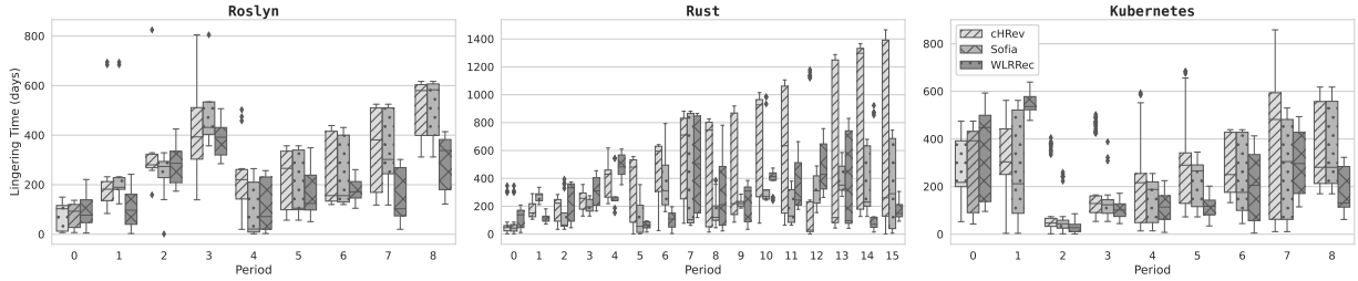
Figure 4.10: The distribution of lingering duration for the top-3 reviewers over quarterly periods.
