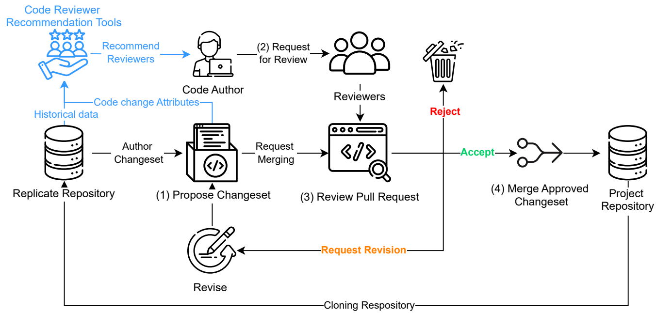
Figure 2.1: The overview of the Modern Code Review (MCR) process (in black) and the role of CRR tools (in blue) in this process.
