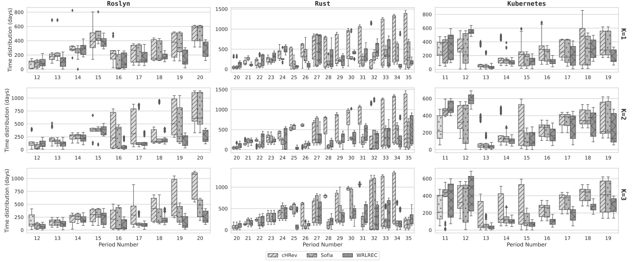
Figure A.5: The distribution of lingering time for the top-3 reviewers over quarterly periods.
