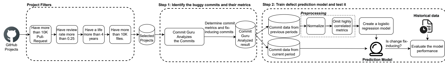
Figure 5.1: The simplified overall architecture of the project selection filters and the defect prediction process.
