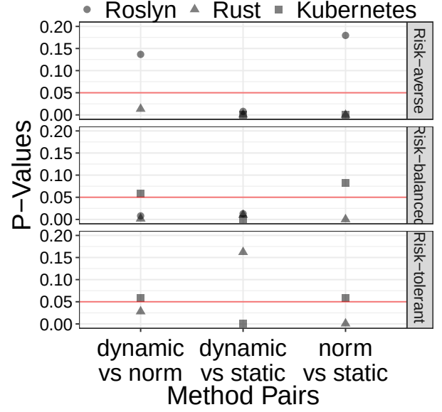
Figure 5.5: Conover Test results.
