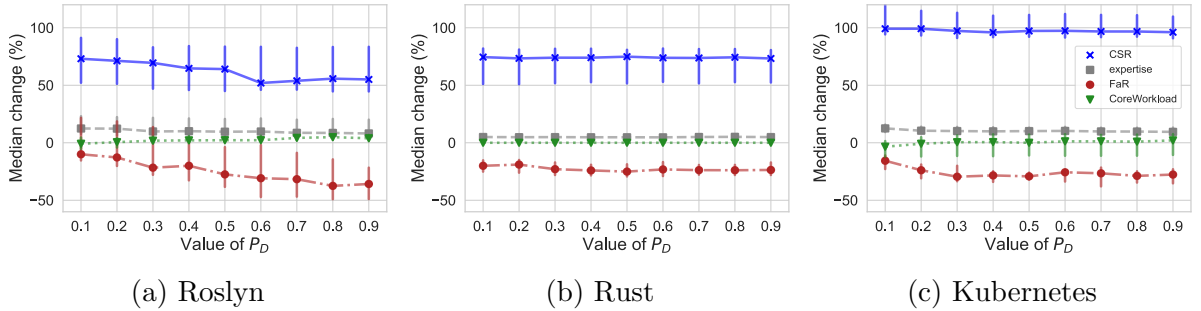
Figure 5.3: The effect of P_D on the performance of CSR for each evaluation metric, on different projects over different quarters.
