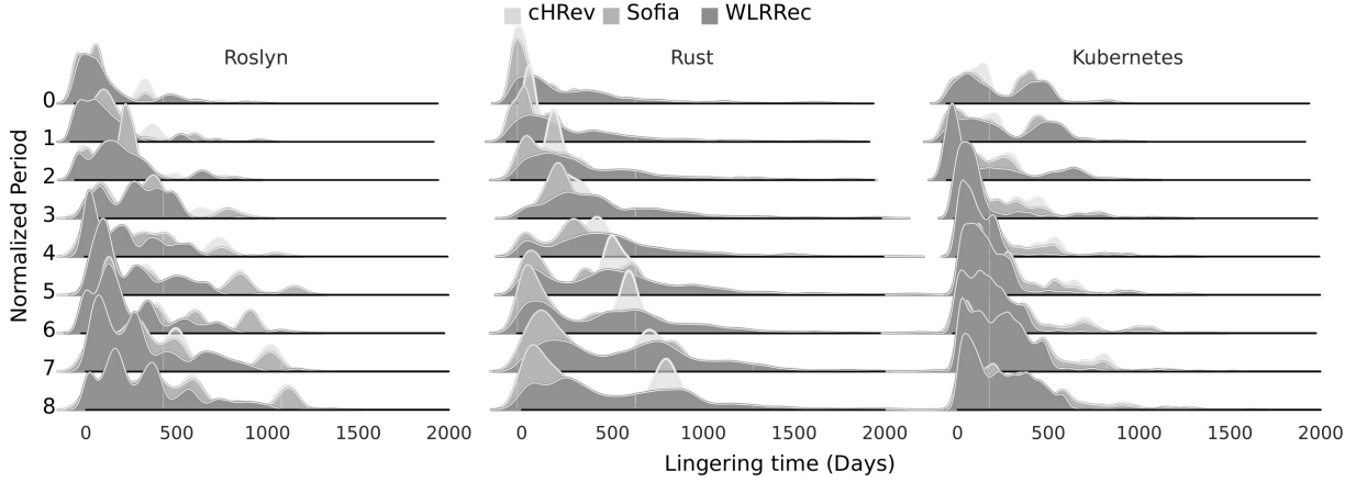
Figure 4.9: The distribution of the duration of stale recommendations (in days) over quarterly periods for the studied projects. Only the first nine periods are drawn.
