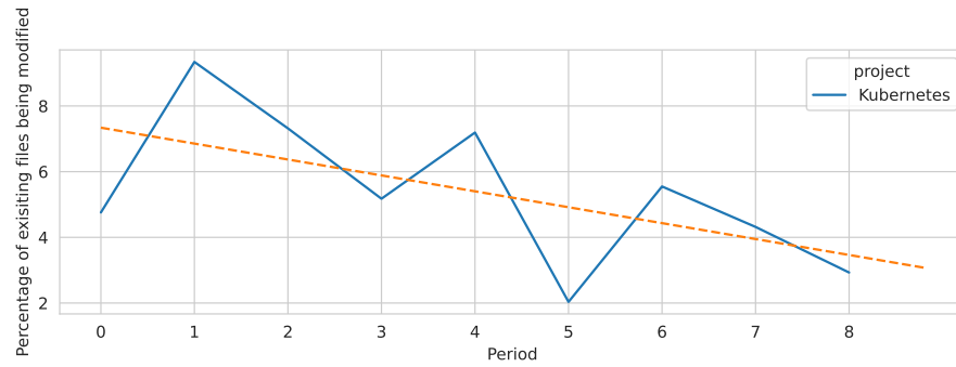
(c) Kubernetes
