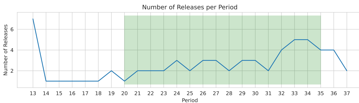
(b) Rust
