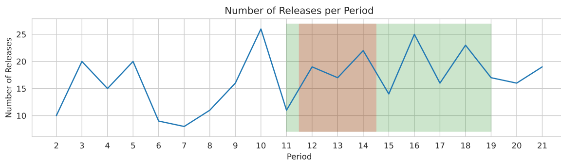
(c) Kubernetes
