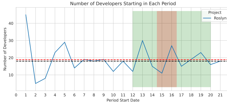
(a) Roslyn
