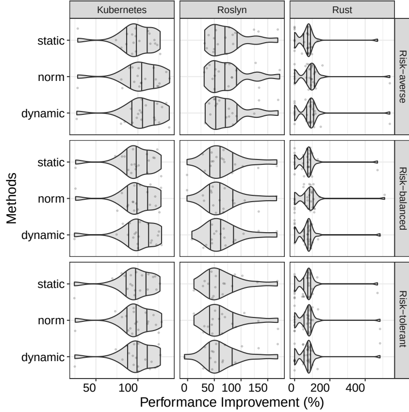
Figure 5.6: The distribution of performance improvement for CSR for different project over time.
