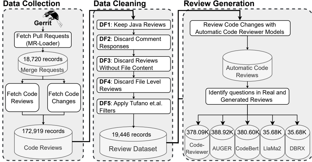
Figure 6.1: The overview of the data preparation procedure.
