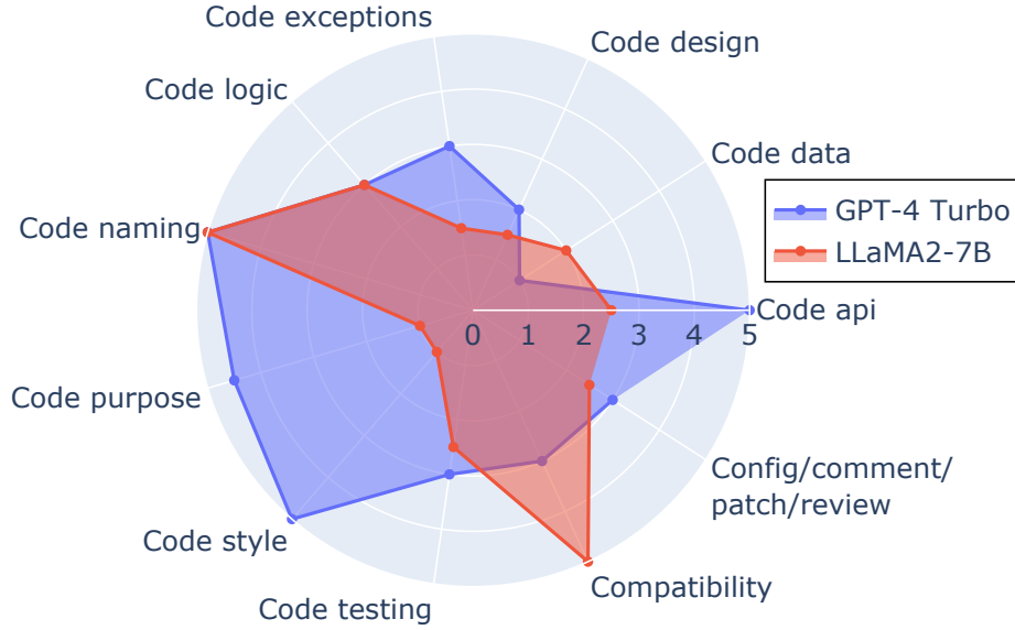
Figure 6.2: similarity scores (median) of responses of LLM-based RCGs to comment threads.
