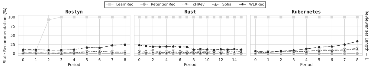
Figure 4.5: The proportions of stale to all recommendations (y-axis). The period numbers are normalized, with zero representing the oldest period.
