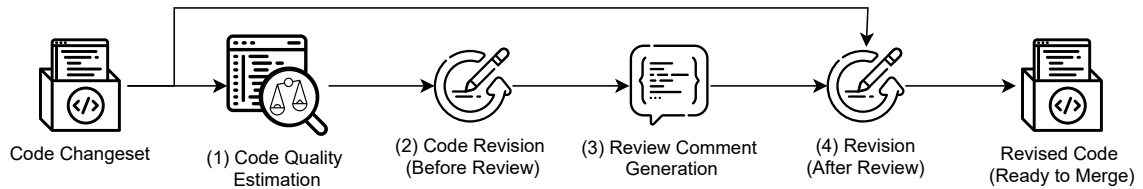
Figure 2.2: The breakdown of the automatic code review process tasks demonstrated in the expected order in an ideal flow.
