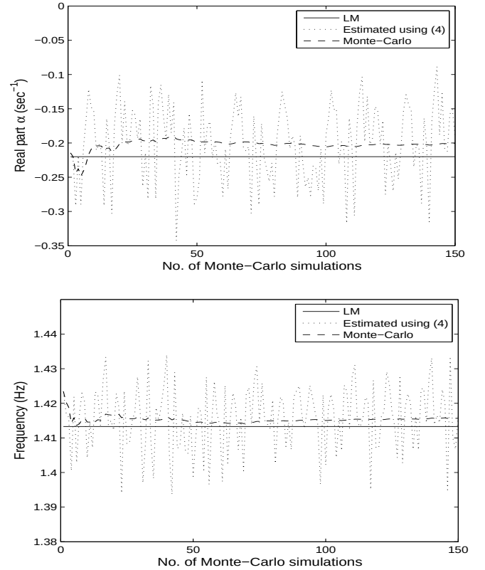
Fig. 11. Real part and frequency of the identified inter-area mode -0.22 \pm j8.83 for the IEEE 14-bus system; ARMA(14,14).
