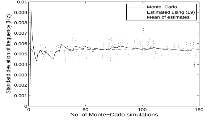
Fig. 7. Standard deviation of the real part and the frequency of the identified inter-area mode -0.1228 \pm j4.7824 for the 2-area benchmark system; AR(15).
