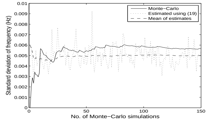
Fig. 8. Standard deviation of the real part and the frequency of the identified inter-area mode -0.1228 \pm j4.7824 for the 2-area benchmark system; ARMA(10,10).
