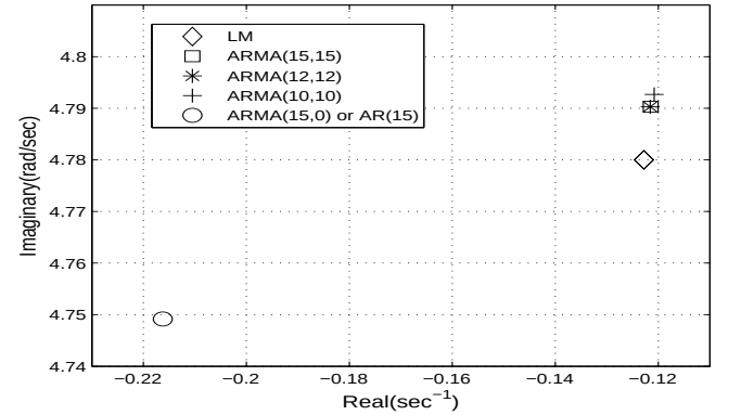
Fig. 4. Mean of the identified inter-area mode -0.1228 \pm j4.7824 for the 2-area benchmark system using a Monte-Carlo method with 150 independent simulations.
