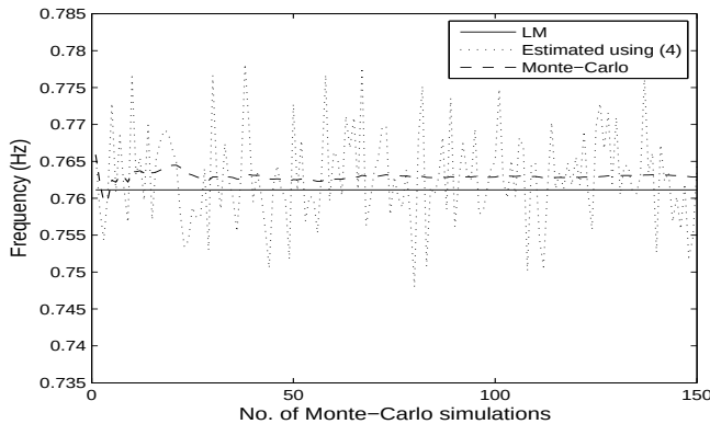
Fig. 6. Real part and frequency of the identified inter-area mode -0.1228 \pm j4.7824 for the 2-area benchmark system; ARMA(10,10).
