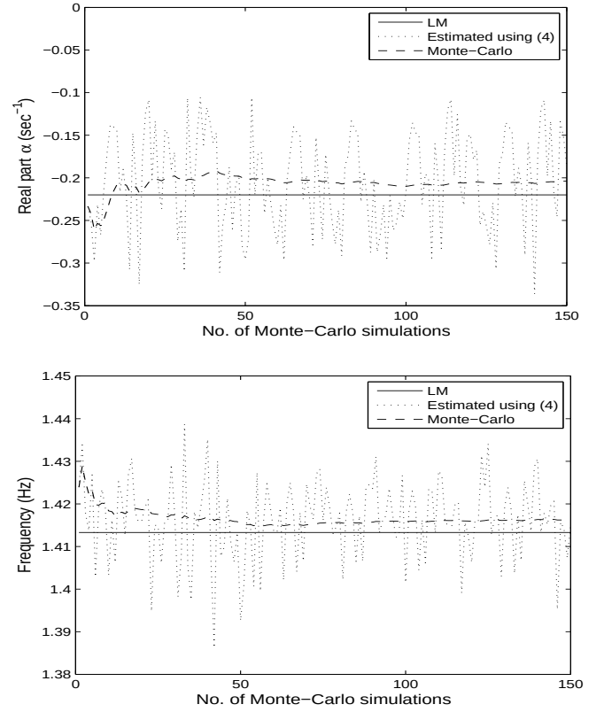
Fig. 10. Real part and frequency of the identified inter-area mode -0.22 \pm j8.83 for the IEEE 14-bus system; ARMA(12,12).
