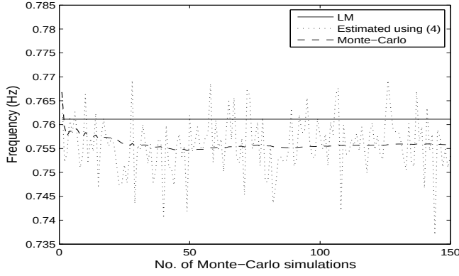
Fig. 5. Real part and frequency of the identified inter-area mode -0.1228 \pm j4.7824 for the 2-area benchmark system; AR(15).
