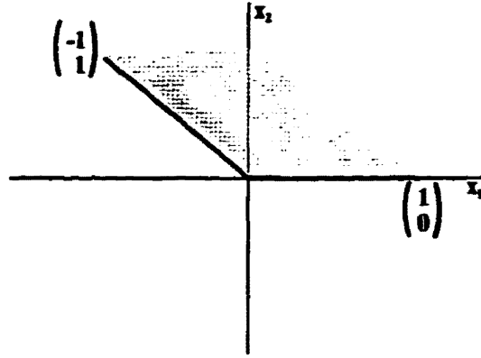
Figure 29: The proper (polyhedral) cone K_1 for Example 23.
