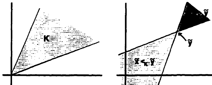
Figure 16: Orderings with respect to a proper cone K in \mathbb{R}^2
