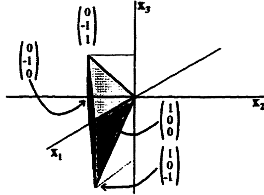
Figure 31: A proper (polyhedral) cone K_1 for Example 24.
