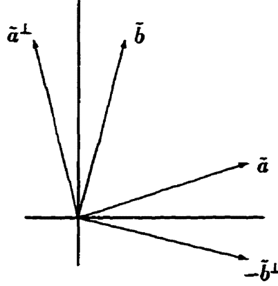
Figure 18: A 2-dimensional cone with extreme rays \tilde{a} and \tilde{b} .
