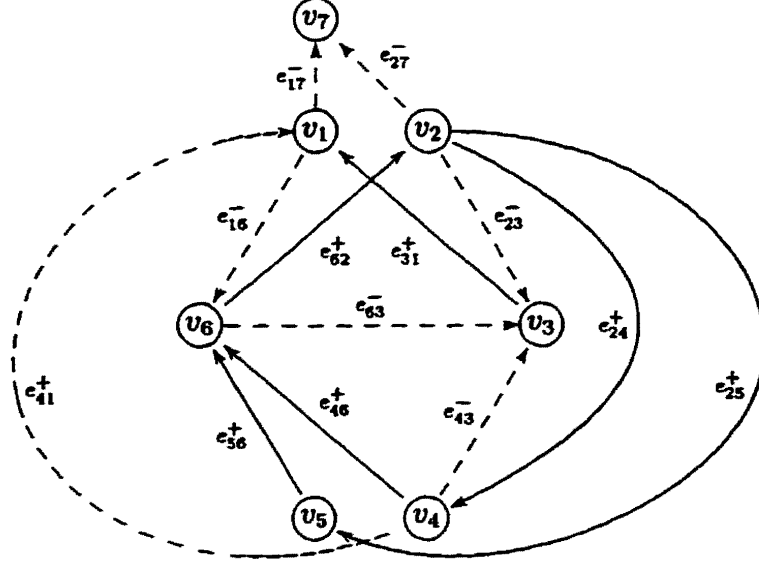
Figure 13: G(\tilde{f}, \Omega) for Example 13
