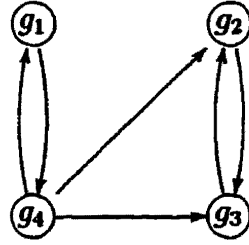
Figure 32: G_{K_1}(\tilde{f}, \mathcal{O}) for Example 24
