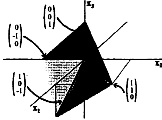
Figure 33: A proper (polyhedral) cone K_2 for Example 24.
