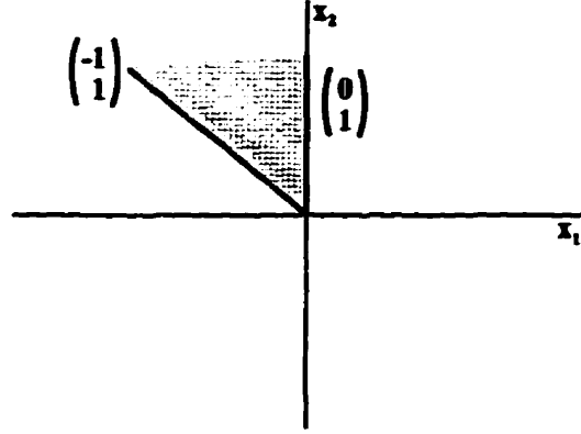
Figure 30: The proper (polyhedral) cone K_2 for Example 23.
