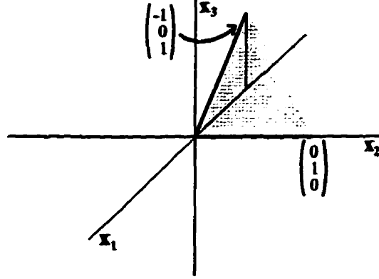
Figure 35: A proper (polyhedral) cone K_3 for Example 24.
