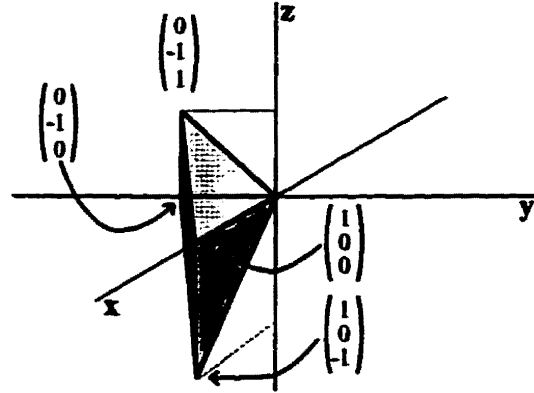
Figure 26: A proper (polyhedral) cone K_2 for Example 22.
