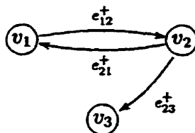
Figure 5: G(\tilde{f}, \Omega) for Example 6
