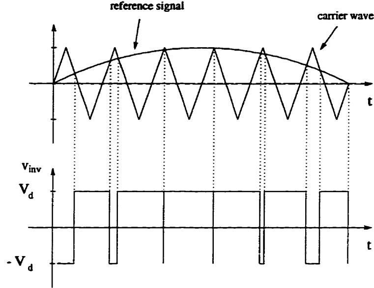
Figure 5.5: Pulse-Width Modulation.
