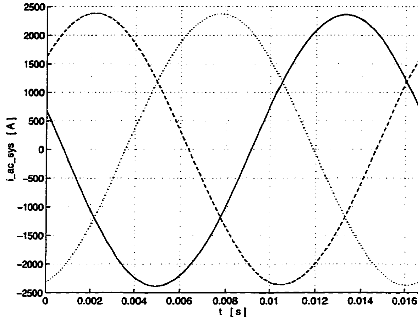
Figure 7.12: AC-system currents with the active filter disabled (— phase a , — phase b , ... phase c ).
