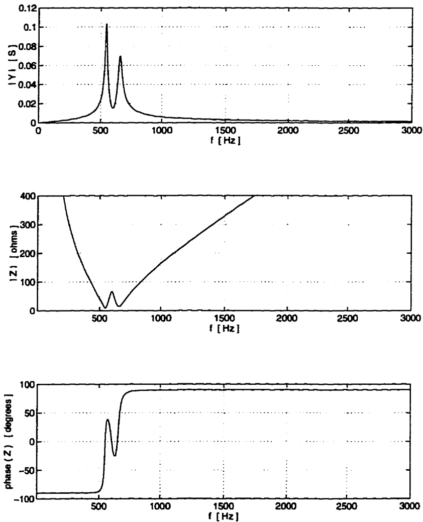
Figure 3.4: Frequency characteristics of a double-tuned filter ( R_1 = 0 \, \Omega , R_2 = 0 \, \Omega , R_3 = 0.444 \, \Omega , L_1 = 41.95 \, \text{mH} , L_2 = 1.44 \, \text{mH} , C_1 = 1.691 \, \mu\text{F} and C_3 = 49.15 \, \mu\text{F} ).
