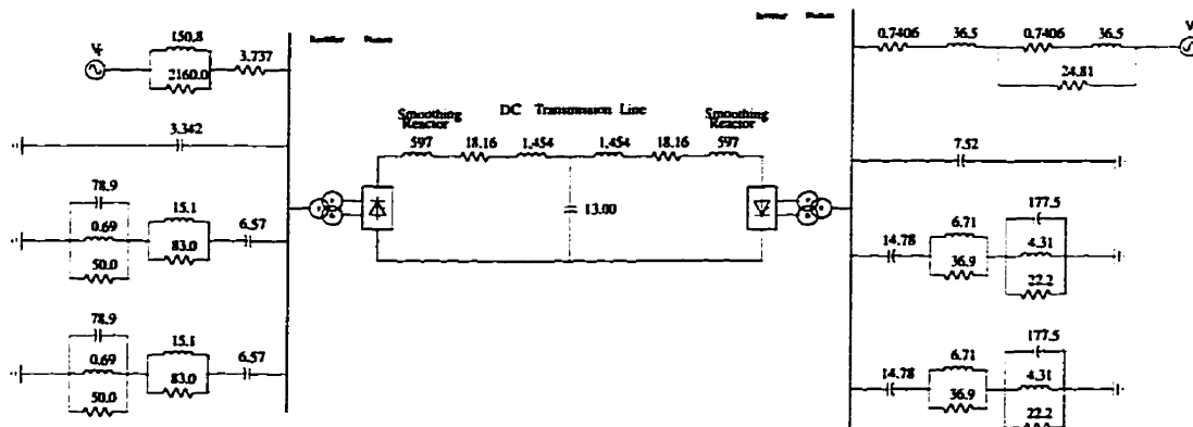
Figure 4.1: The 50-Hz CIGRÉ HVDC benchmark model [ \Omega , mH, \mu F].
