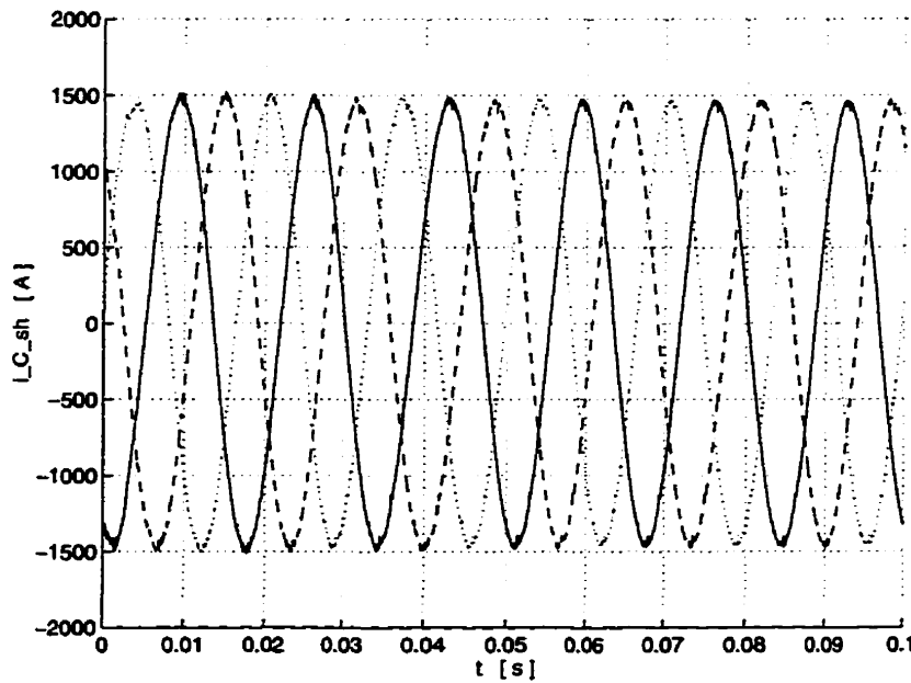
Figure 7.32: Currents through the shunt capacitor banks - Response to a 10%-step in the current order of the HVDC system (— phase a , — phase b , ... phase c ).
