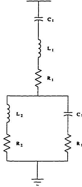
Figure 3.3: Double-tuned filter.
