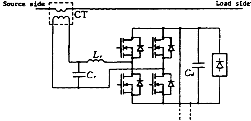
Figure 1.9: Details of one of the active sources of the series active filters (extracted from [20]).
