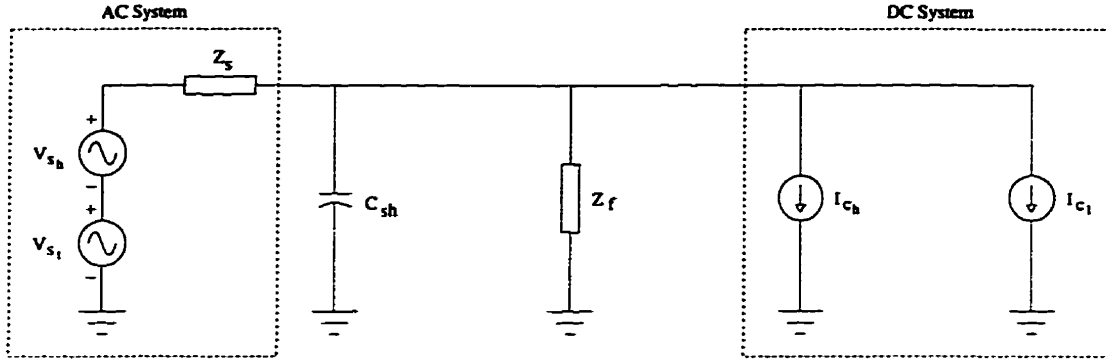
Figure 3.11: Single-phase diagram of an HVDC terminal and connected AC system.
