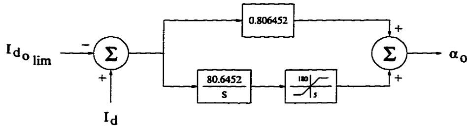
Figure 4.9: Current control.
