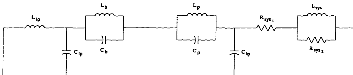
Figure 5.15: Equivalent circuit of the system.
