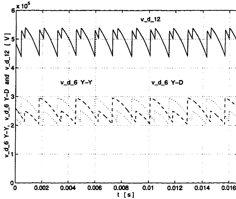
Figure 2.9: DC voltages of an HVDC-converter twelve-pulse bridge (— 12-pulse, --- 6-pulse Y-Y, ... 6-pulse Y- \Delta ).
