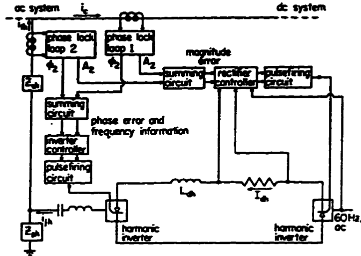
Figure 1.5: Control scheme of the capacitor-commutated active filter (extracted from [17]).
