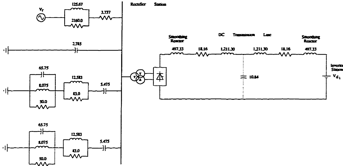
Figure 4.2: The 60-Hz HVDC reference system used in the research [ \Omega , mH, \mu F].
