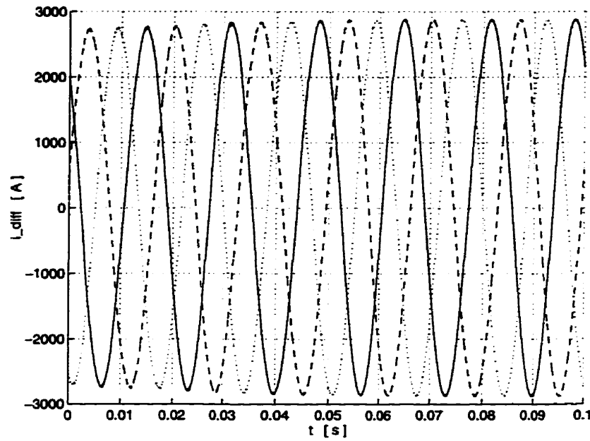
Figure 7.31: HVDC-converter AC line currents which have not been filtered - Response to a 10%-step in the current order of the HVDC system (— phase a , — phase b , ... phase c ).
