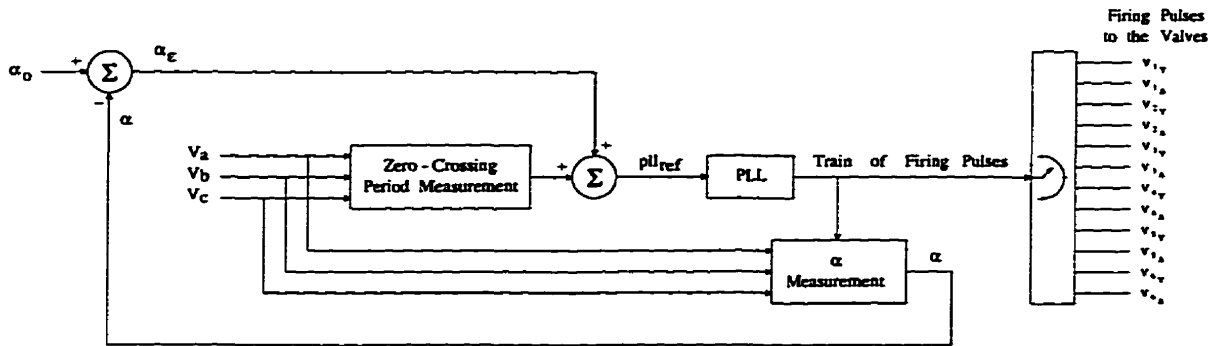
Figure 4.10: Firing control.
