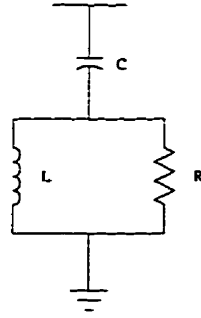
Figure 3.5: Second-Order High-Pass Filter.
