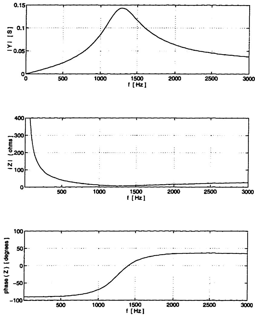
Figure 3.6: Frequency characteristics of a second-order high-pass filter ( R = 46.76\Omega , L = 2.318 mH and C = 6.591 \mu F).
