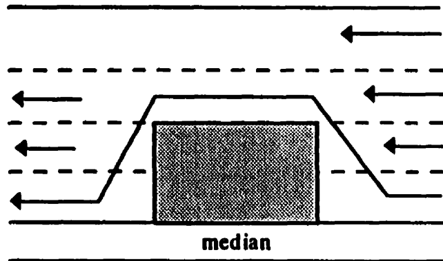
Traffic control plan 8
