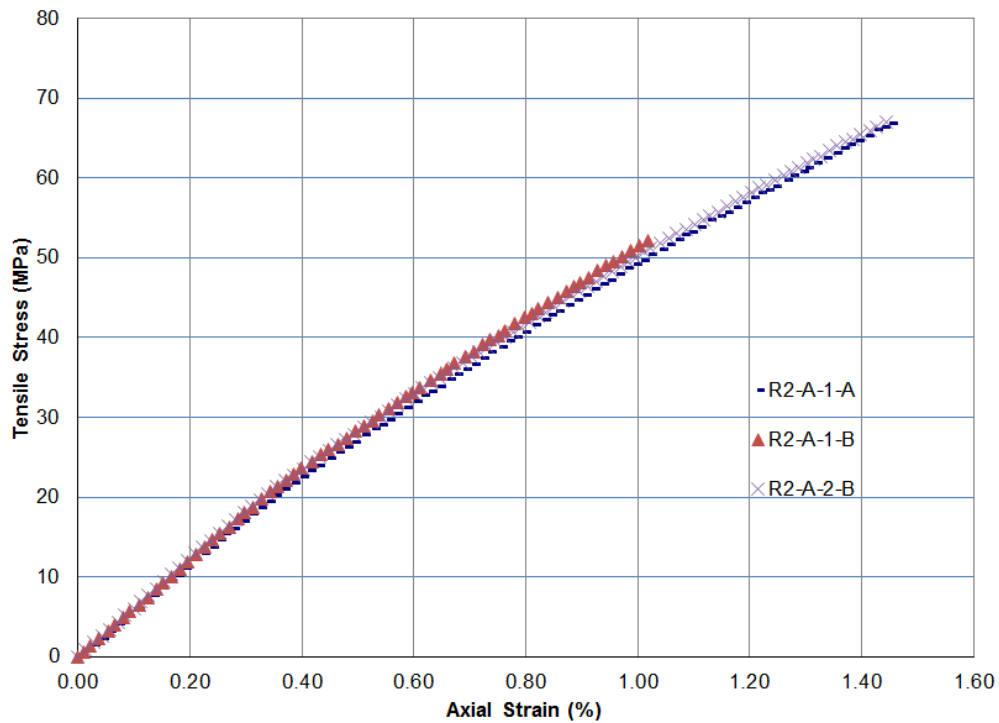
Figure 4.8 - Resin 2 / Liner A - Tensile stress - strain response for all acceptable tests
