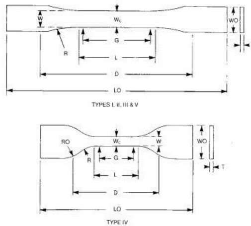
Specimen Dimensions for Thickness, T , mm (in.)
