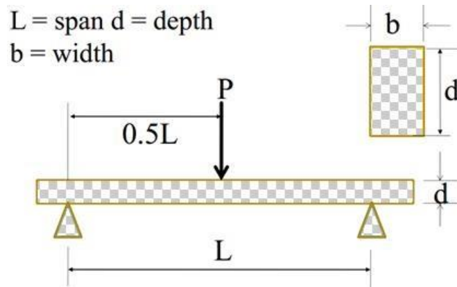
Figure 5.1 - Three-Point loading bending test
