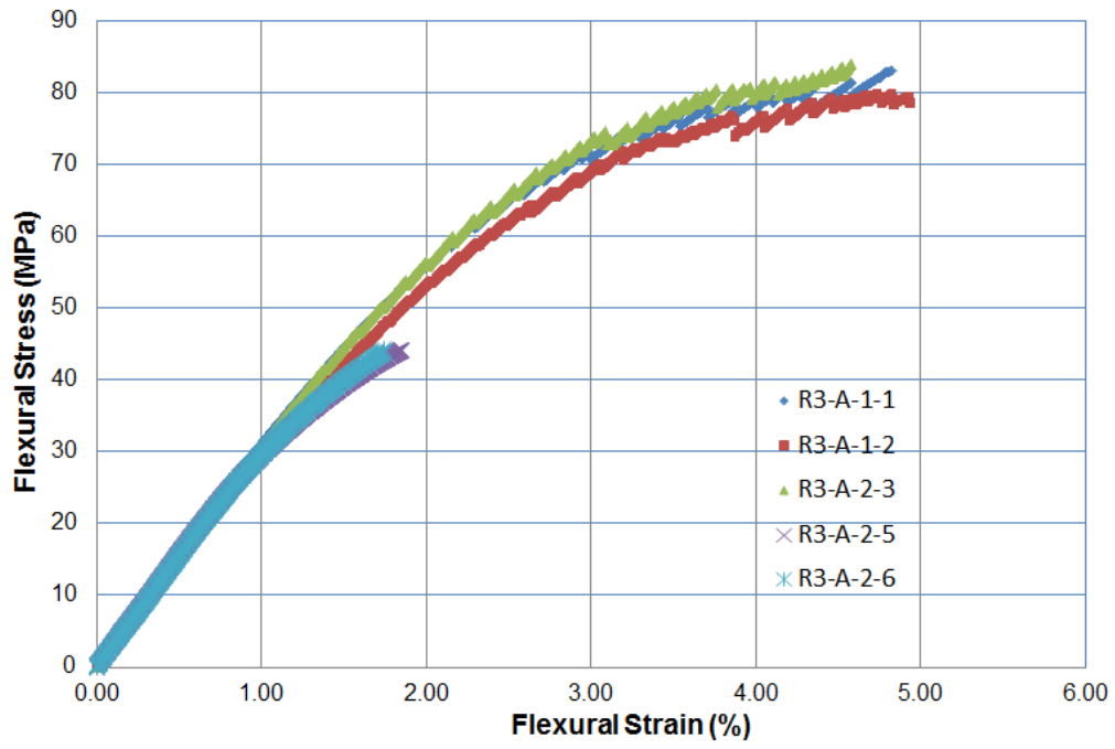
Figure 5.11 - Resin 3 / Liner A - Flexural stress-strain response
