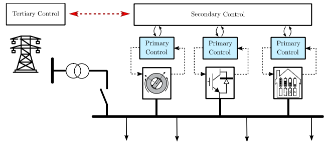
Fig. 11 Illustration of traditional hierarchical MG control.
