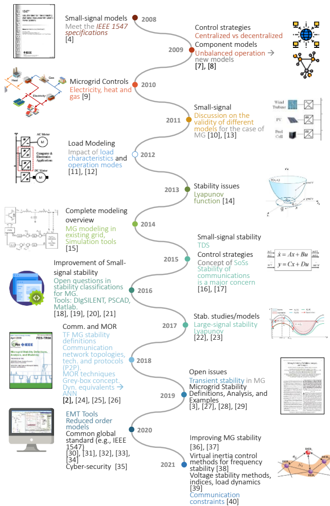
Fig. 1 Evolution of MG modeling topics for stability analysis. Different colors are used to identify the year the highlighted topic first appeared.
