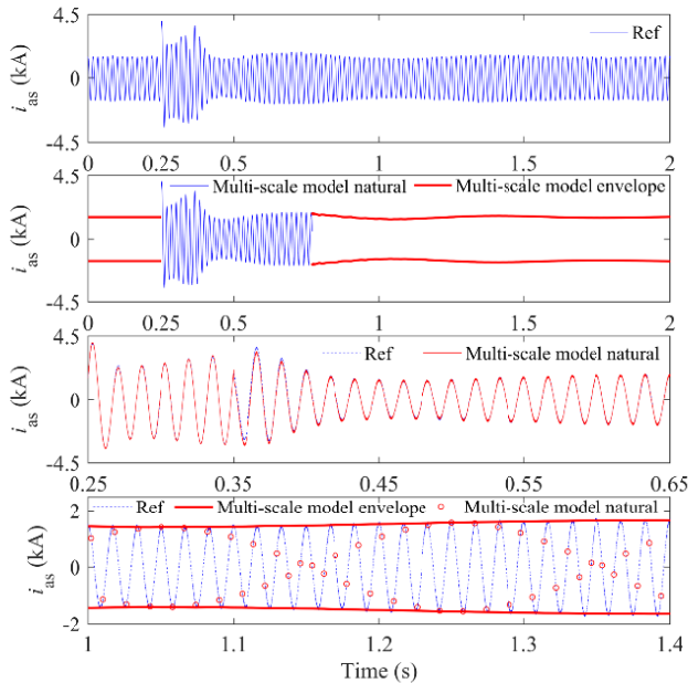
Fig. 13 Phase-a stator current i_{as} of DFIG; (a) natural waveform of the reference solution in PSCAD; (b) natural and envelope waveforms in the multi-scale simulation; solid light: natural waveform; solid bold: envelope; (c) zoomed-in view of i_{as} during electromagnetic transients, dashed: natural waveform of the reference solution in PSCAD/EMTDC; solid: natural waveforms in the multi-scale simulation; (d) zoomed-in view of i_{as} during electromechanical transients, solid light: natural waveform of the reference solution; solid bold: envelope waveforms in the multi-scale simulation; circle: natural waveforms in the multi-scale simulation.
