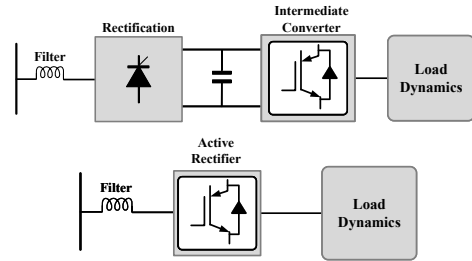
Fig. 9 General structure of a PEC-interfaced load.
