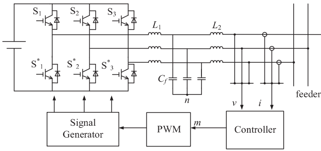
Fig. 4 A two-level, three-phase voltage-sourced inverter [79].
