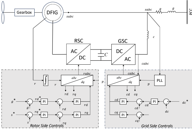
Fig. 6 Modeling of control loops in DFIG wind generator (adapted from [101]).
