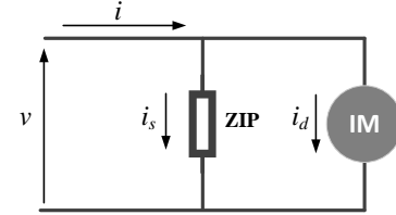
Fig. 8 ZIP+IM composite load model.
