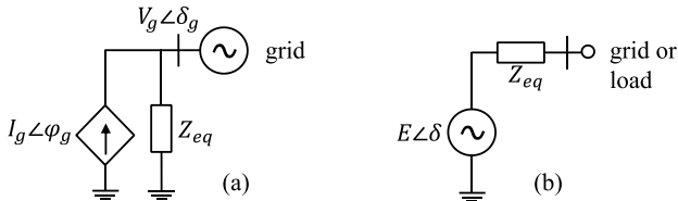
Fig. 5 Concepts of inverter controls: (a) GFL and (b) GFM.
