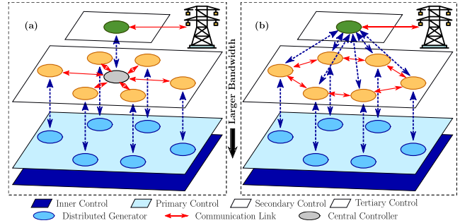
Fig. 12 Architectures for secondary control: (a) centralized and (b) distributed.
