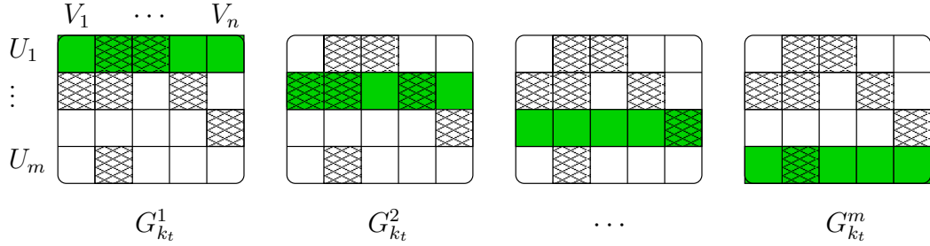
Figure 4.6: m.k_t \bullet G — we only put edges between the m shaded strips.
