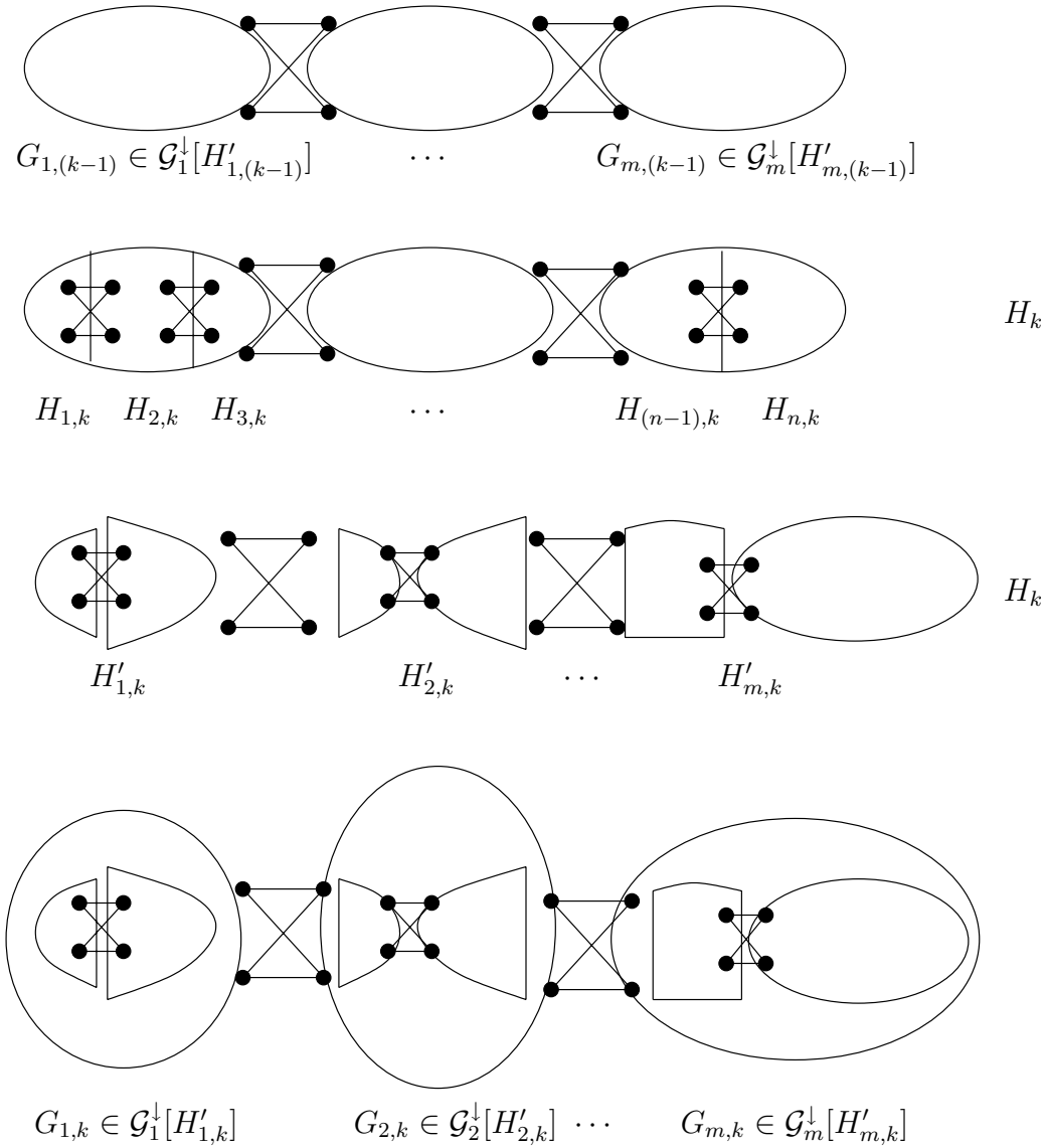
Figure 3.1: We add edges to G_{1,(k-1)} + \cdots + G_{m,(k-1)} to produce a \mathcal{P} -maximal graph H_k . Some of the ind-parts will split into joins of smaller parts; H_k must then have a different (\mathcal{P}_1, \dots, \mathcal{P}_m) -partition from that of H_{k-1} .
