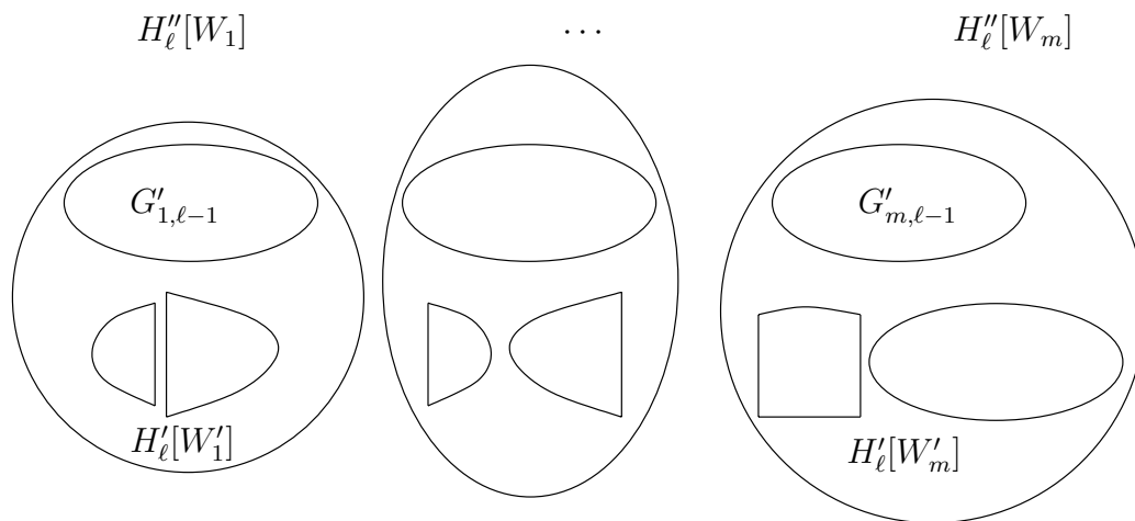
Figure 4.12: Constructing H''_\ell from H'_\ell and H_{\ell-1} .
