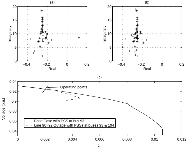
Fig. 6. Line 90-92 outage: (a) Some eigenvalues with PSS at bus 93; (b) eigenvalues with PSS's at bus 93 and 104; (c) P-V curves.
