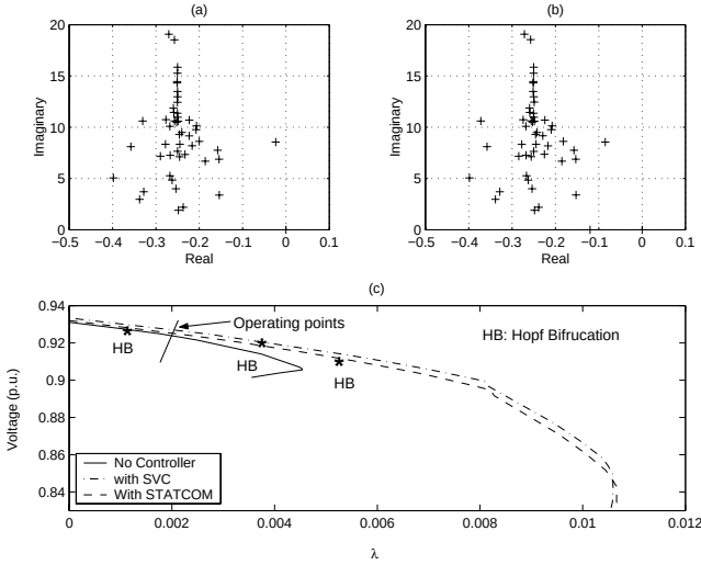
Fig. 9. Line 90-92 outage: (a) Some eigenvalues with SVC; (b) eigenvalues with STATCOM; (c) and P-V curves with SVC and STATCOM.
